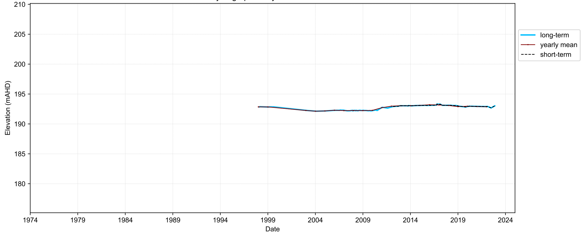
Hydrograph for hydroid: 40151291
