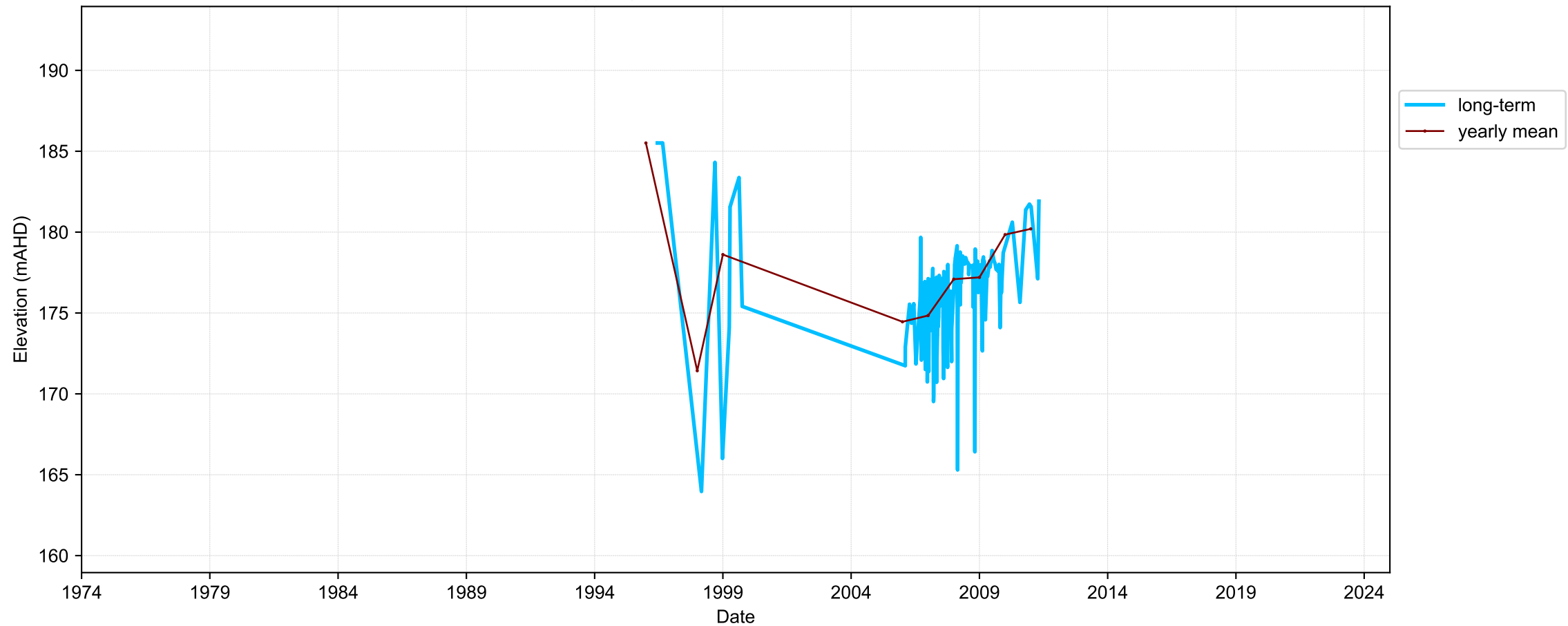
Hydrograph for hydroid: 40144445
