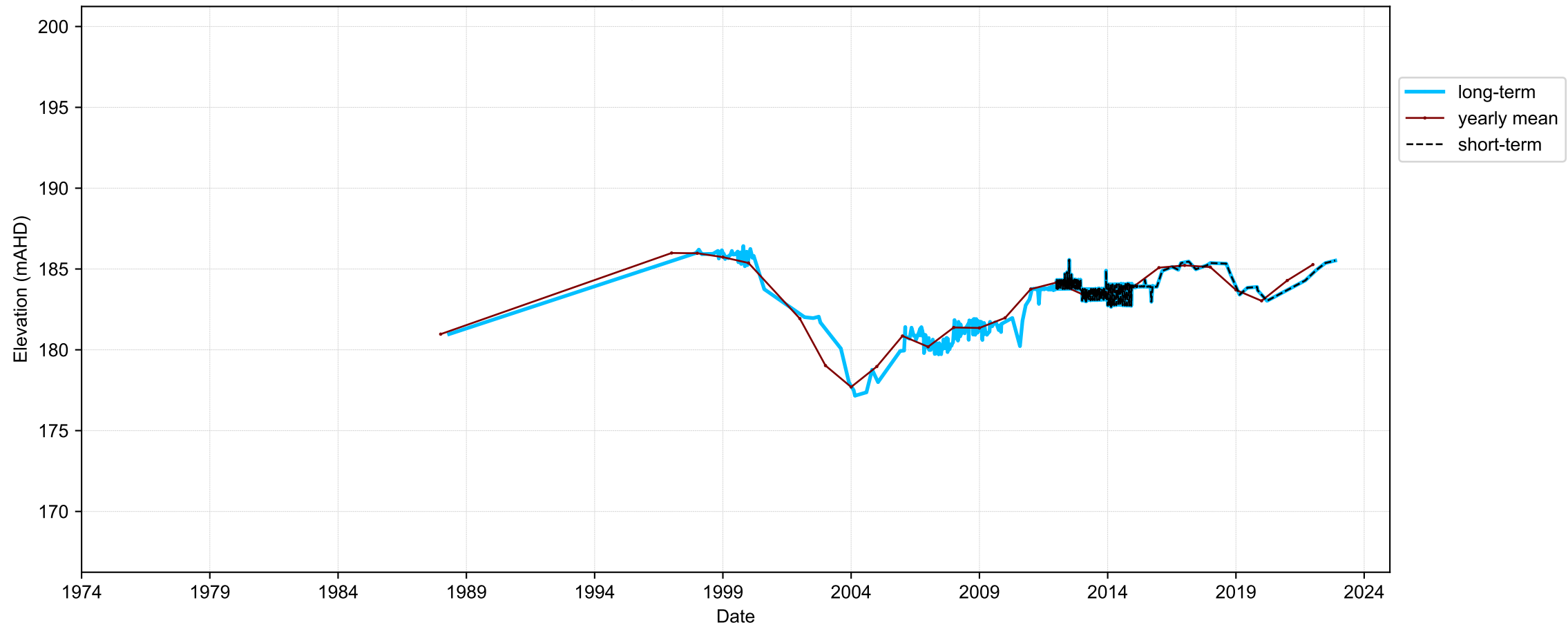
Hydrograph for hydroid: 40133231
