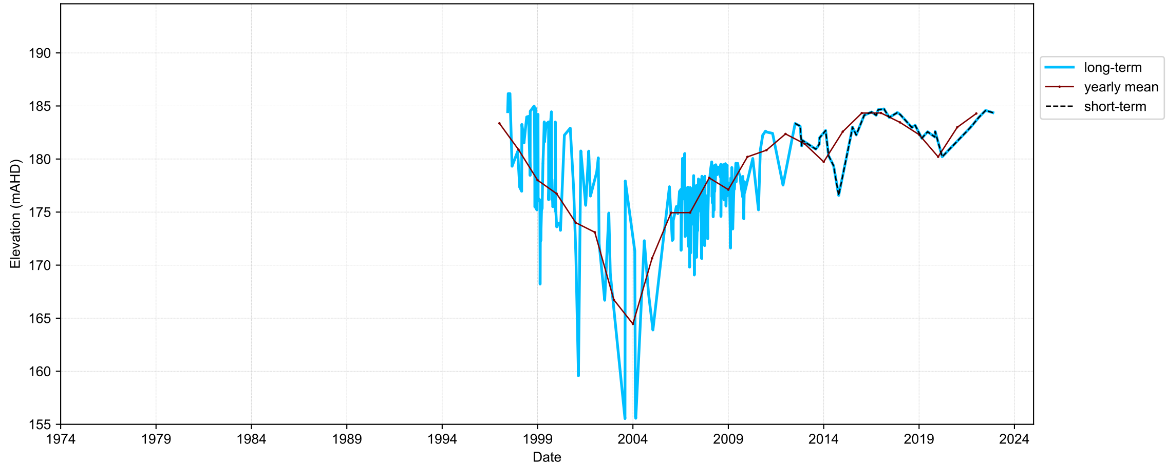
Hydrograph for hydroid: 40135936
