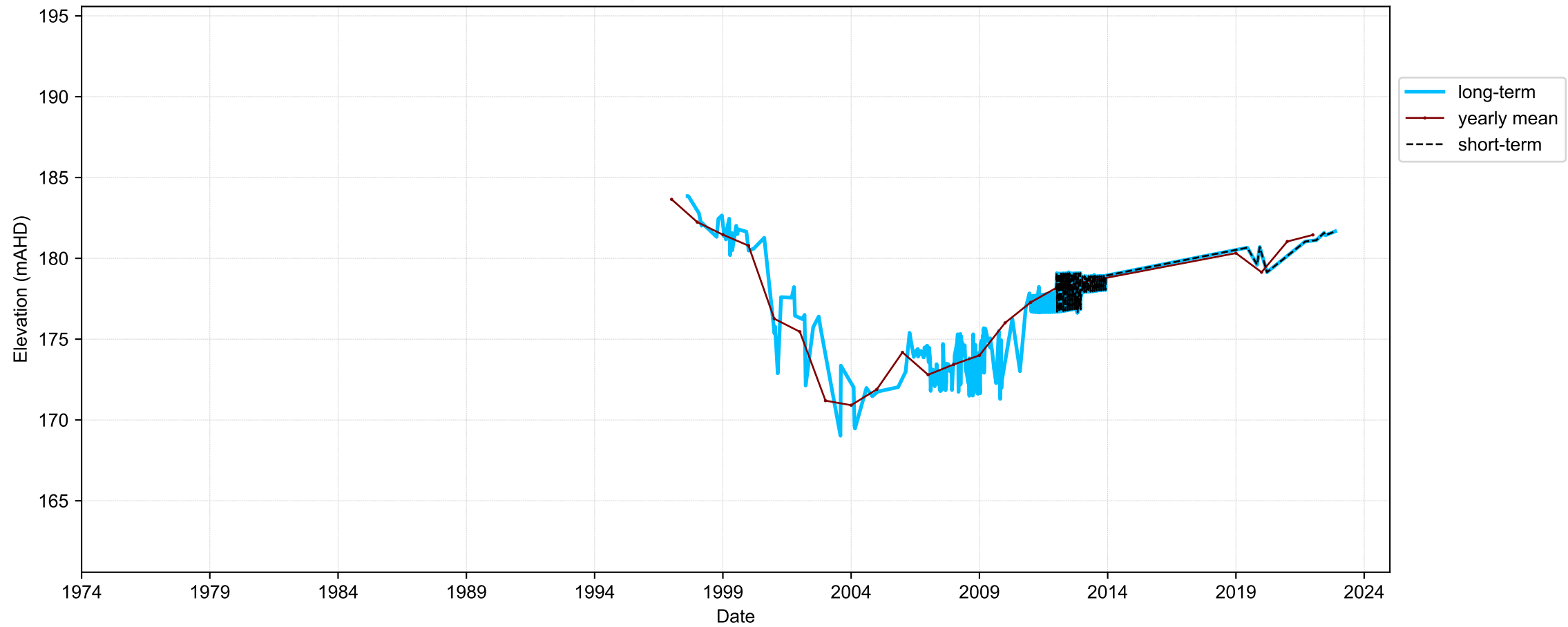
Hydrograph for hydroid: 40135189
