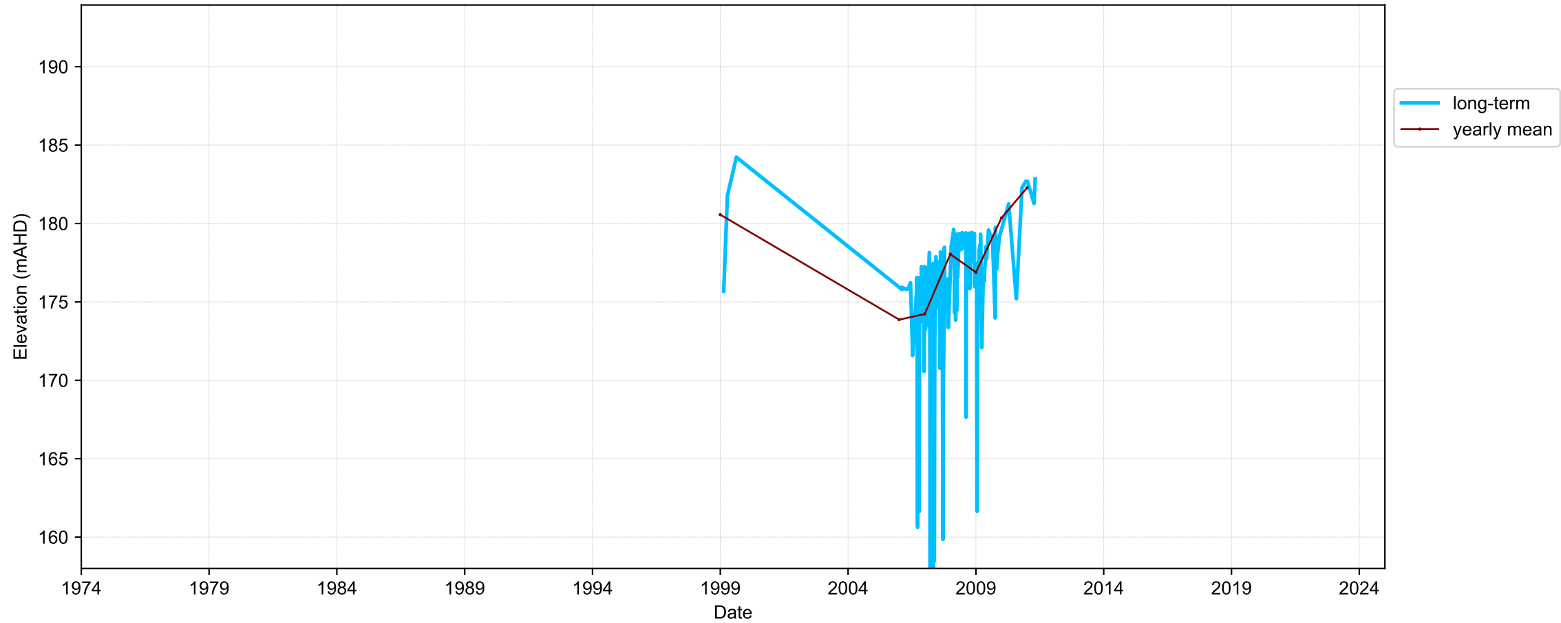
Hydrograph for hydroid: 40151408
