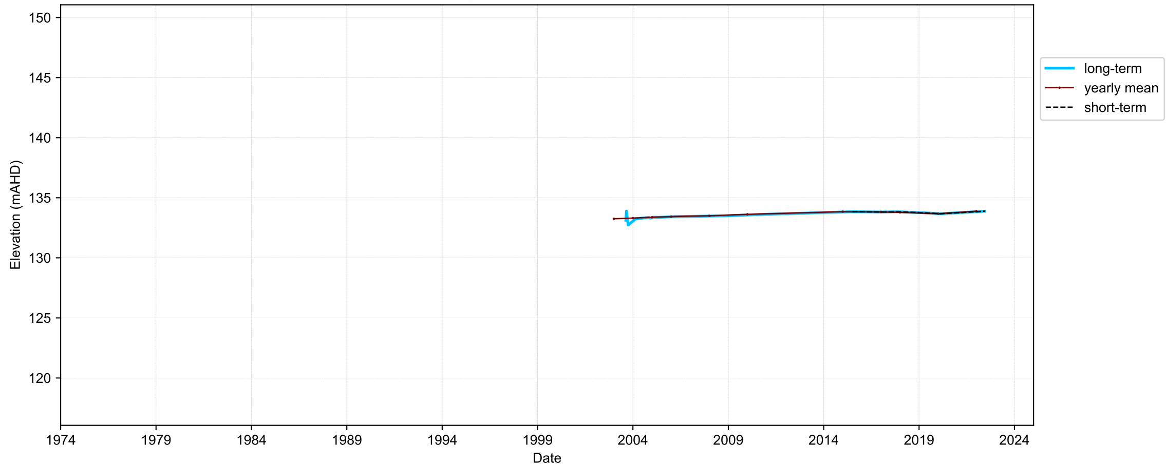
Hydrograph for hydroid: 40150844
