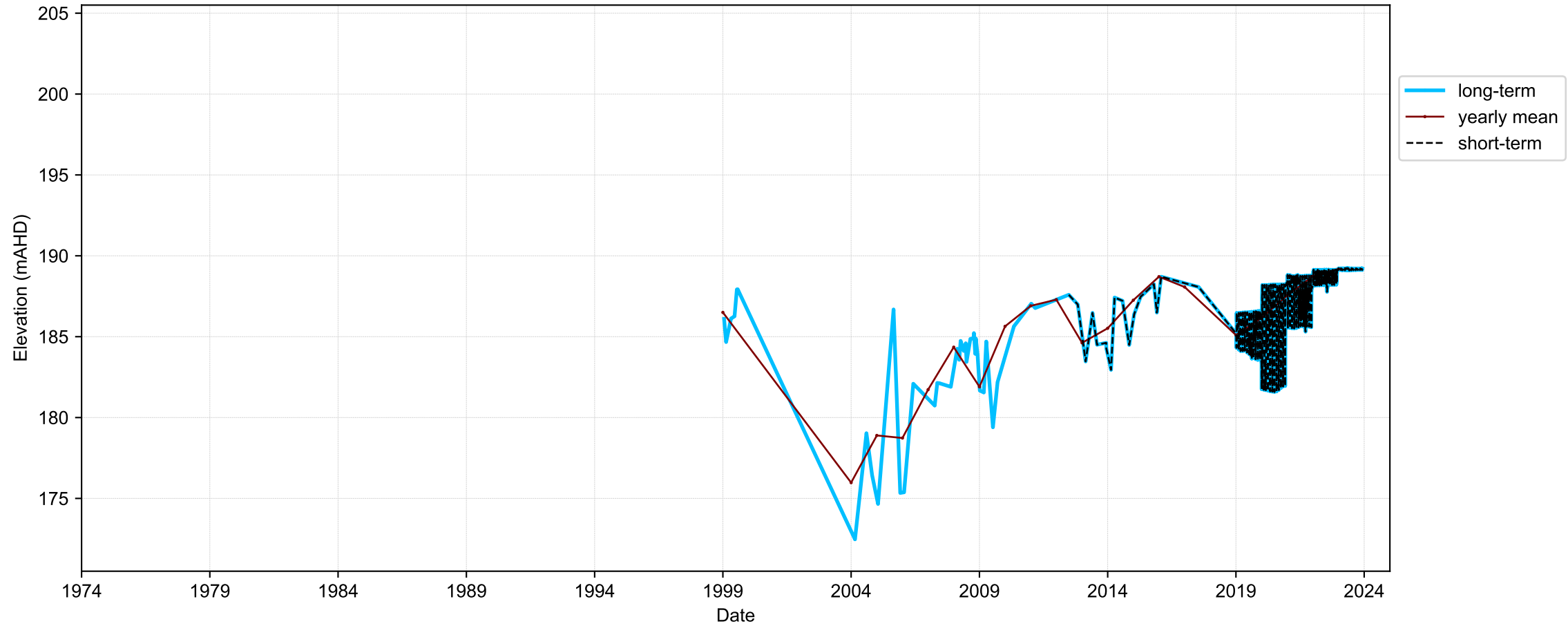
Hydrograph for hydroid: 40133555
