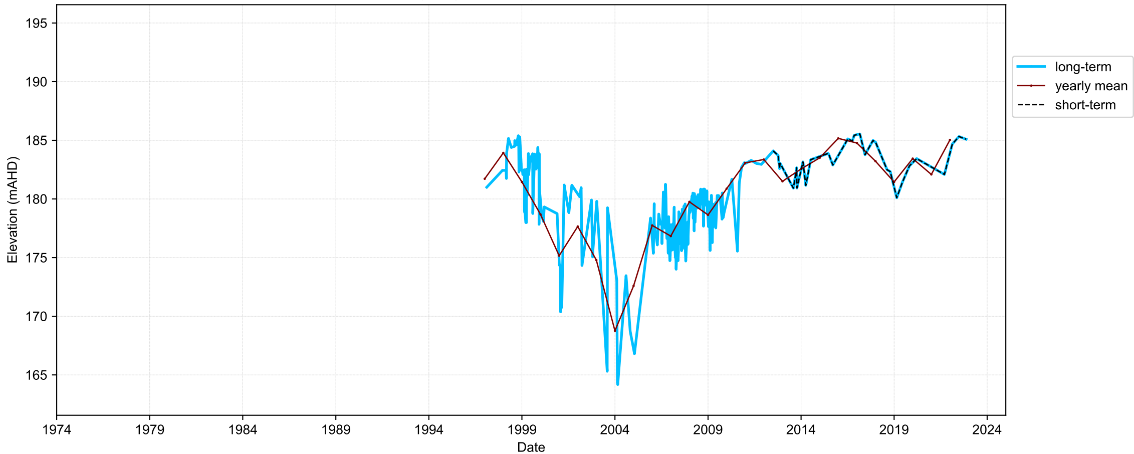
Hydrograph for hydroid: 40139970
