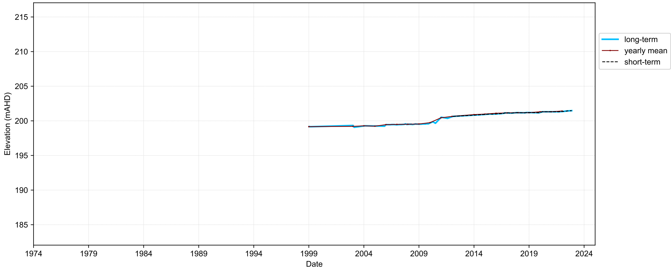
Hydrograph for hydroid: 40141684
