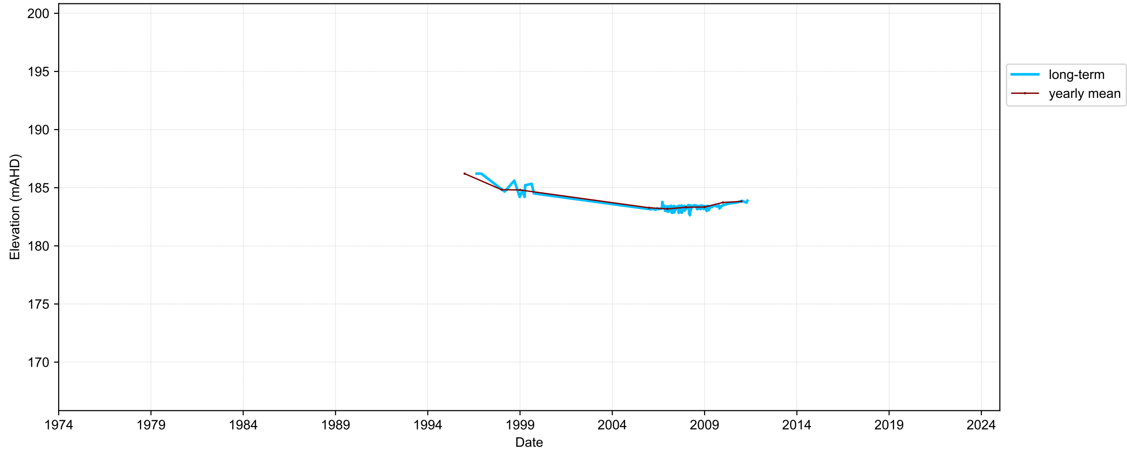
Hydrograph for hydroid: 40151740
