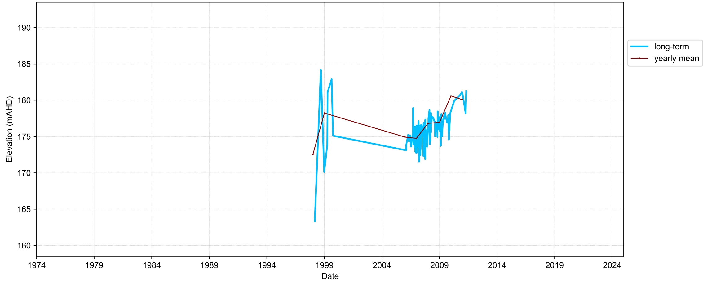
Hydrograph for hydroid: 40132349
