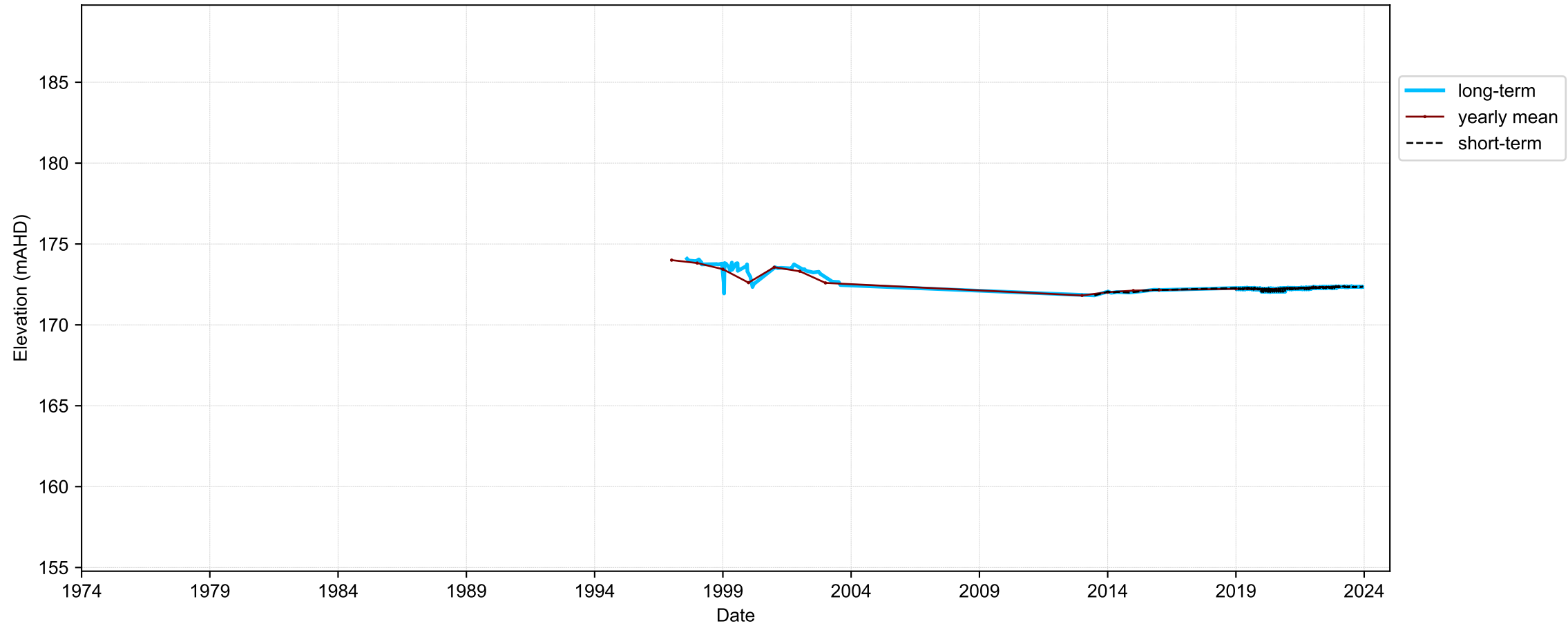
Hydrograph for hydroid: 40147663
