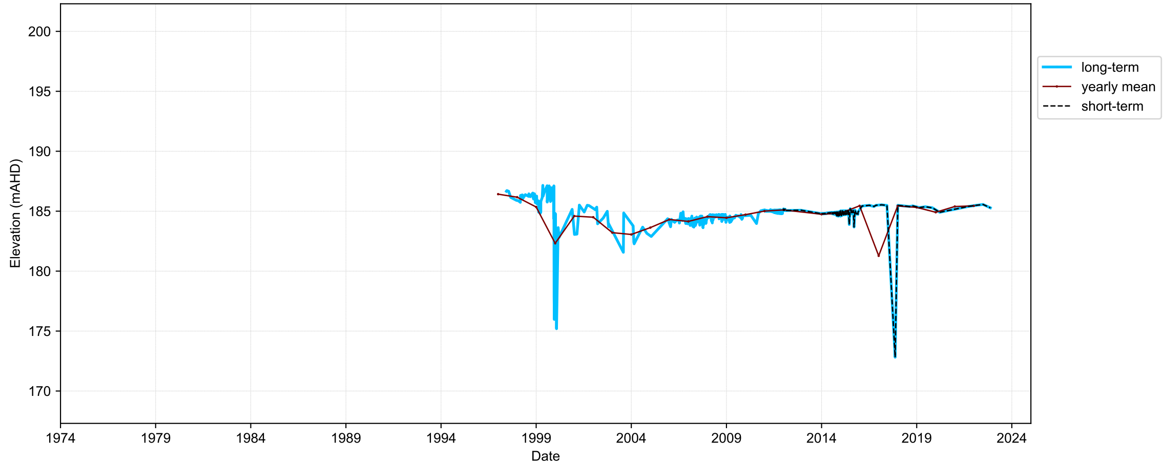
Hydrograph for hydroid: 40136150
