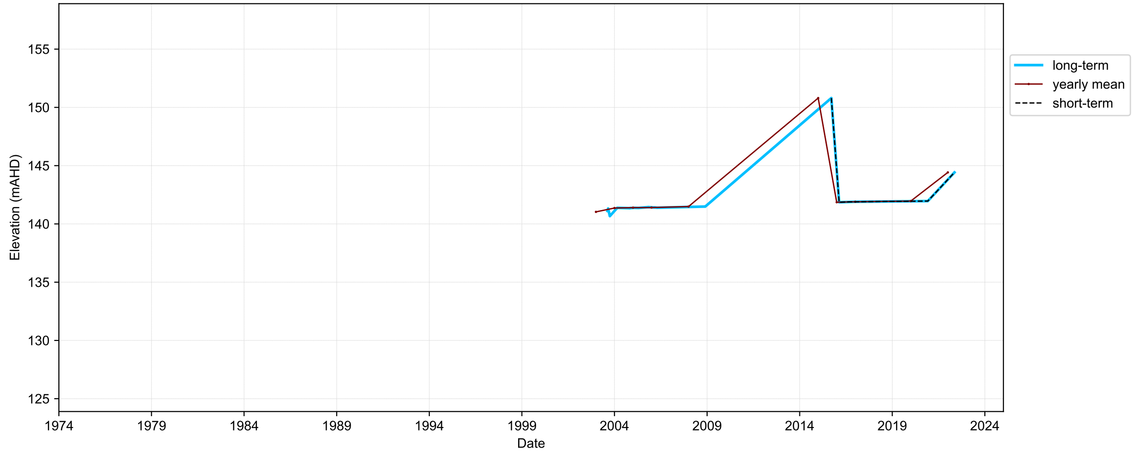
Hydrograph for hydroid: 40137584
