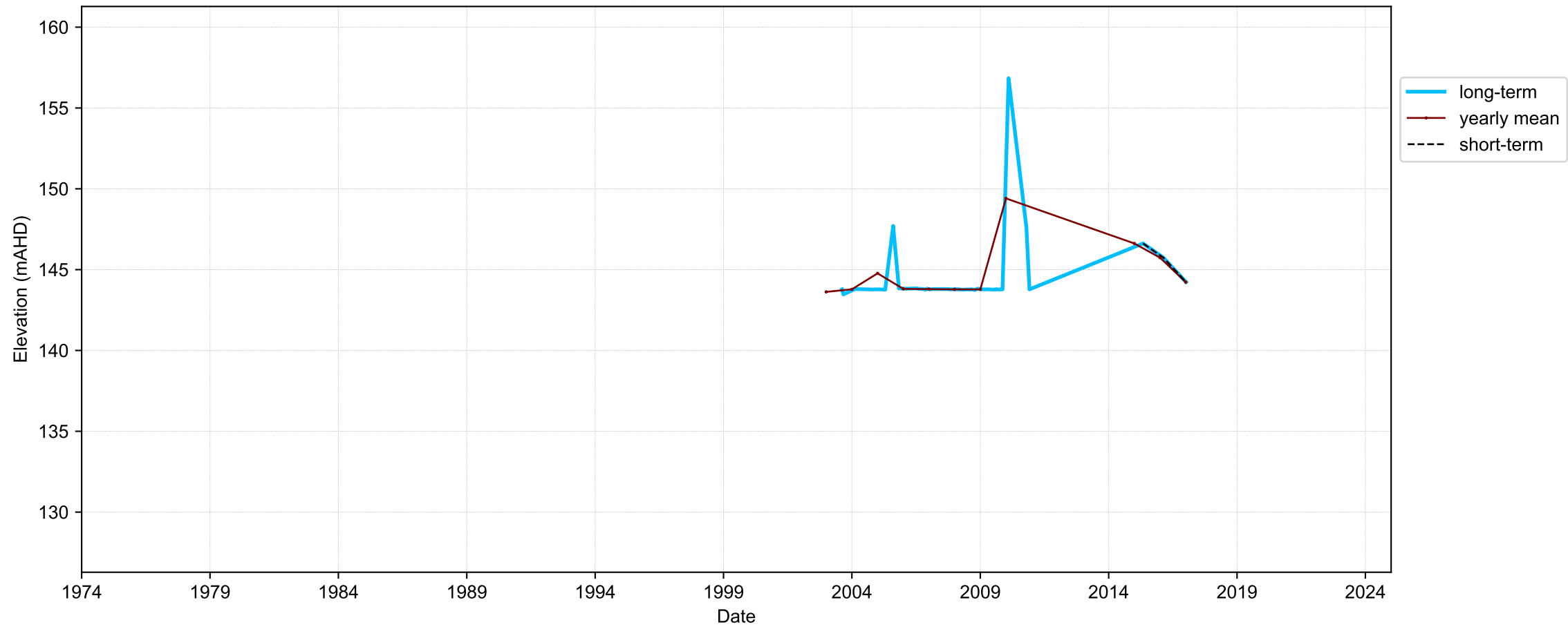
Hydrograph for hydroid: 40143188
