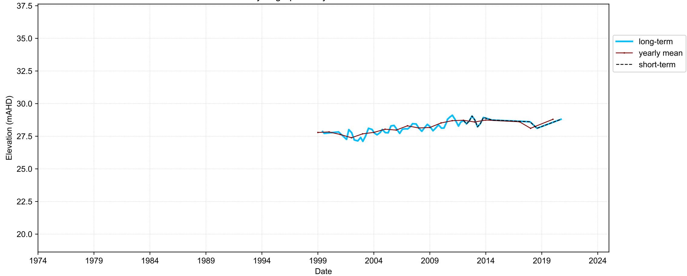
Hydrograph for hydroid: 30156387
