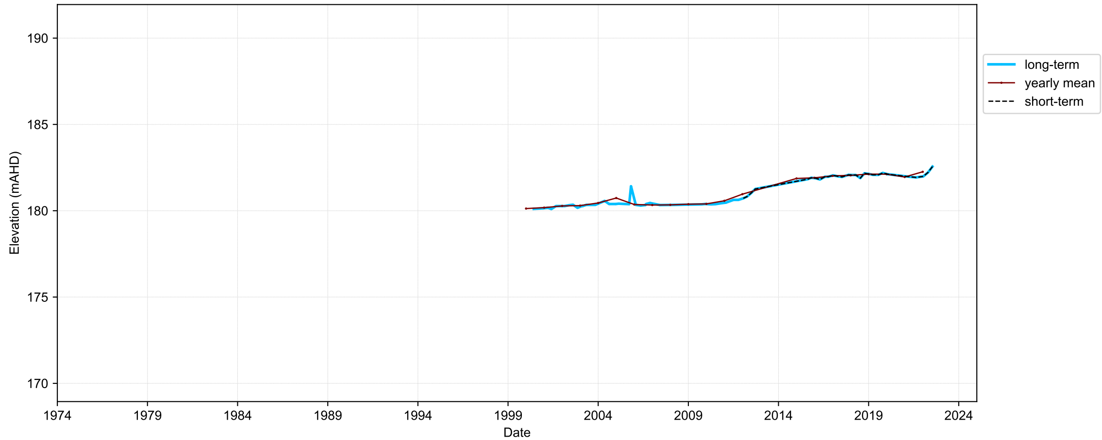
Hydrograph for hydroid: 40148533
