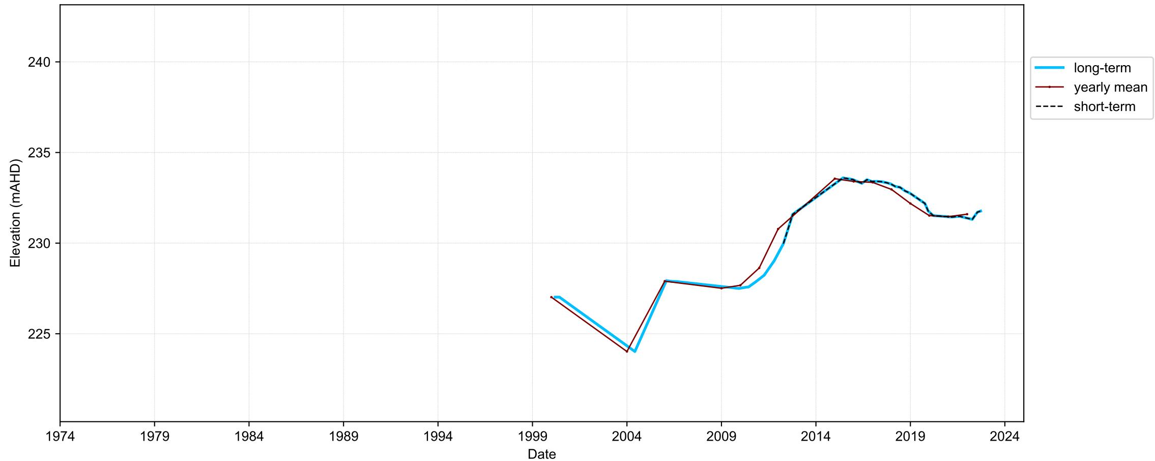
Hydrograph for hydroid: 40065888
