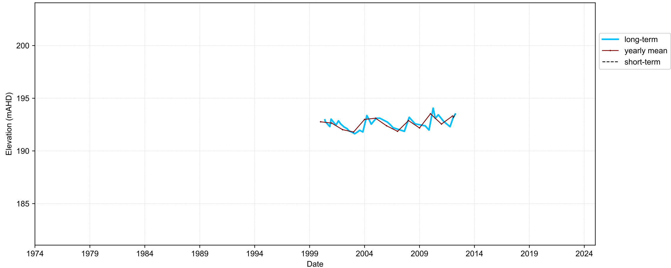
Hydrograph for hydroid: 40139927
