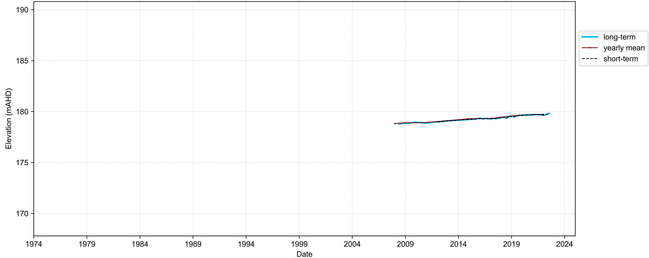
Hydrograph for hydroid: 40132952
