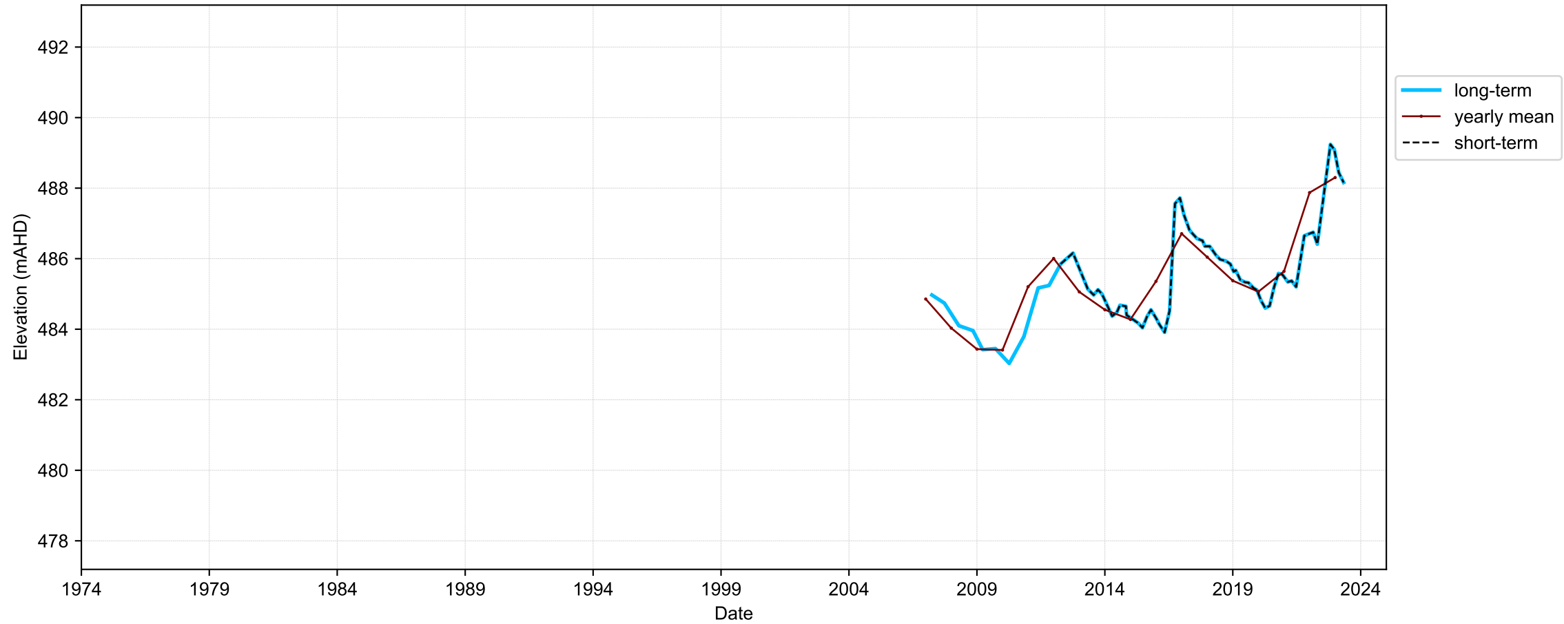
Hydrograph for hydroid: 10079462
