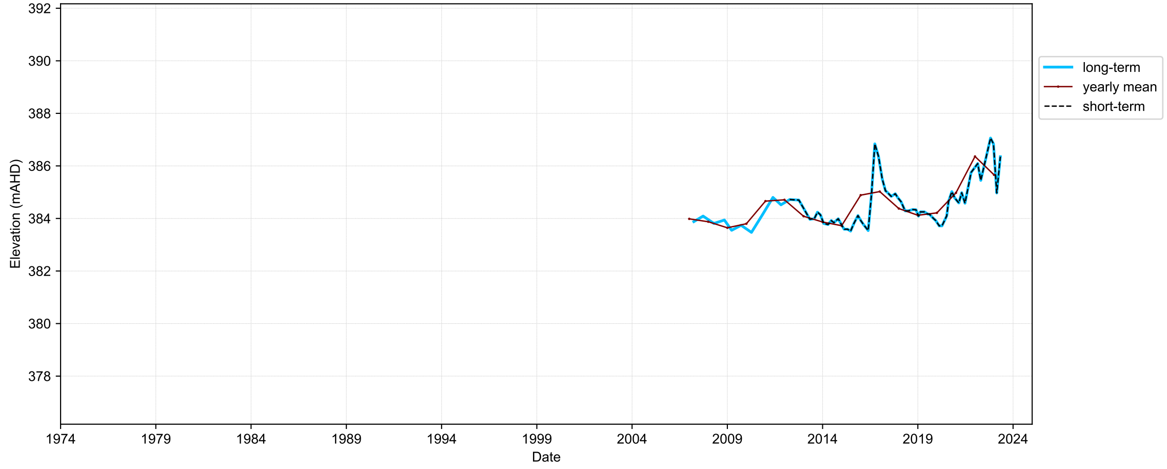
Hydrograph for hydroid: 10070189
