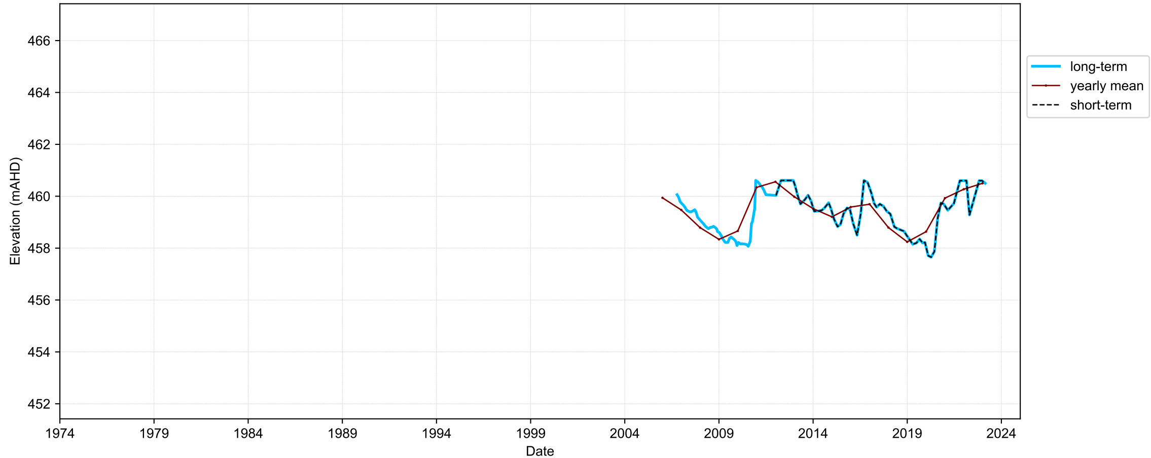
Hydrograph for hydroid: 10095089
