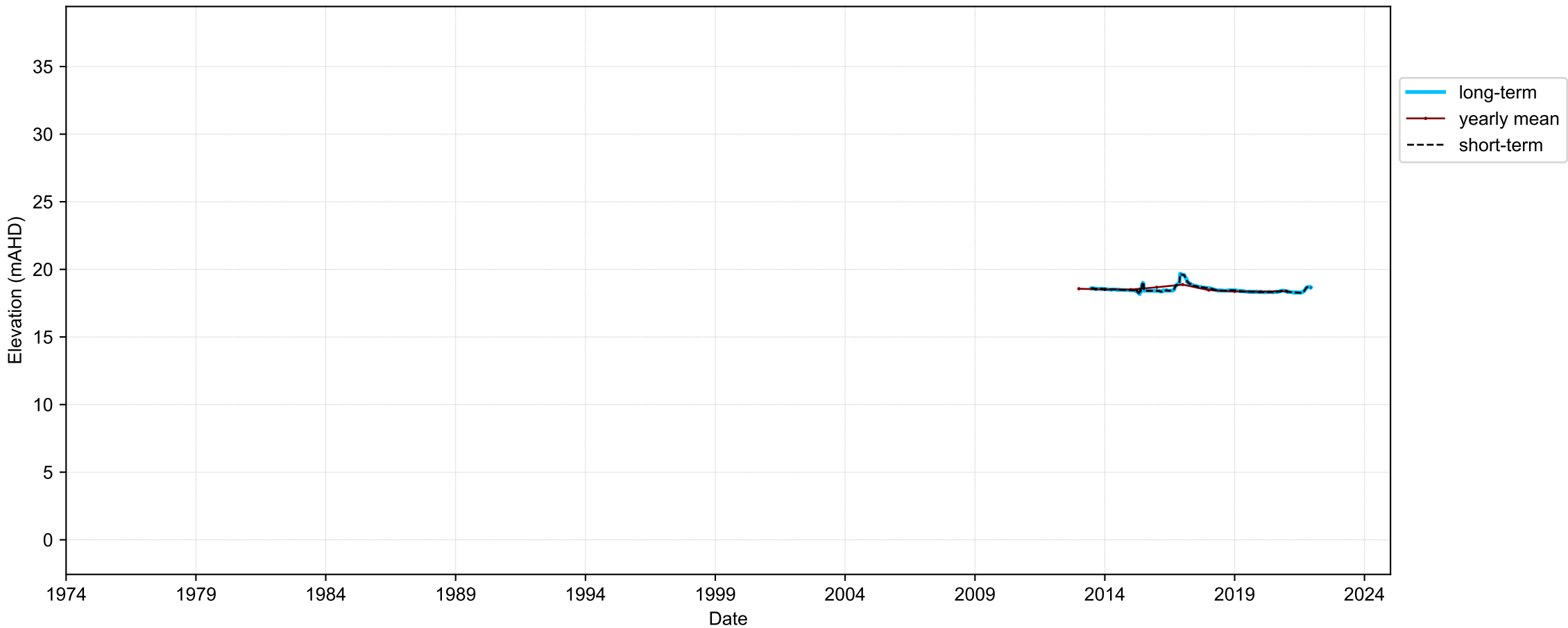
Hydrograph for hydroid: 10028276
