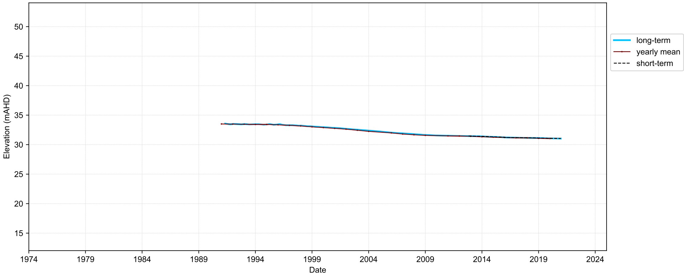
Hydrograph for hydroid: 10139927
