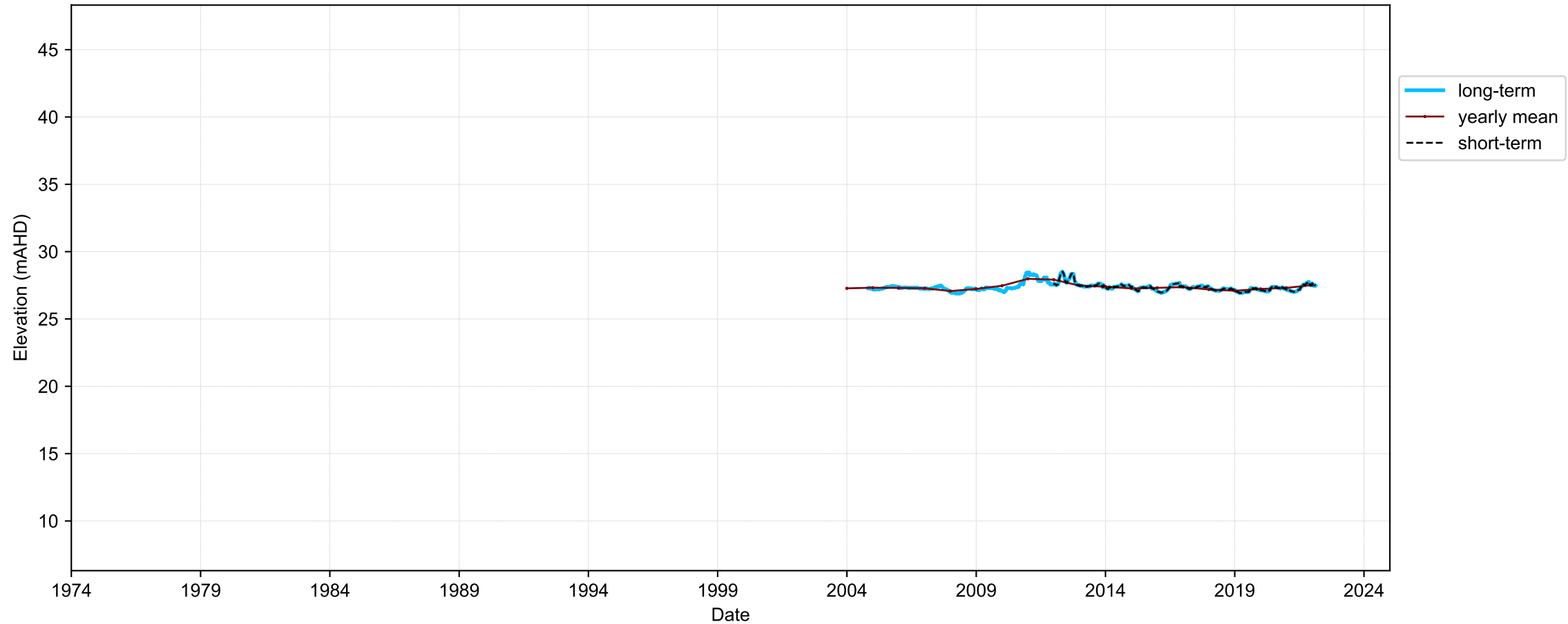
Hydrograph for hydroid: 10112887
