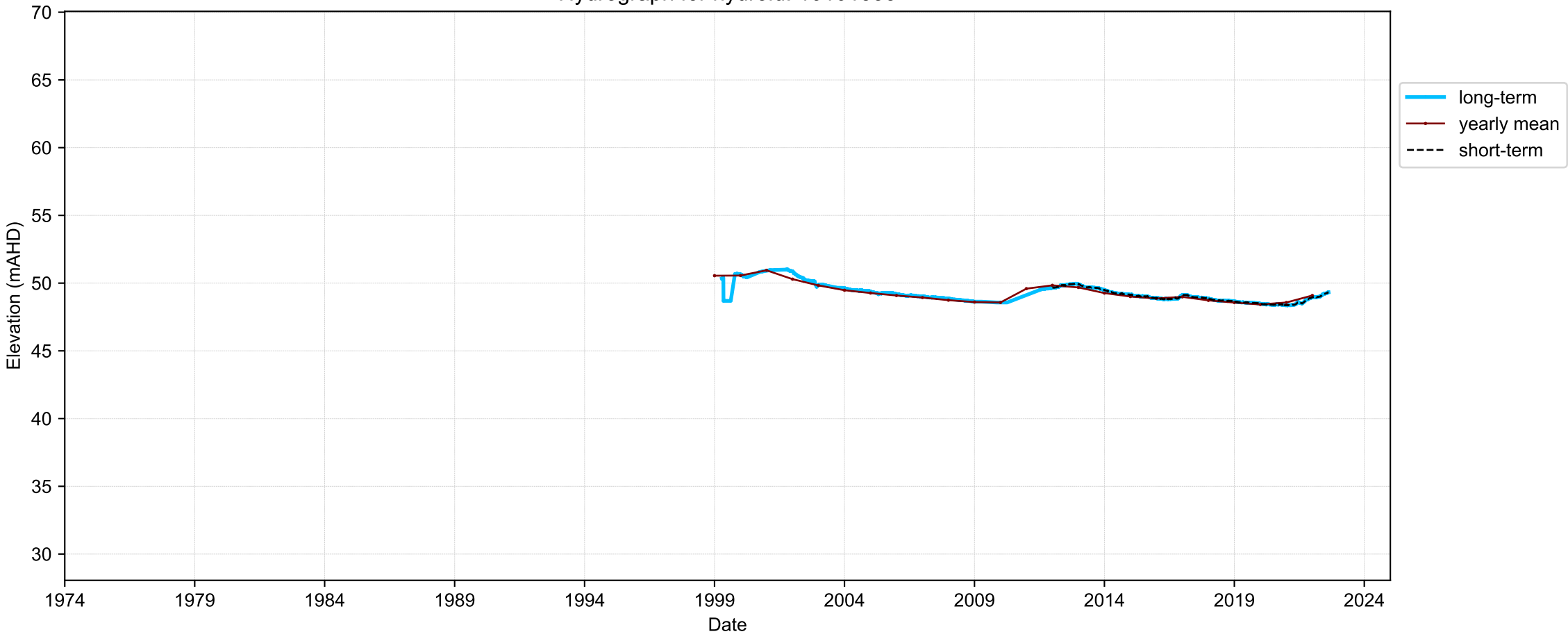
Hydrograph for hydroid: 10101855
