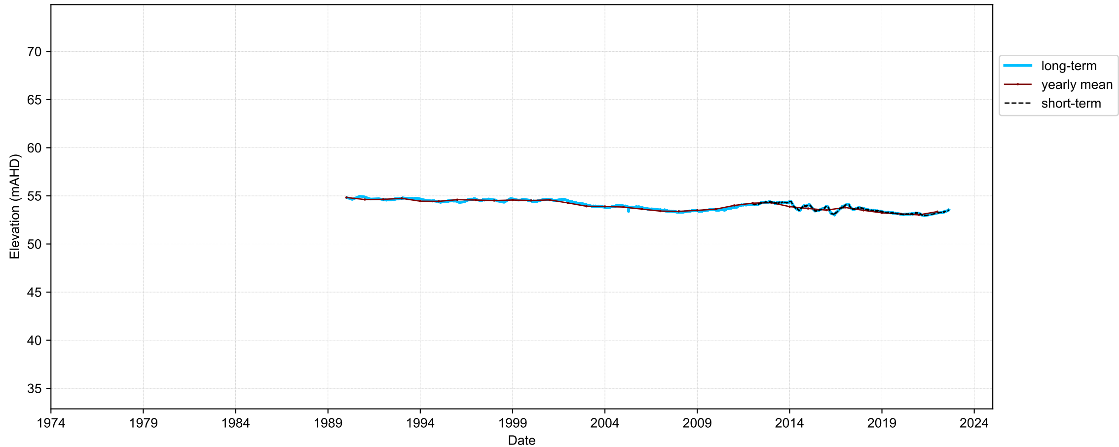
Hydrograph for hydroid: 10018046
