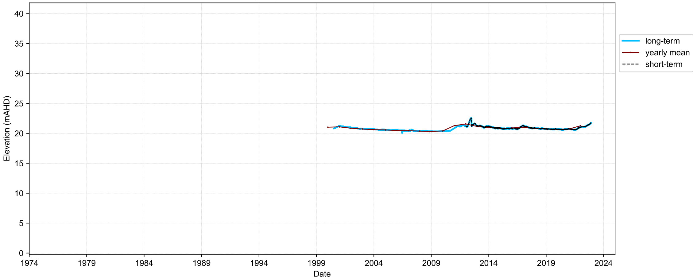
Hydrograph for hydroid: 10057526
