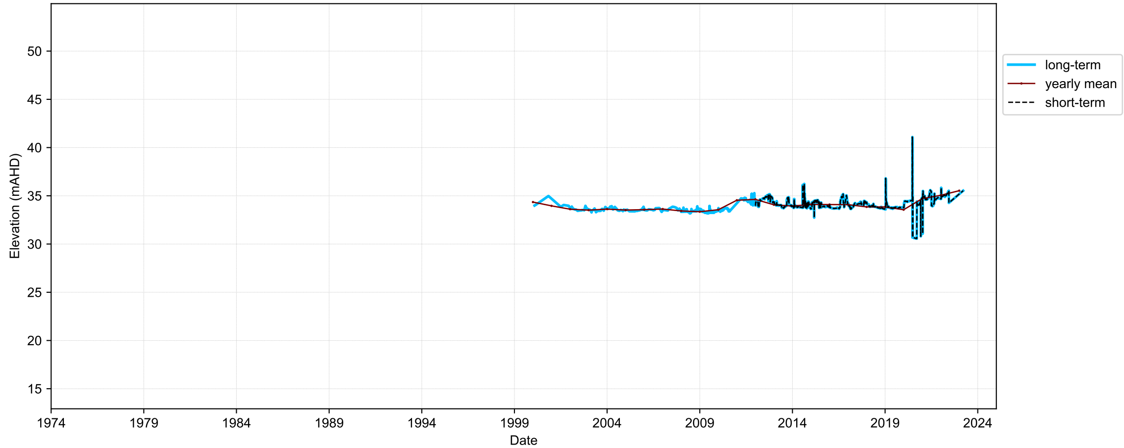
Hydrograph for hydroid: 10124371
