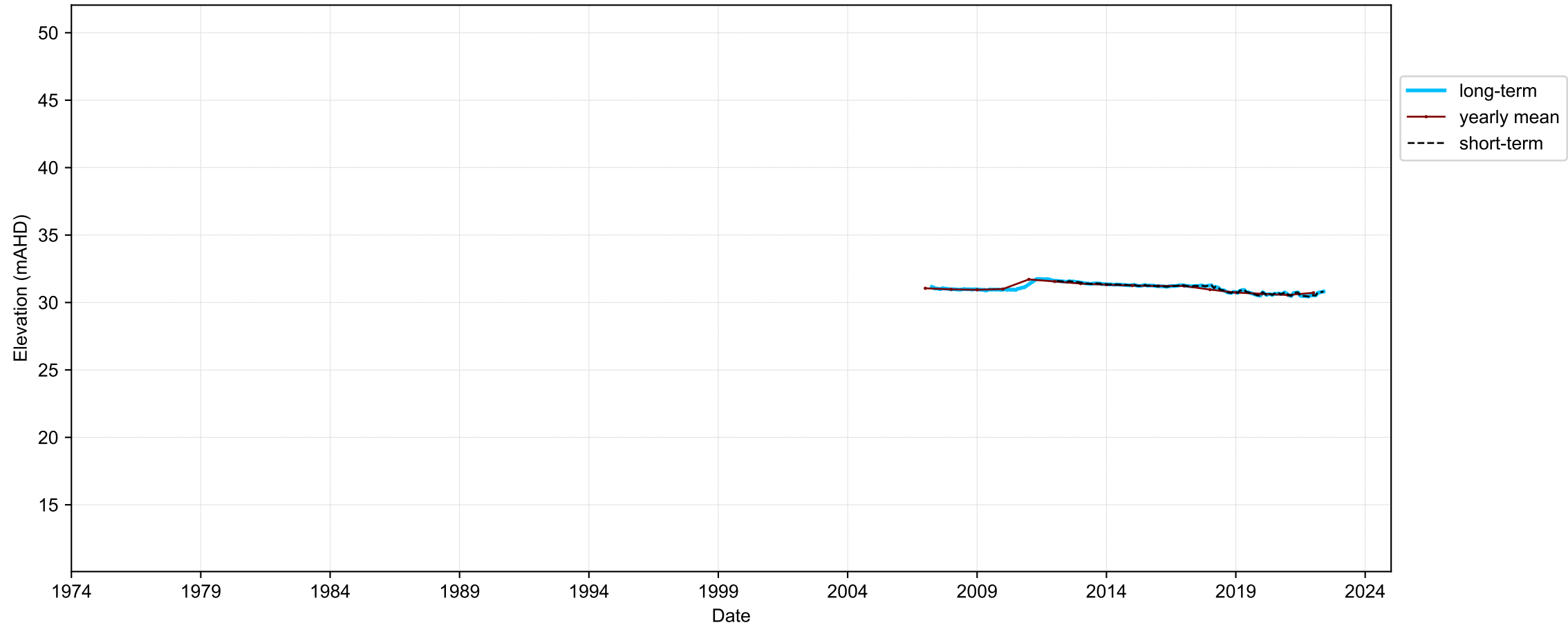
Hydrograph for hydroid: 10080215
