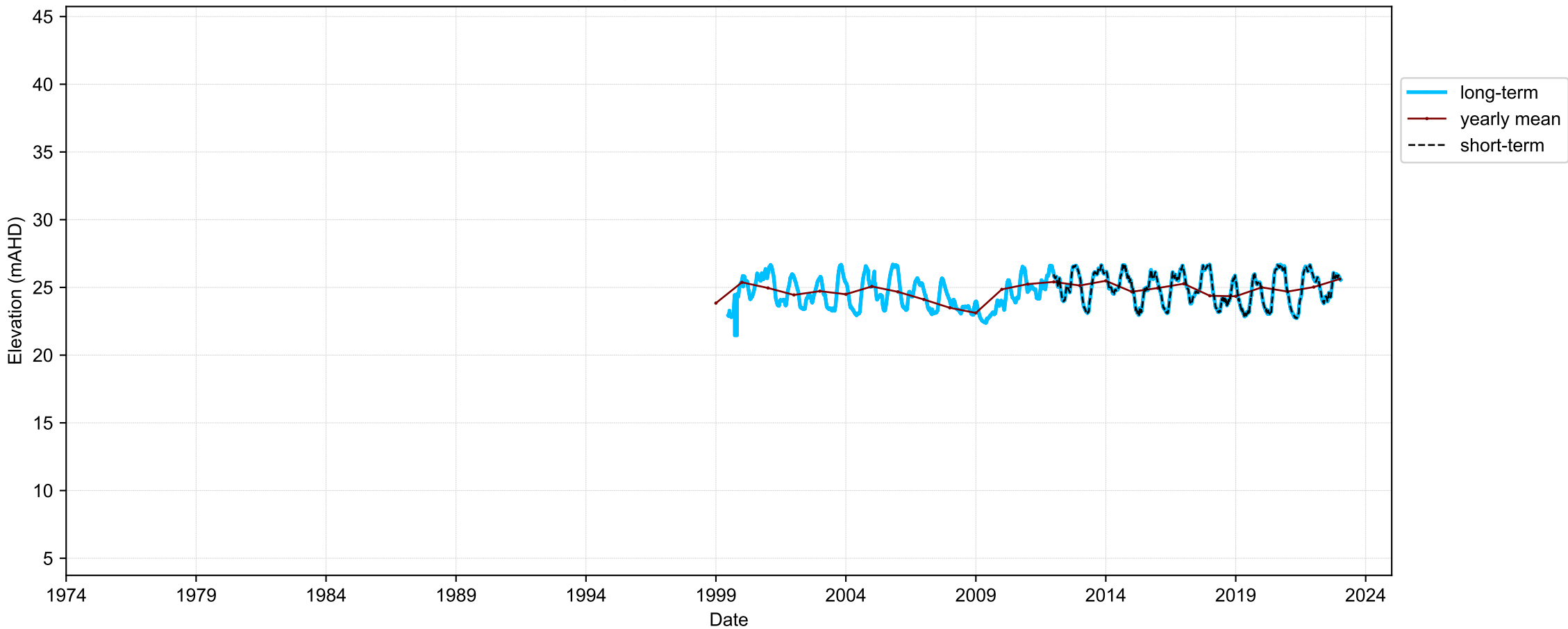
Hydrograph for hydroid: 10082610
