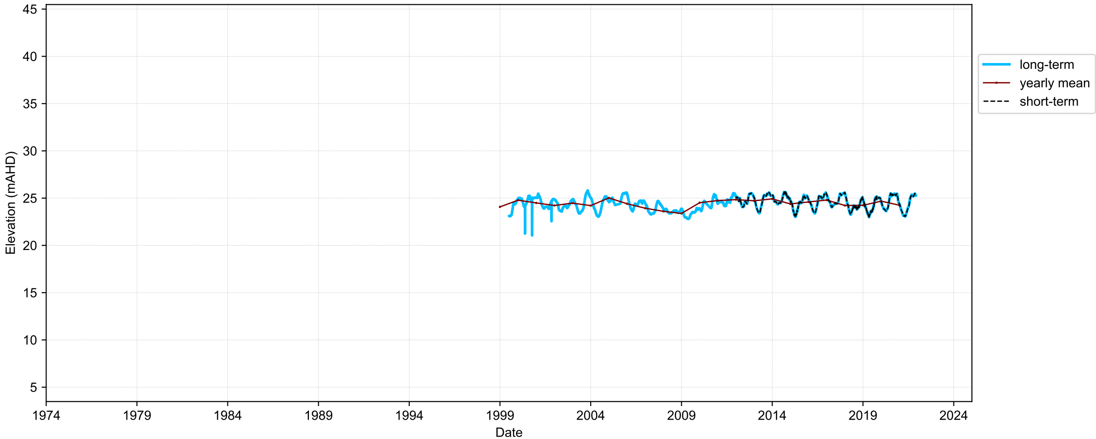
Hydrograph for hydroid: 10077748
