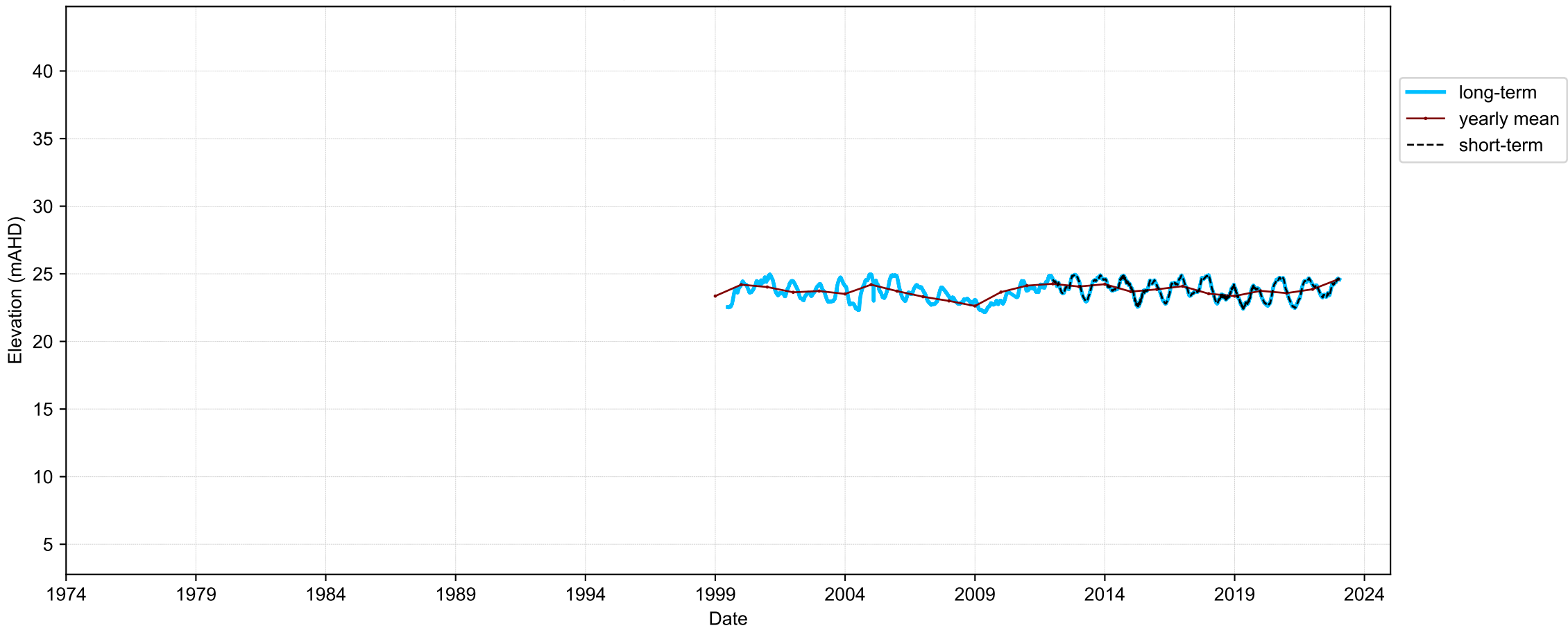
Hydrograph for hydroid: 10085740
