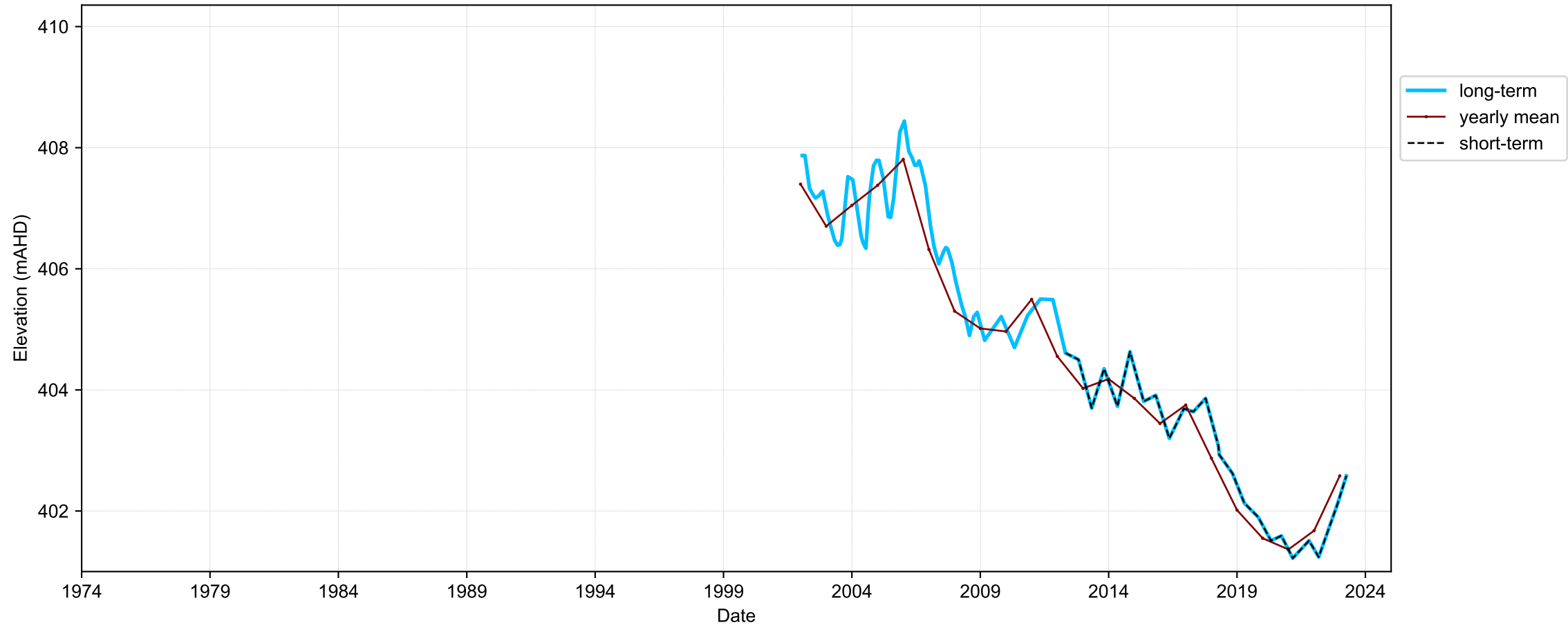
Hydrograph for hydroid: 30076254
