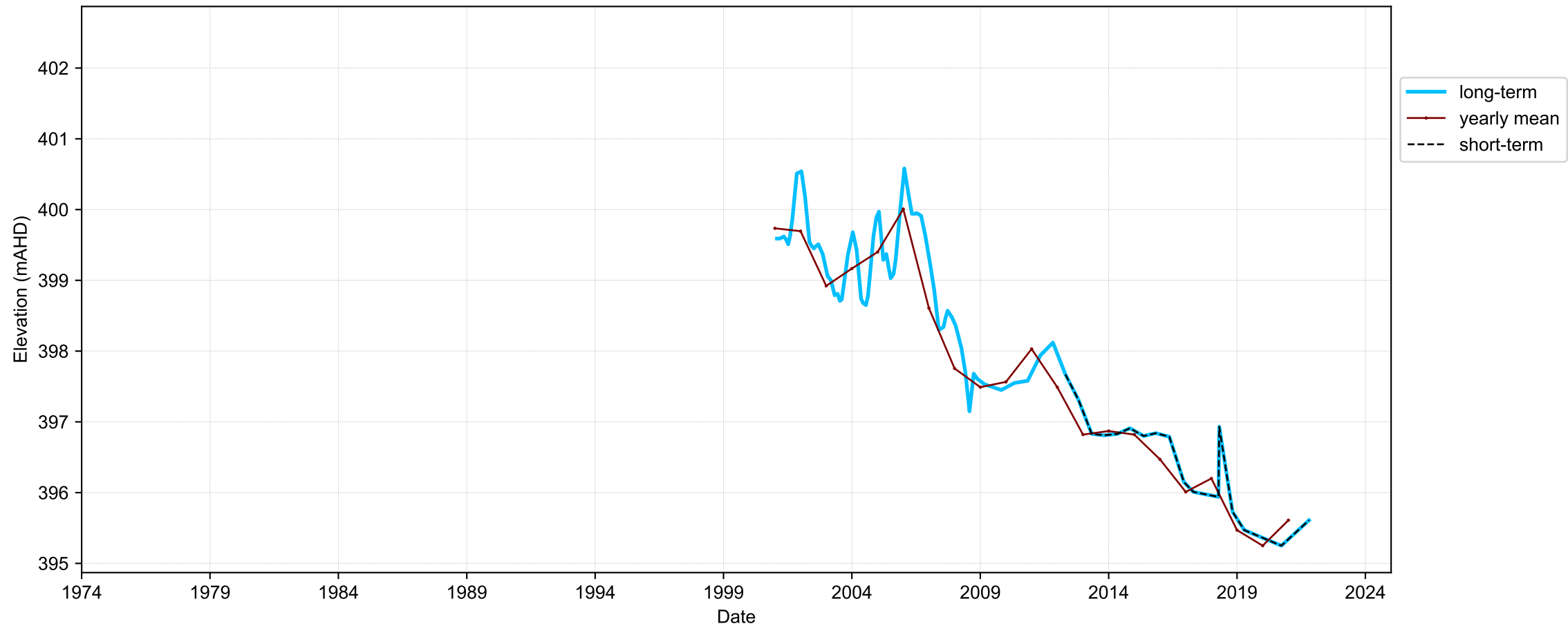
Hydrograph for hydroid: 30120708
