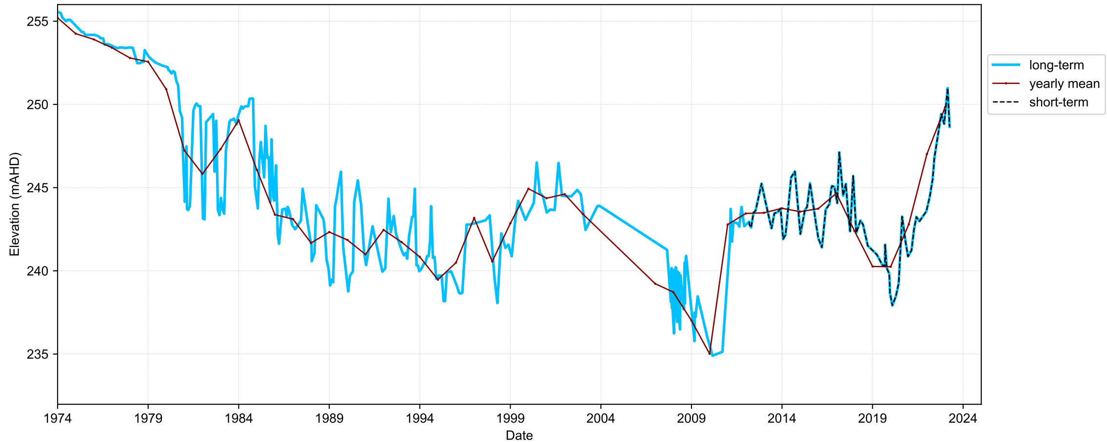
Hydrograph for hydroid: 10005146
