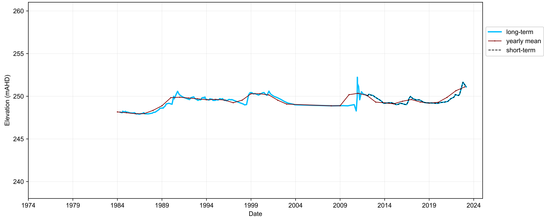
Hydrograph for hydroid: 10056316
