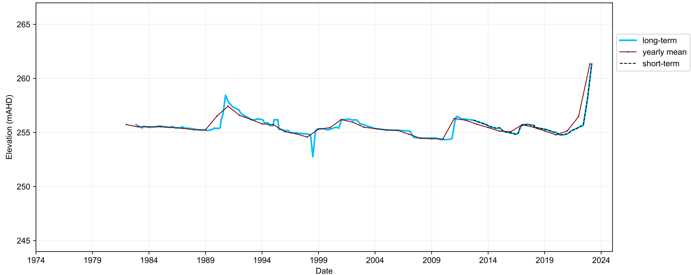
Hydrograph for hydroid: 10056523
