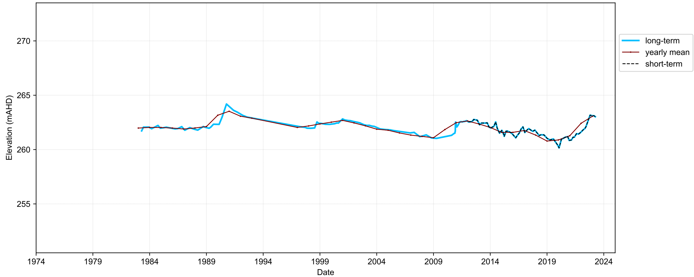
Hydrograph for hydroid: 10071539
