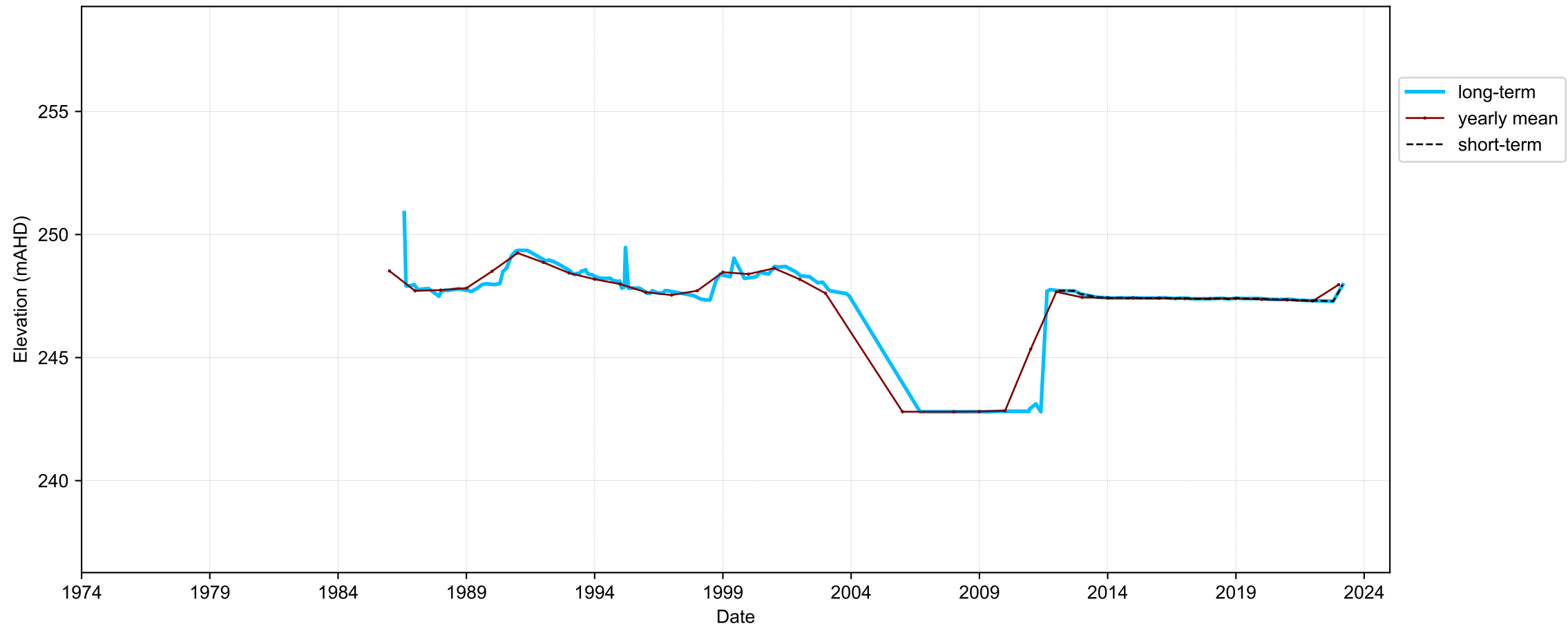
Hydrograph for hydroid: 10067385
