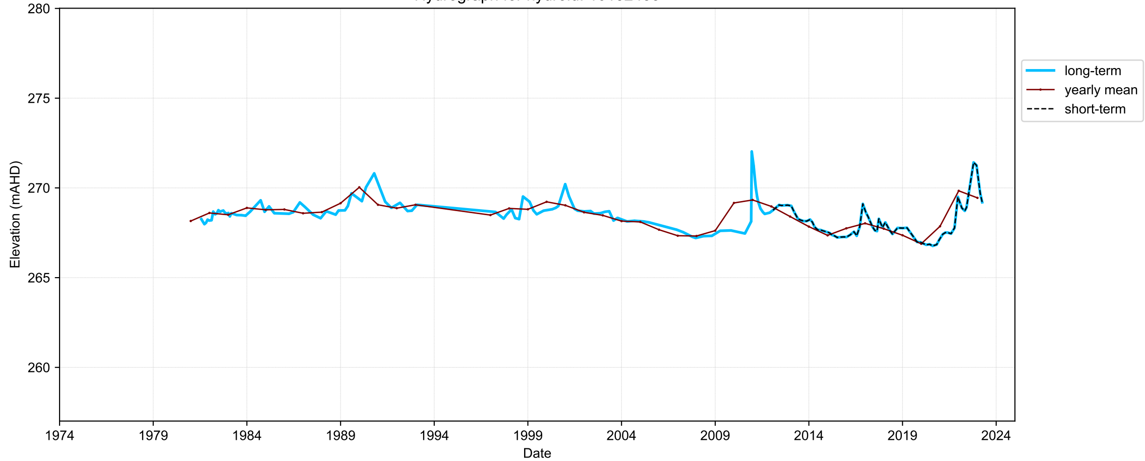
Hydrograph for hydroid: 10132455
