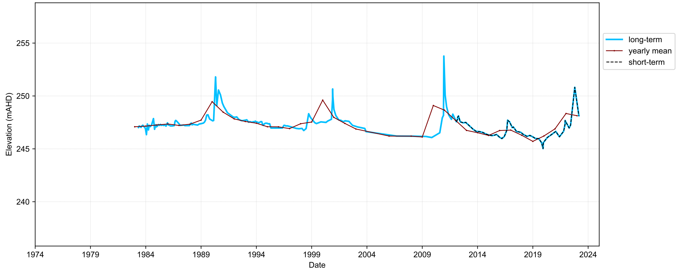
Hydrograph for hydroid: 10060082
