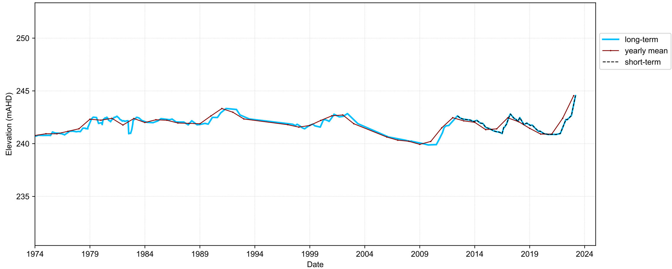
Hydrograph for hydroid: 10015523
