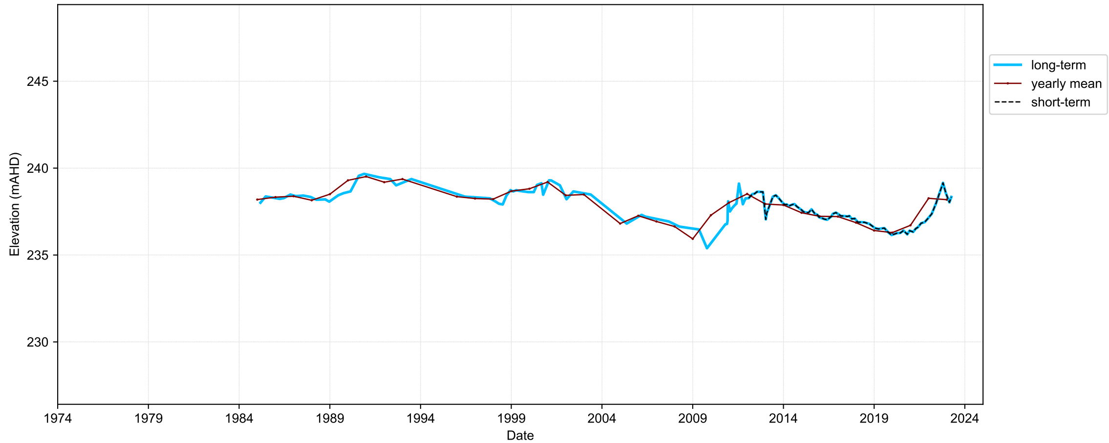
Hydrograph for hydroid: 10134031
