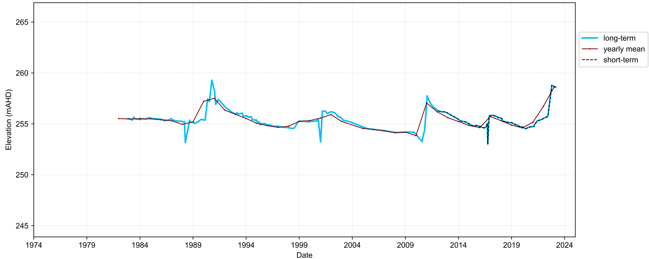
Hydrograph for hydroid: 10052603
