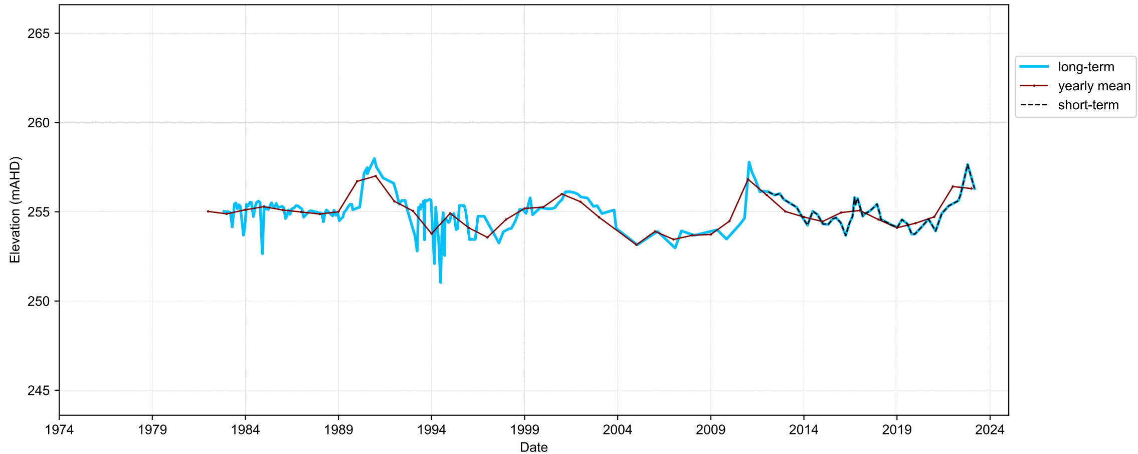
Hydrograph for hydroid: 10049339
