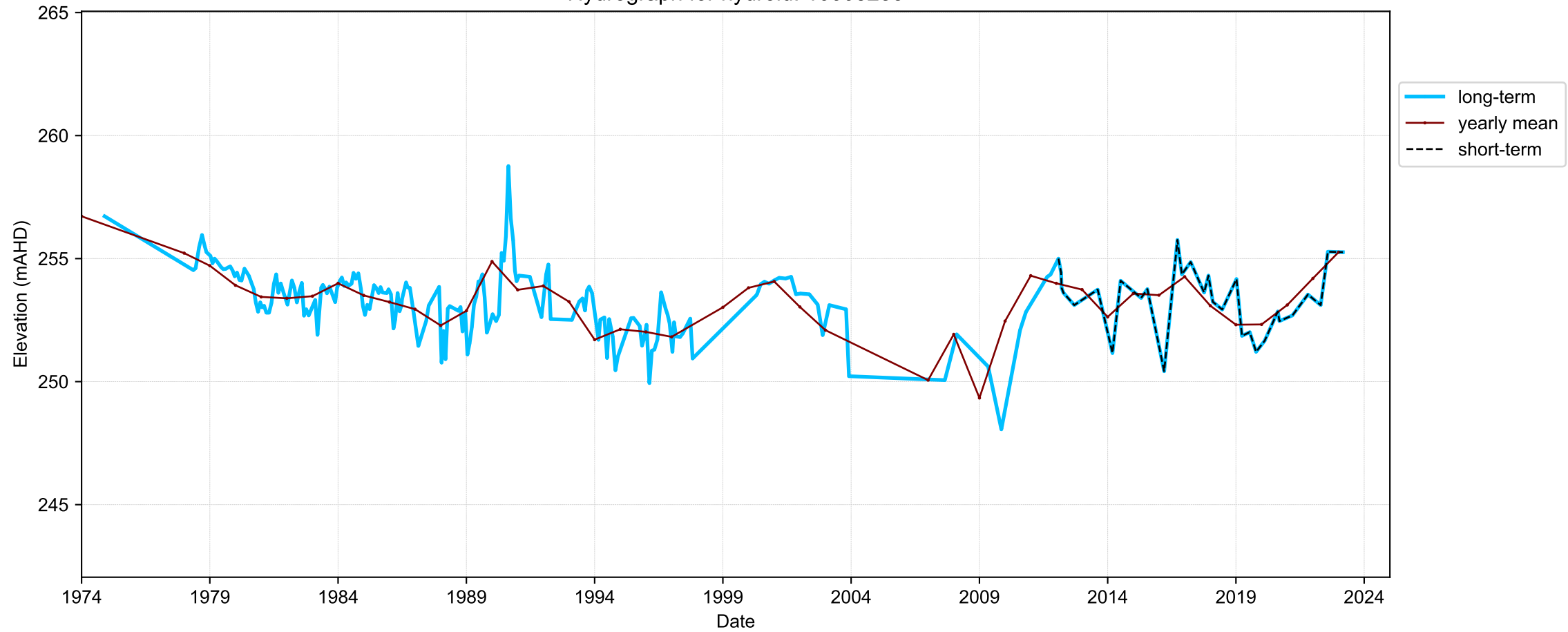
Hydrograph for hydroid: 10003258
