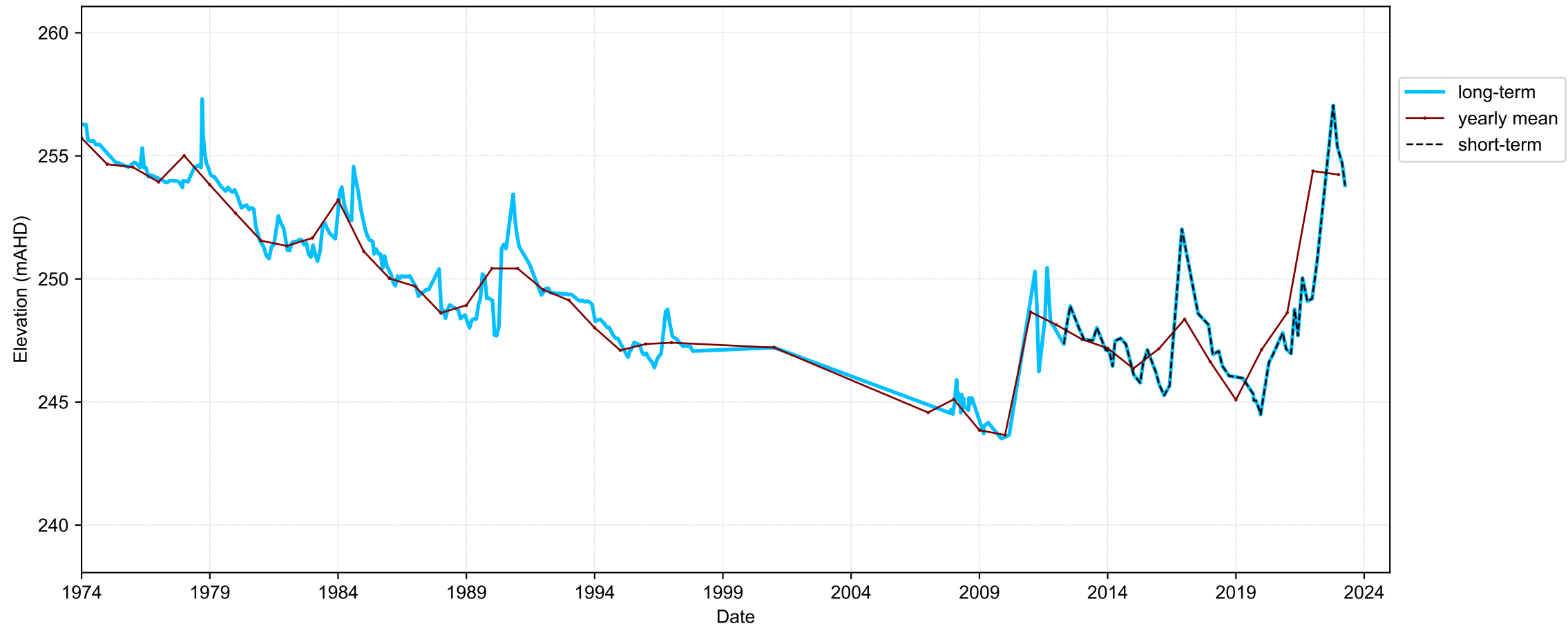
Hydrograph for hydroid: 10005973
