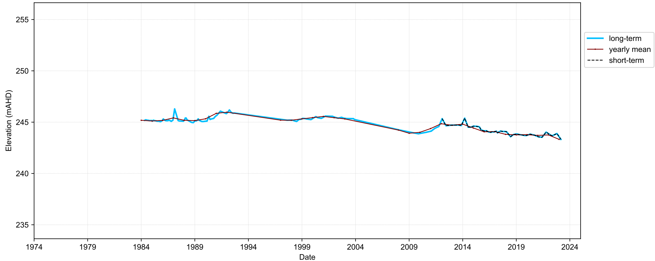
Hydrograph for hydroid: 10111877
