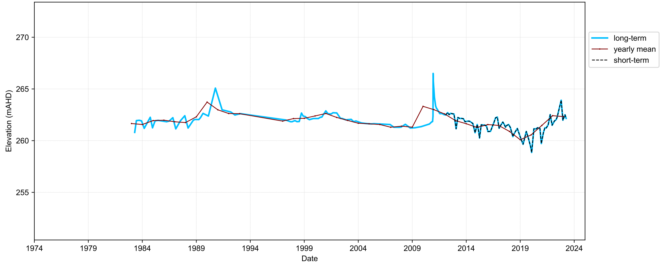
Hydrograph for hydroid: 10059994
