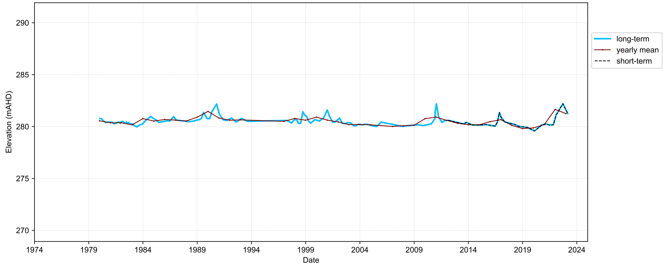
Hydrograph for hydroid: 10008544
