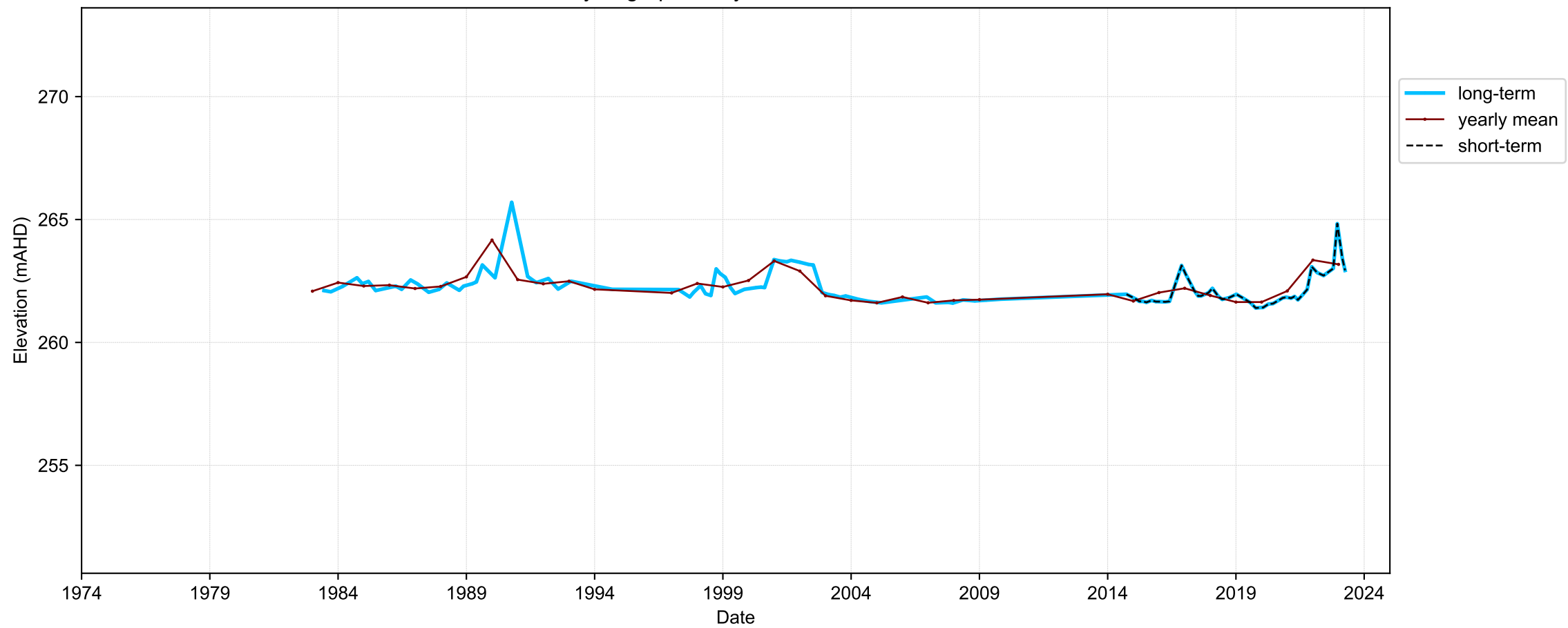
Hydrograph for hydroid: 10070151
