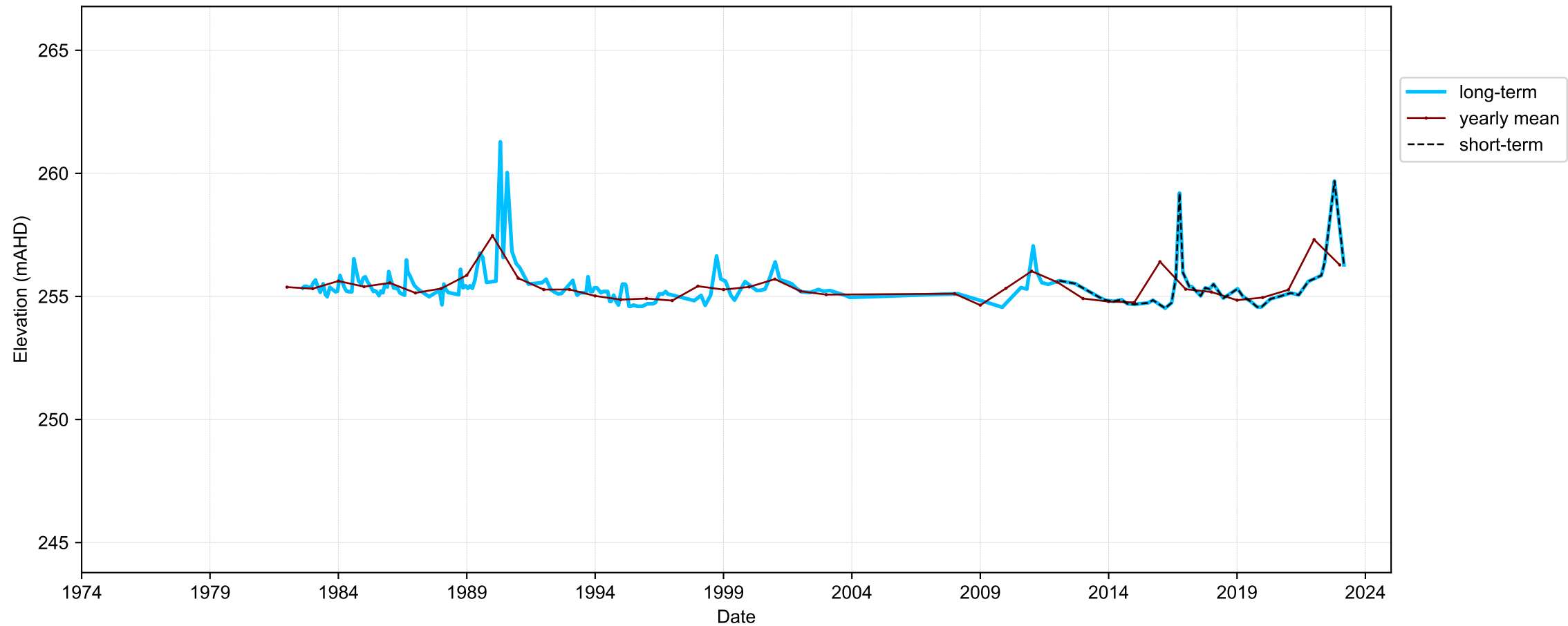
Hydrograph for hydroid: 10049283
