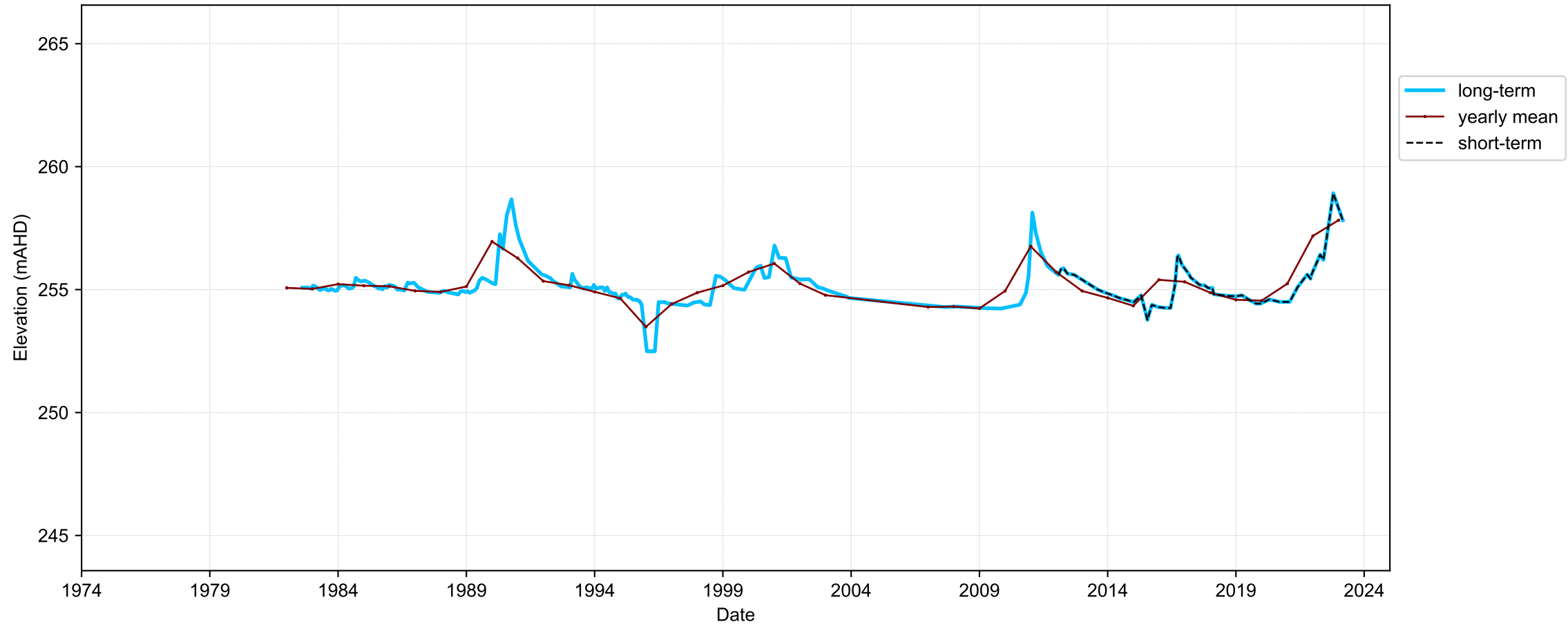
Hydrograph for hydroid: 10050591
