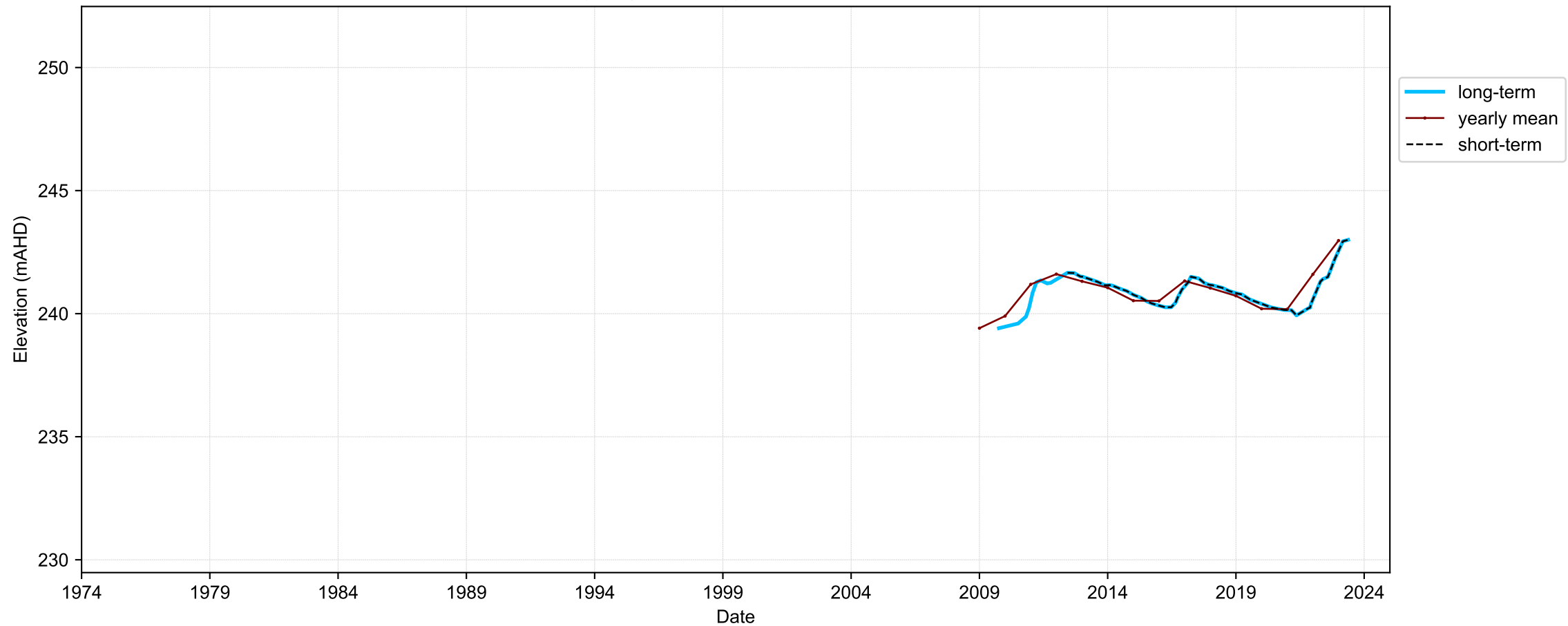
Hydrograph for hydroid: 10091940
