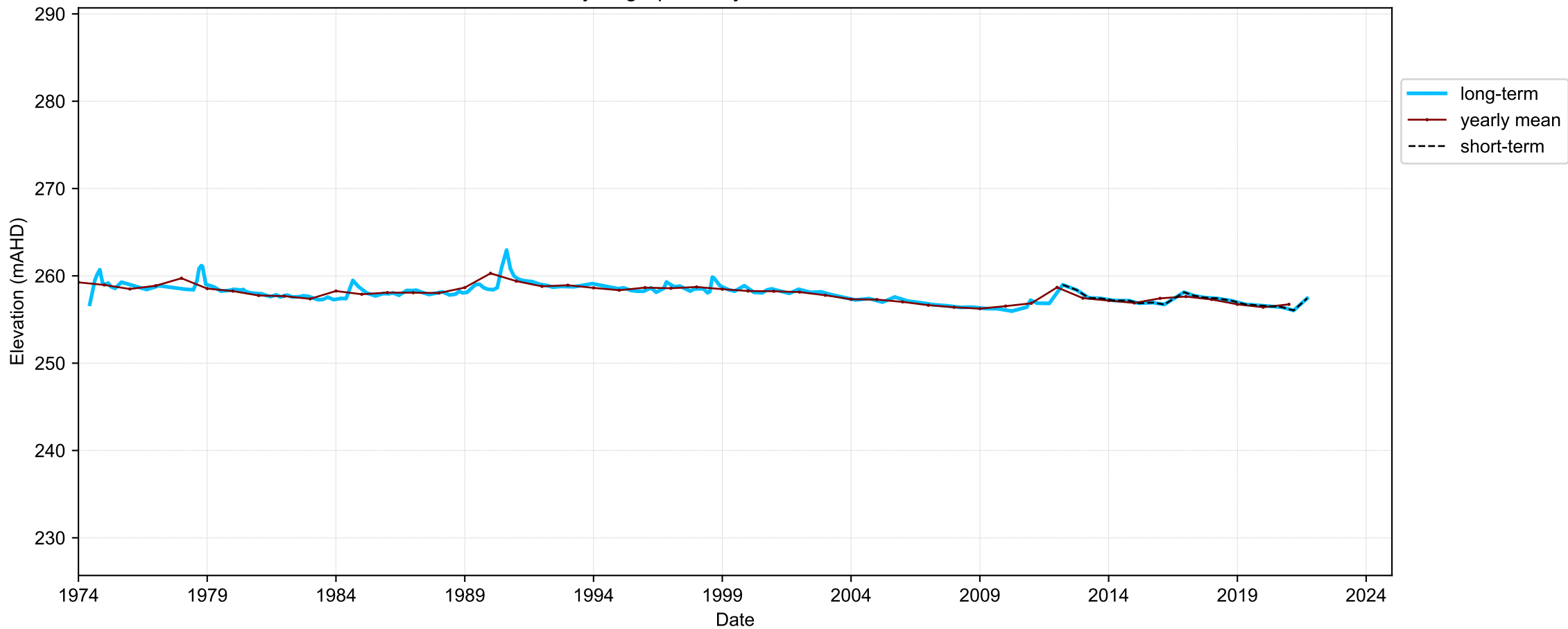
Hydrograph for hydroid: 10133001
