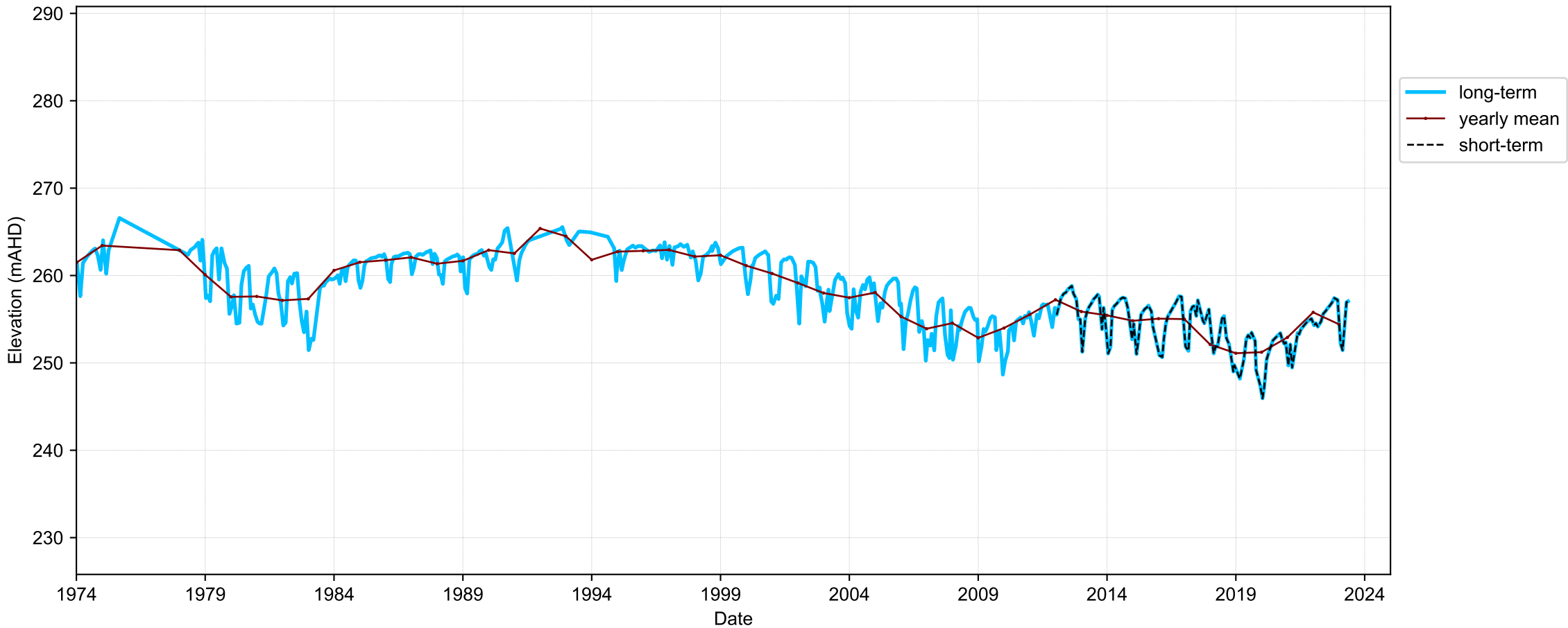
Hydrograph for hydroid: 10021709
