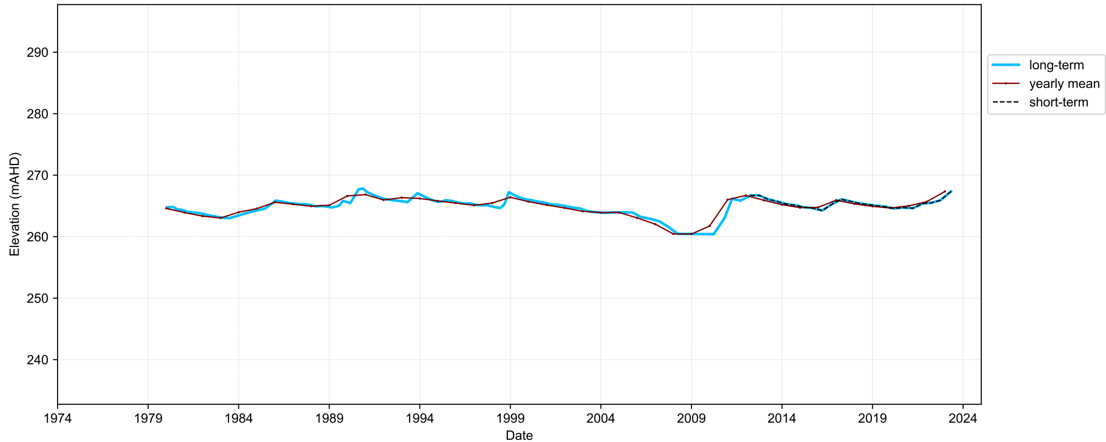
Hydrograph for hydroid: 10111176
