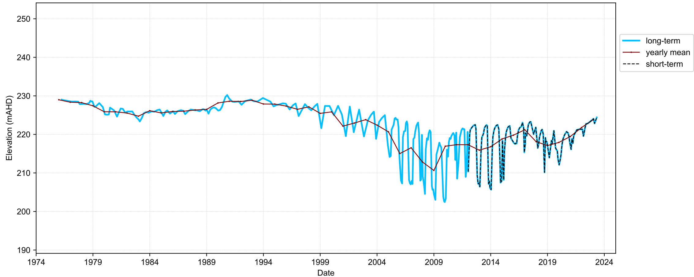
Hydrograph for hydroid: 10105159
