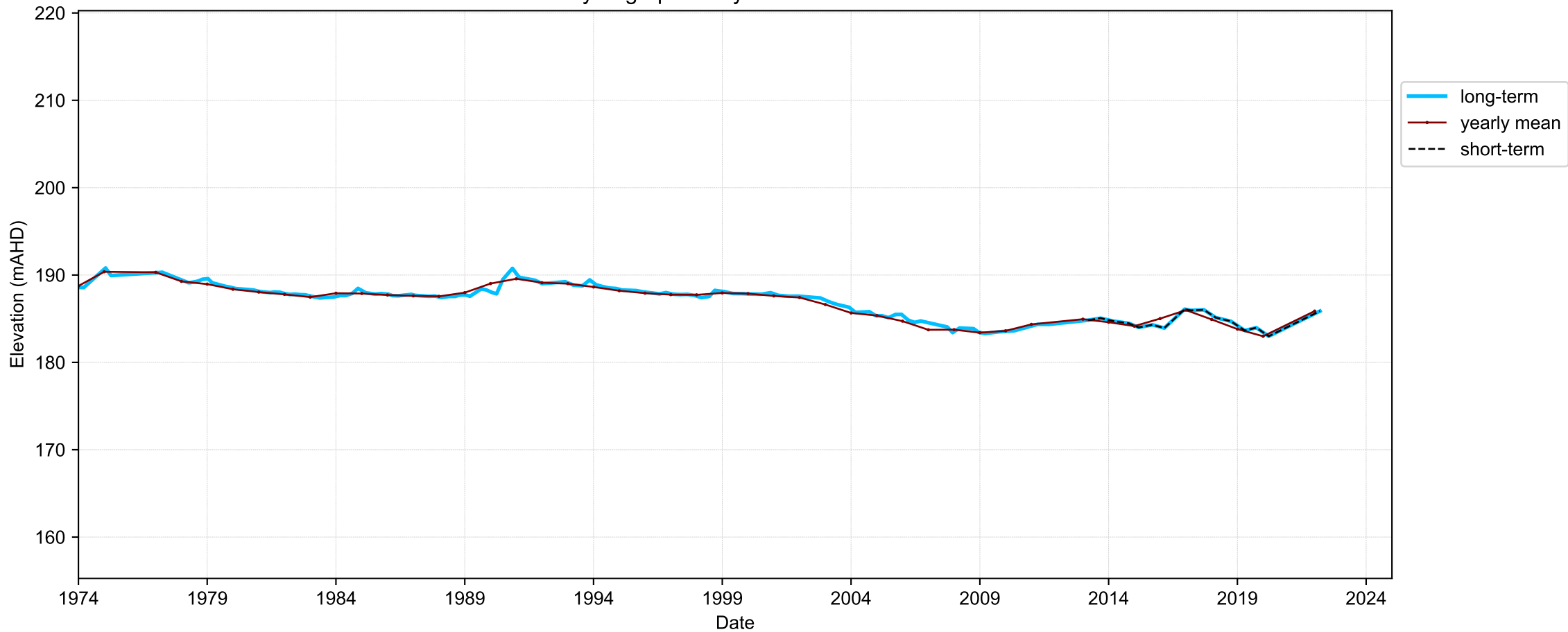
Hydrograph for hydroid: 10151298
