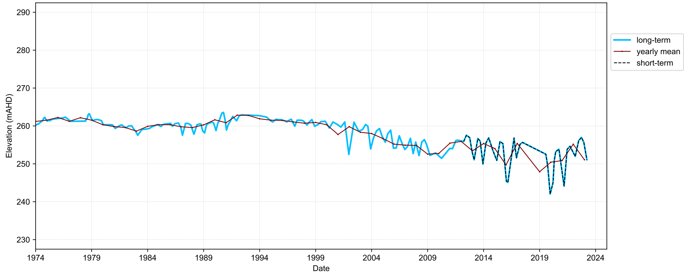
Hydrograph for hydroid: 10016007
