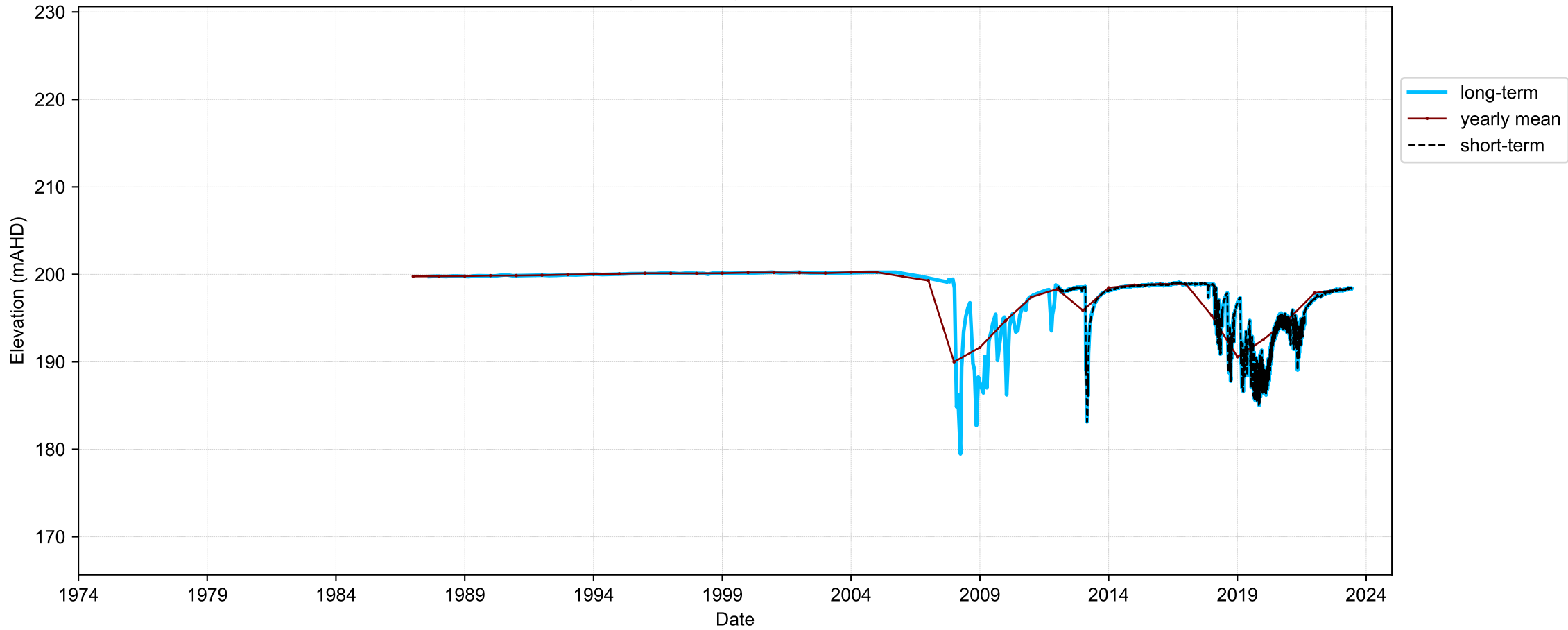
Hydrograph for hydroid: 10005994
