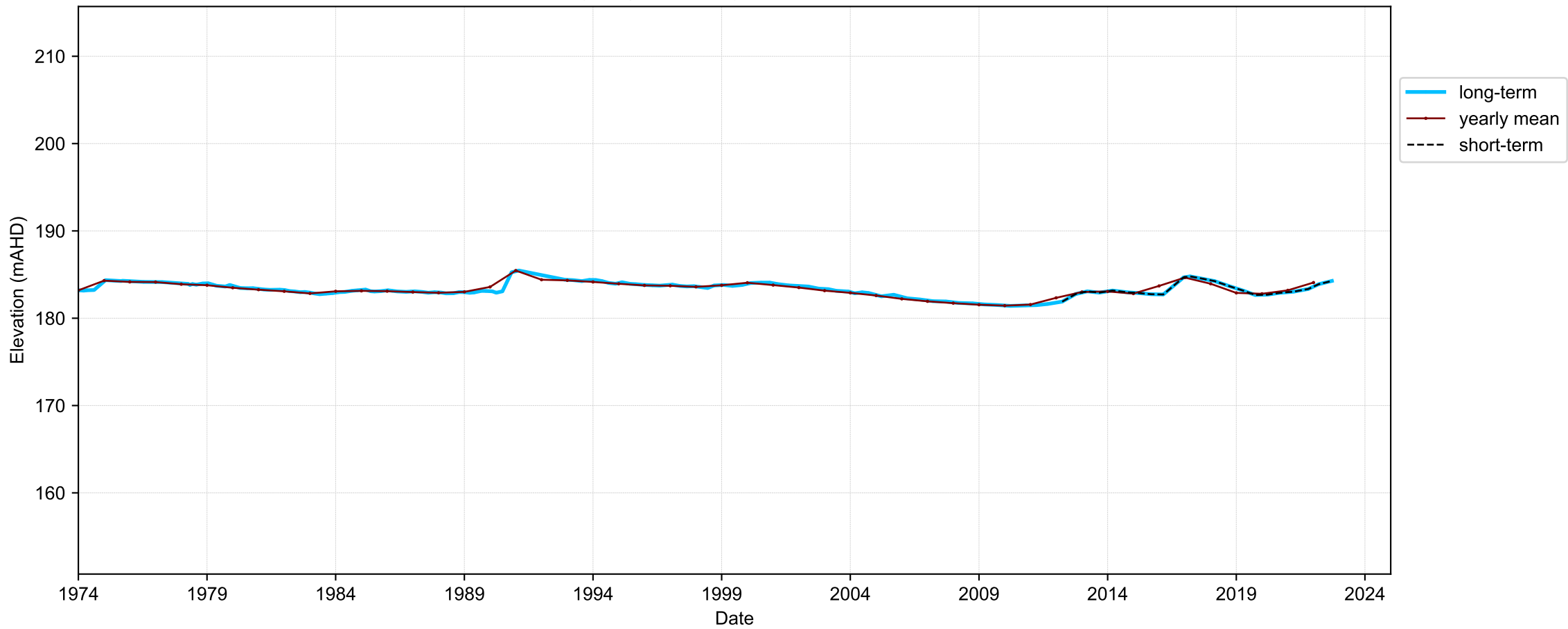
Hydrograph for hydroid: 10140230
