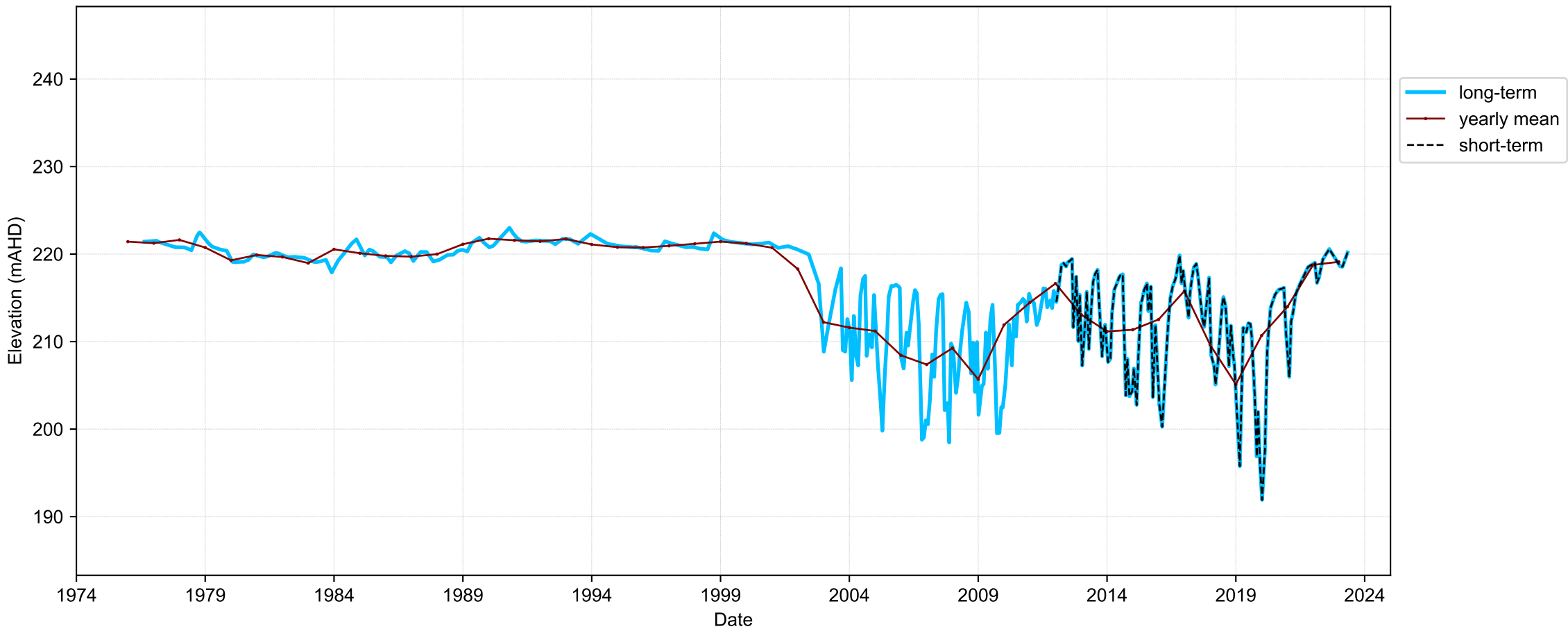
Hydrograph for hydroid: 10140012
