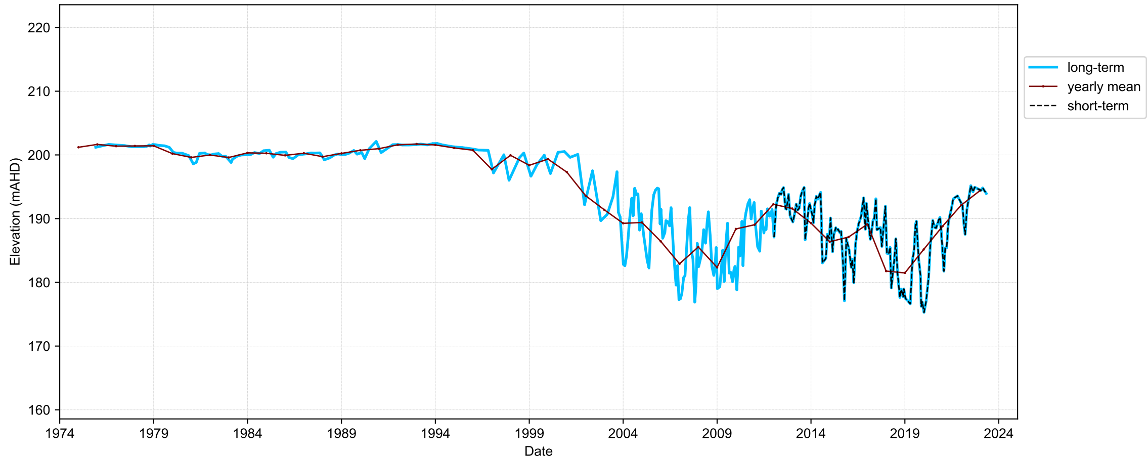
Hydrograph for hydroid: 10108694
