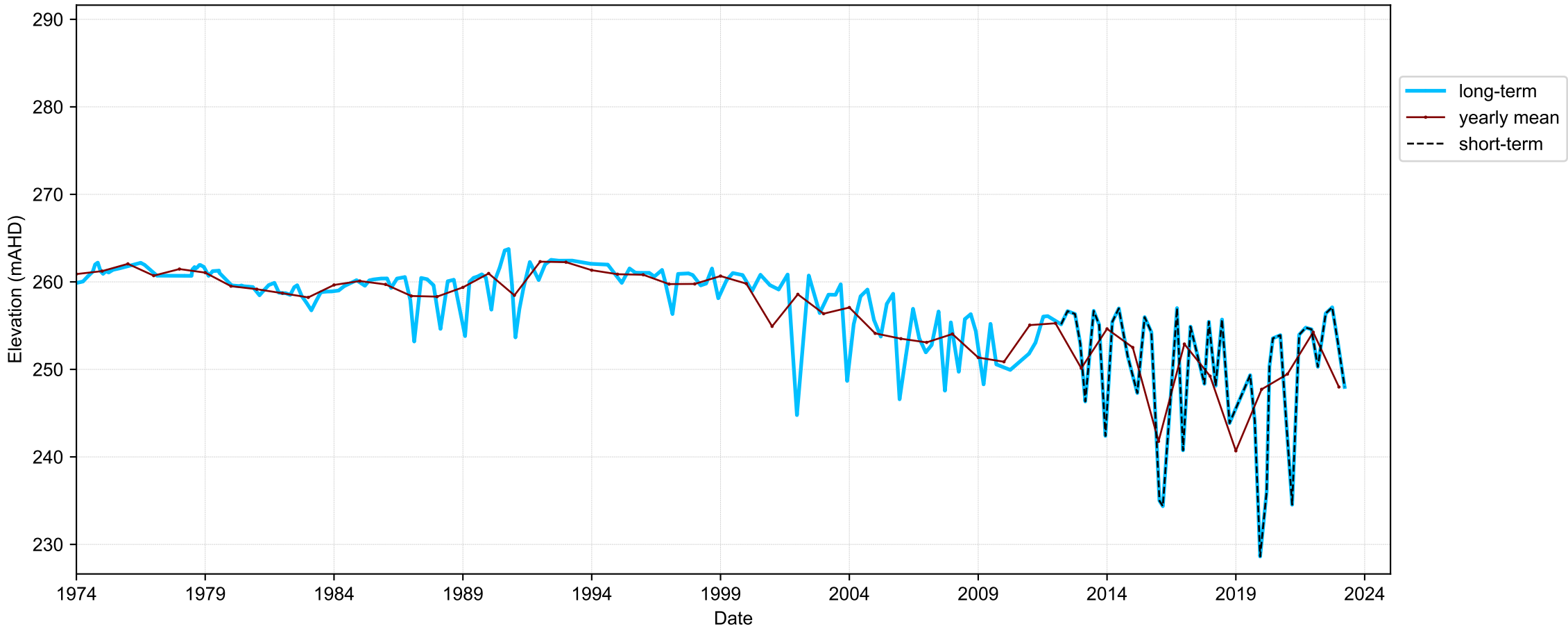
Hydrograph for hydroid: 10007318
