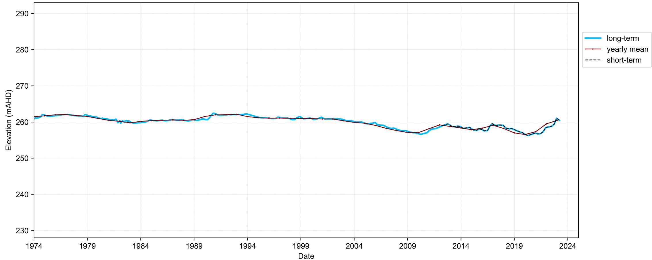
Hydrograph for hydroid: 10114370
