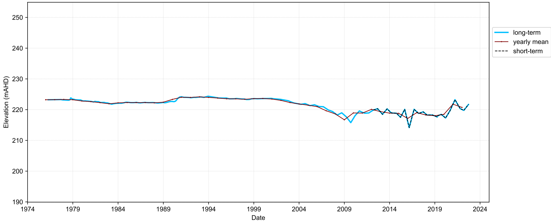
Hydrograph for hydroid: 10023974
