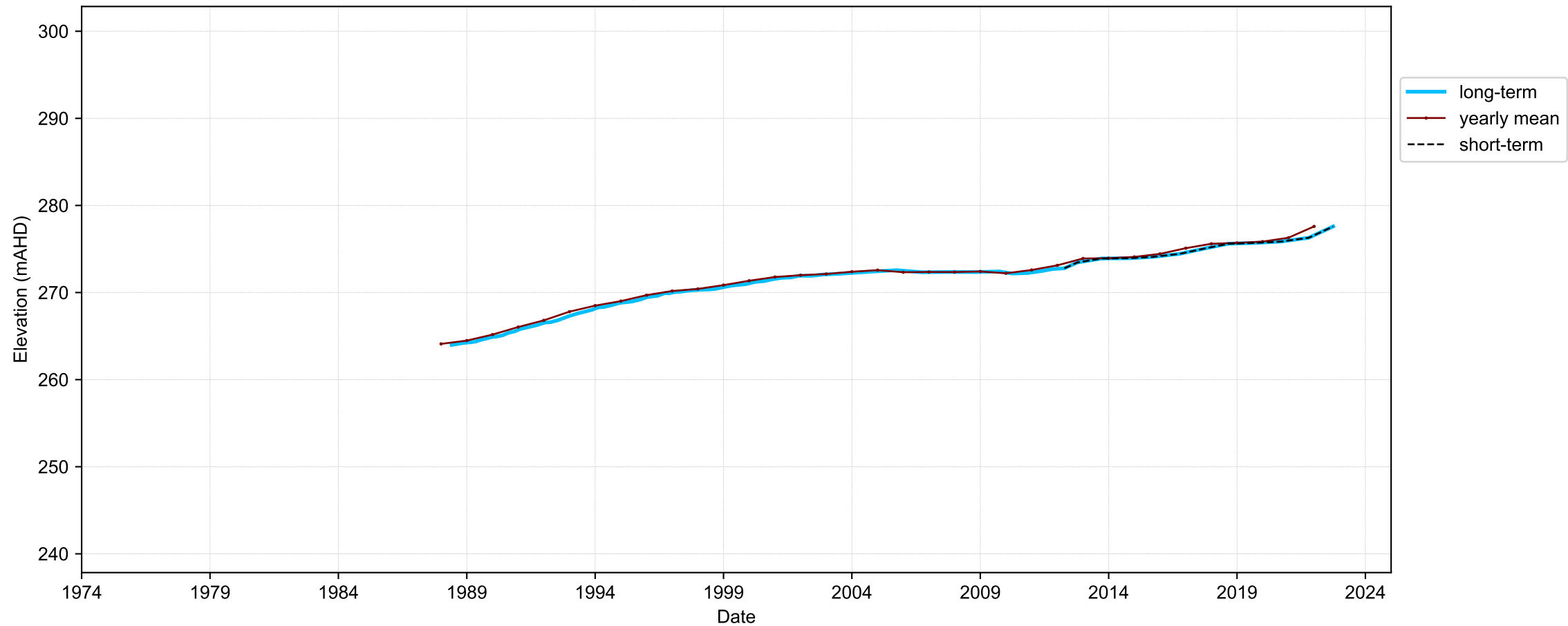
Hydrograph for hydroid: 10073368
