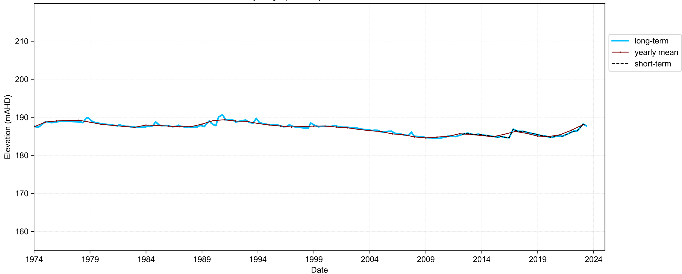
Hydrograph for hydroid: 10109394
