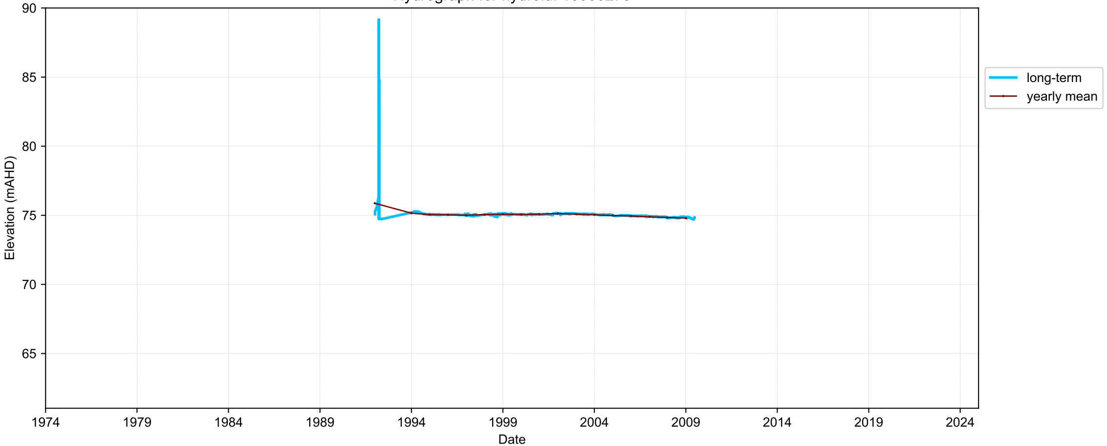
Hydrograph for hydroid: 10006275
