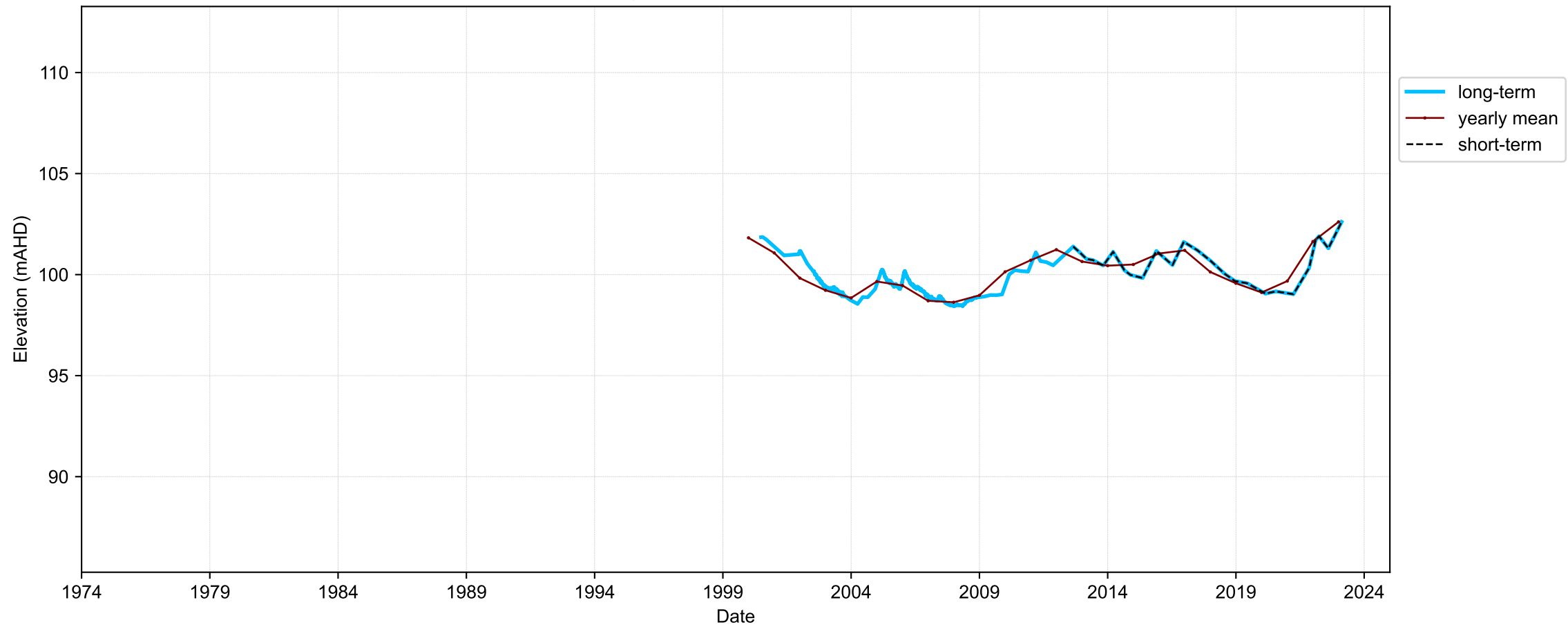
Hydrograph for hydroid: 10011154
