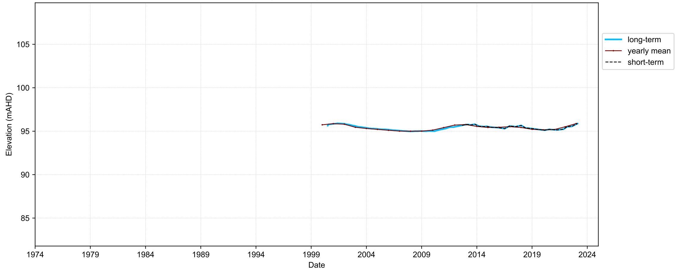
Hydrograph for hydroid: 10015692
