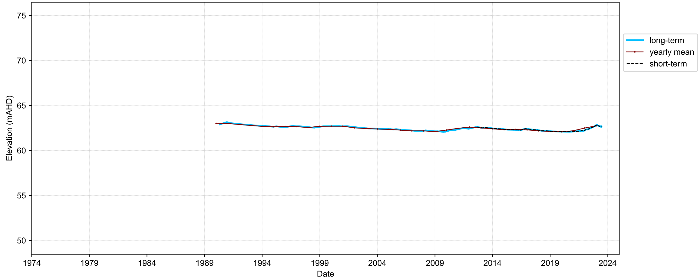
Hydrograph for hydroid: 10112729
