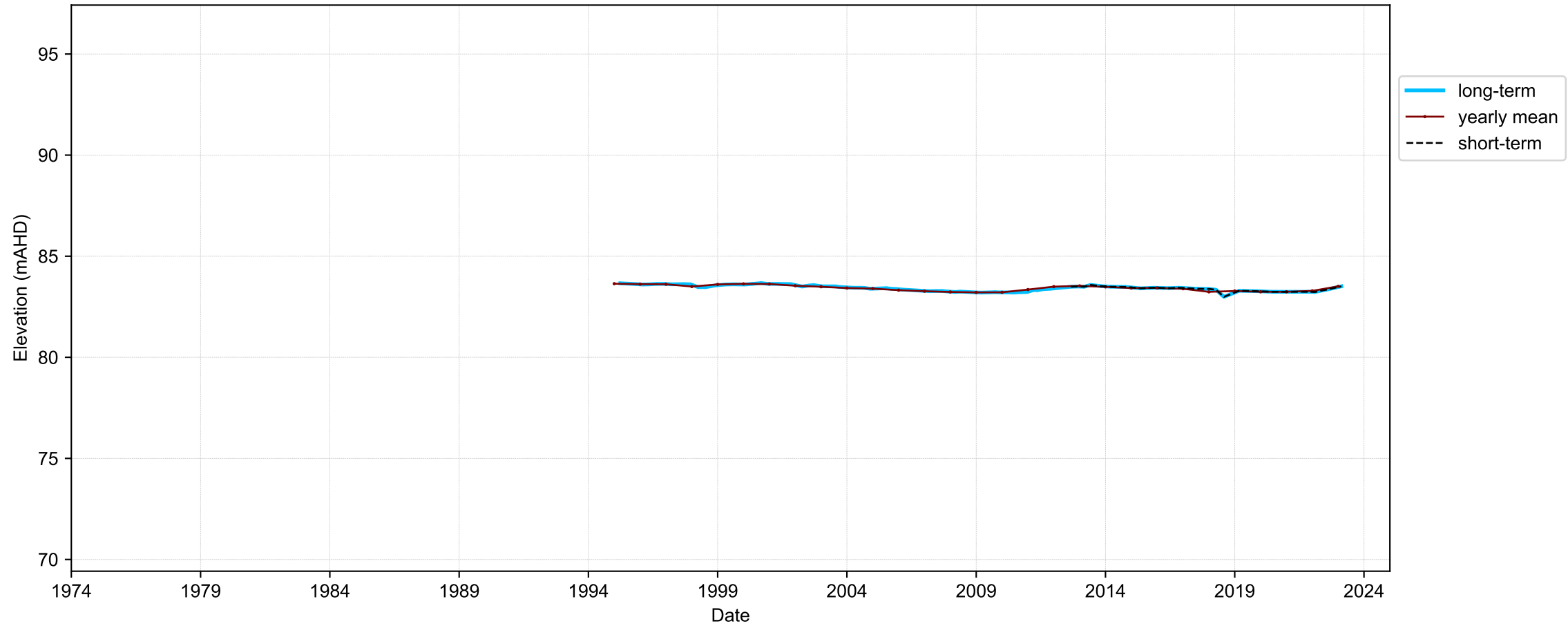
Hydrograph for hydroid: 10132017
