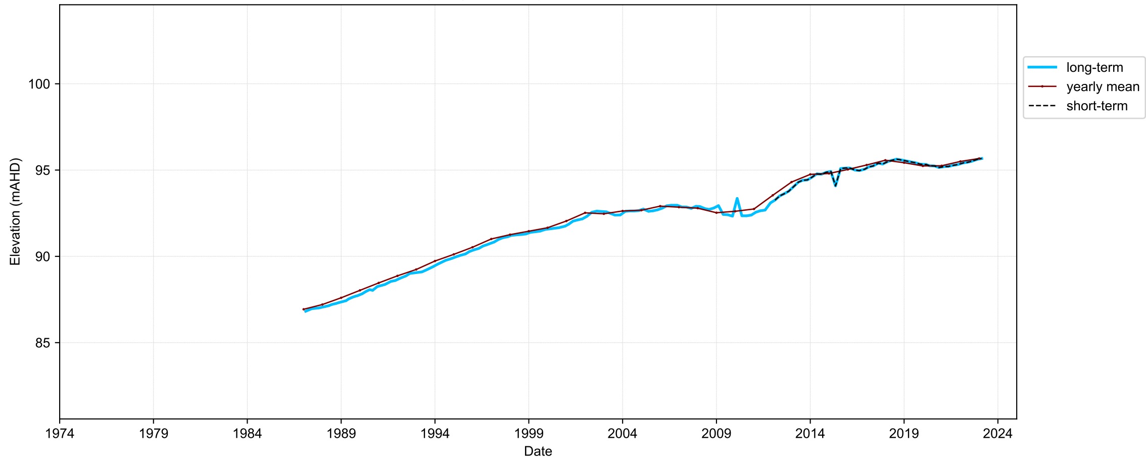
Hydrograph for hydroid: 10101174
