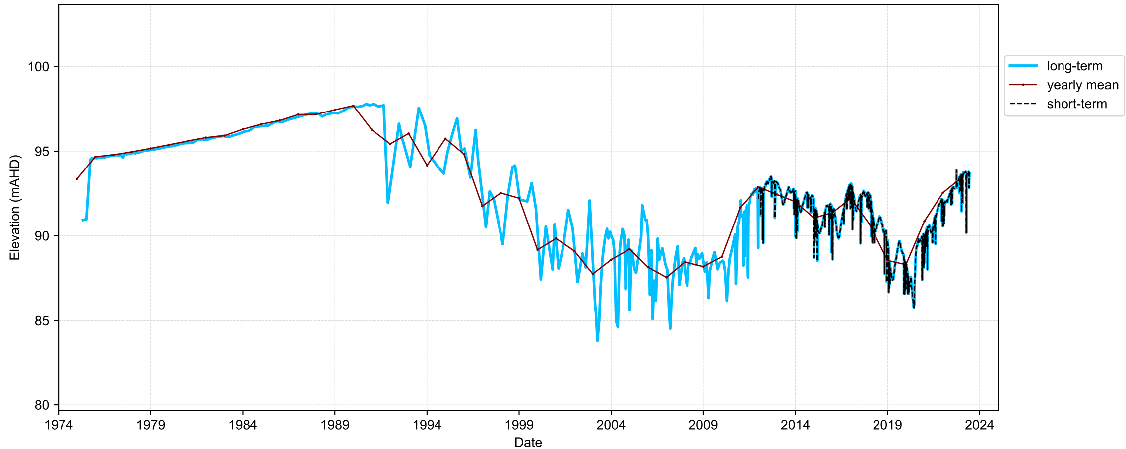
Hydrograph for hydroid: 10004661
