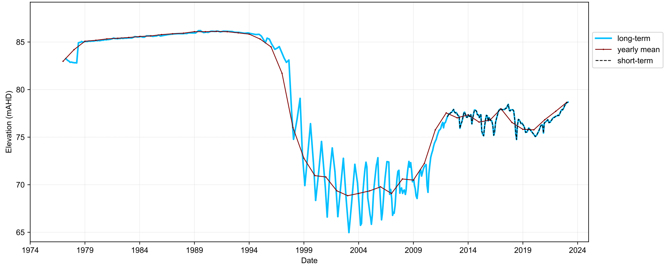
Hydrograph for hydroid: 10004310
