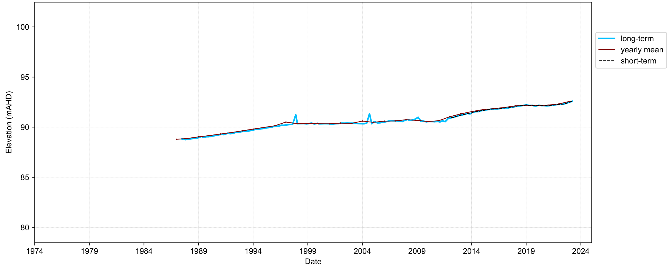
Hydrograph for hydroid: 10049036
