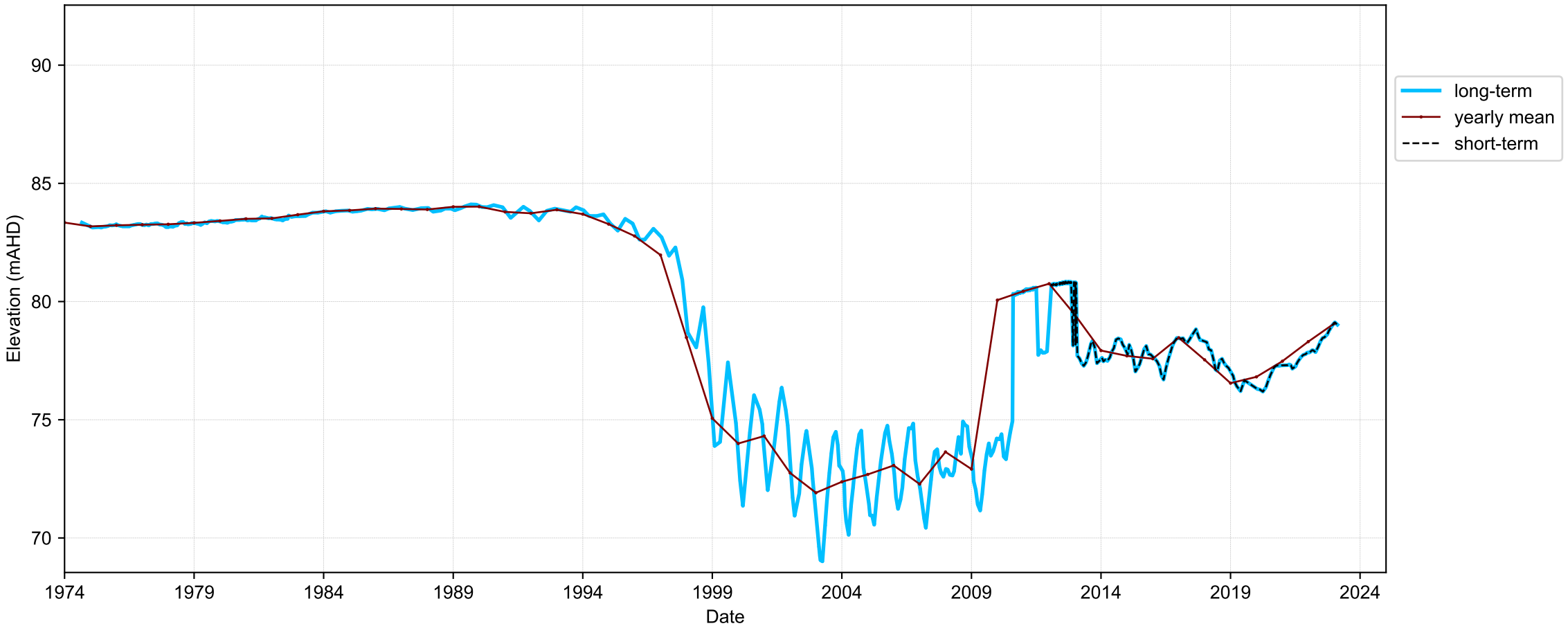
Hydrograph for hydroid: 10105788
