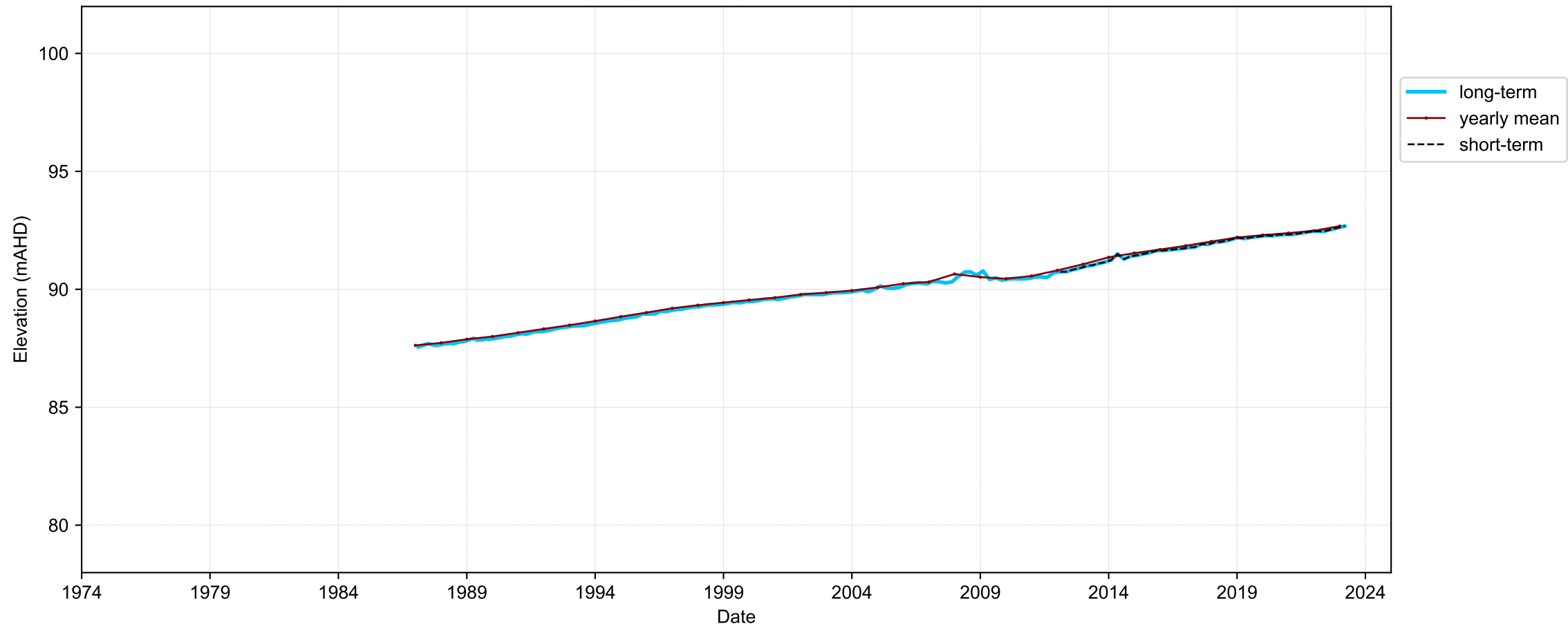
Hydrograph for hydroid: 10046388
