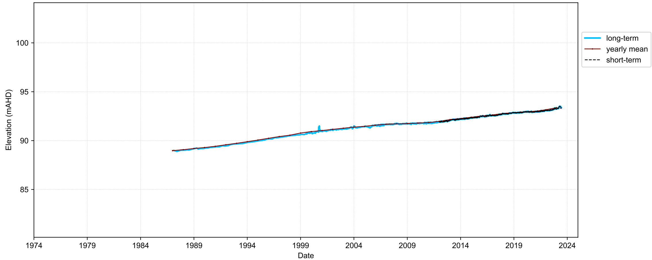
Hydrograph for hydroid: 10007593
