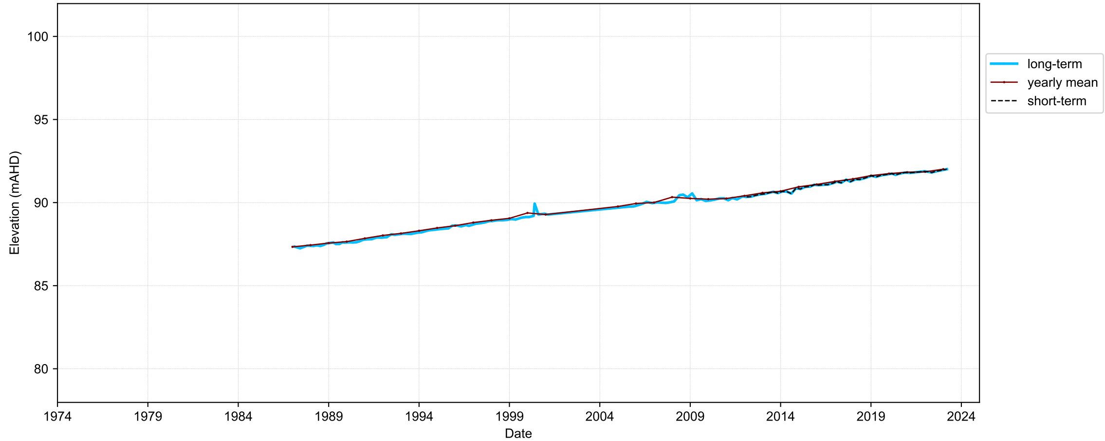
Hydrograph for hydroid: 10046103
