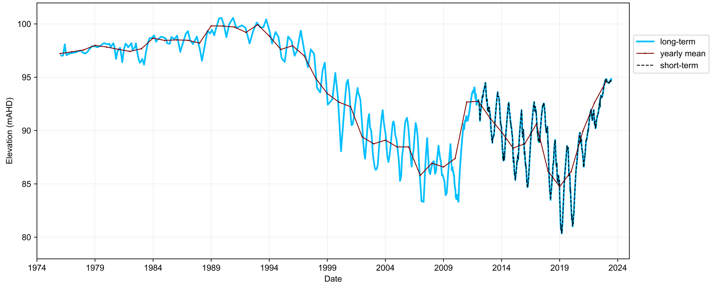
Hydrograph for hydroid: 10101169
