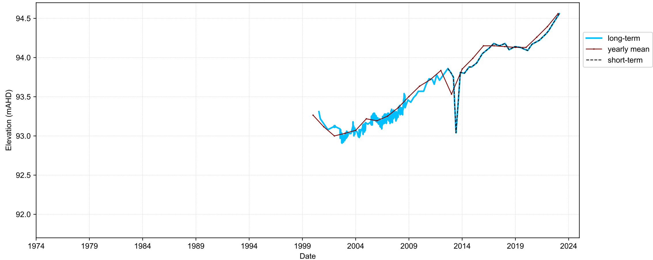
Hydrograph for hydroid: 10007851
