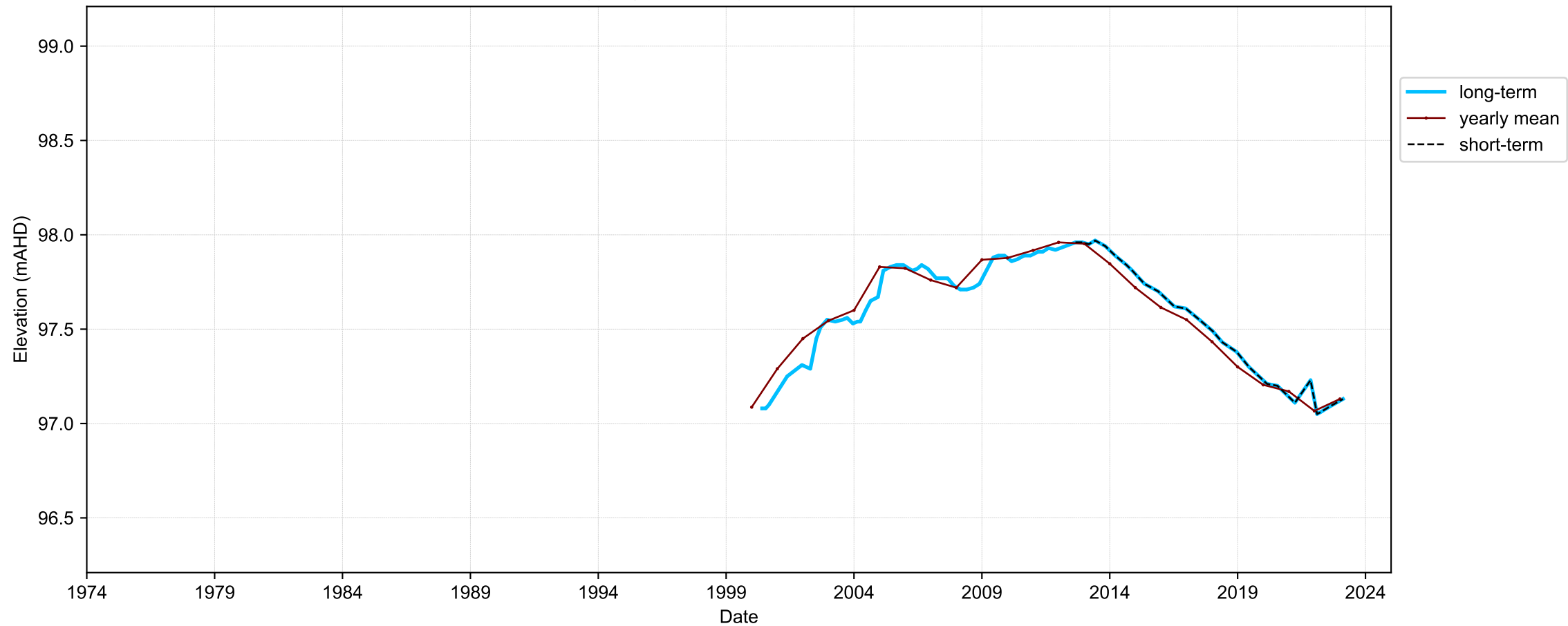
Hydrograph for hydroid: 10006076
