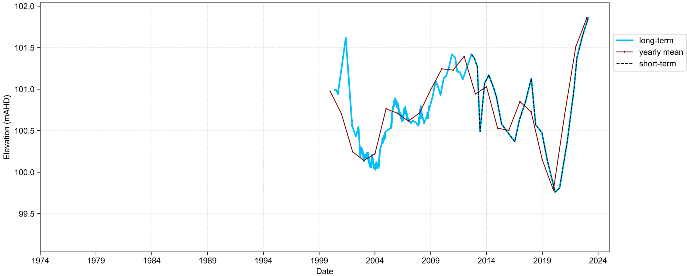
Hydrograph for hydroid: 10008425
