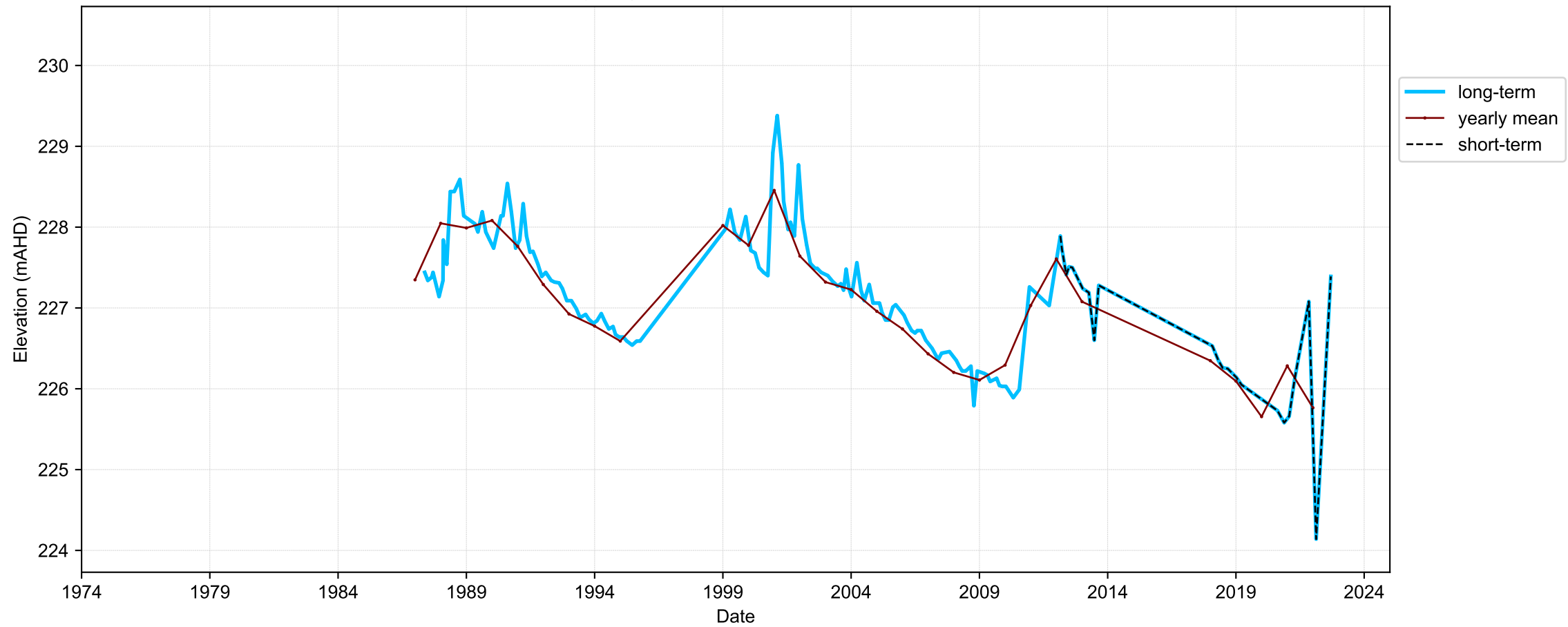
Hydrograph for hydroid: 10103983
