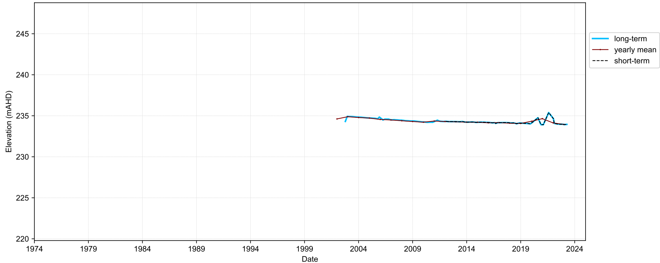
Hydrograph for hydroid: 40131608
