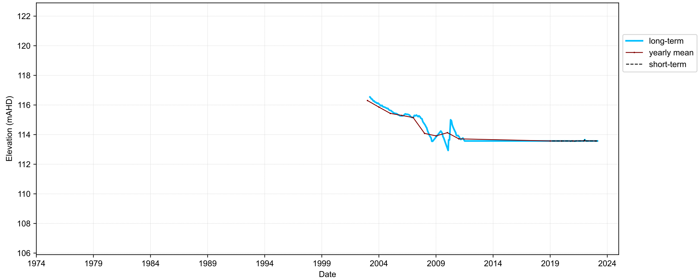
Hydrograph for hydroid: 10062879
