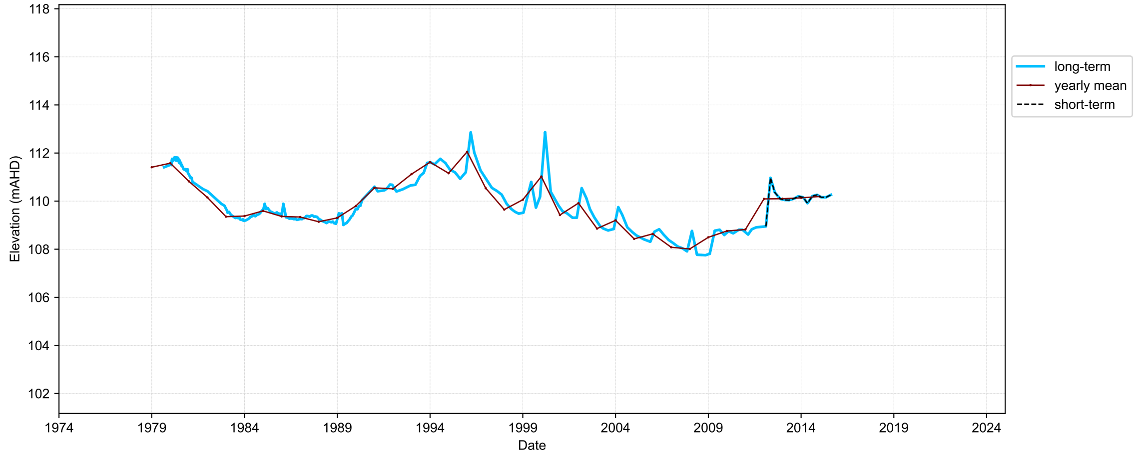
Hydrograph for hydroid: 10100284
