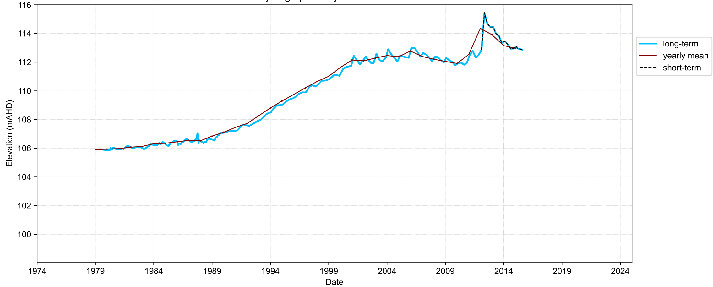
Hydrograph for hydroid: 10128414
