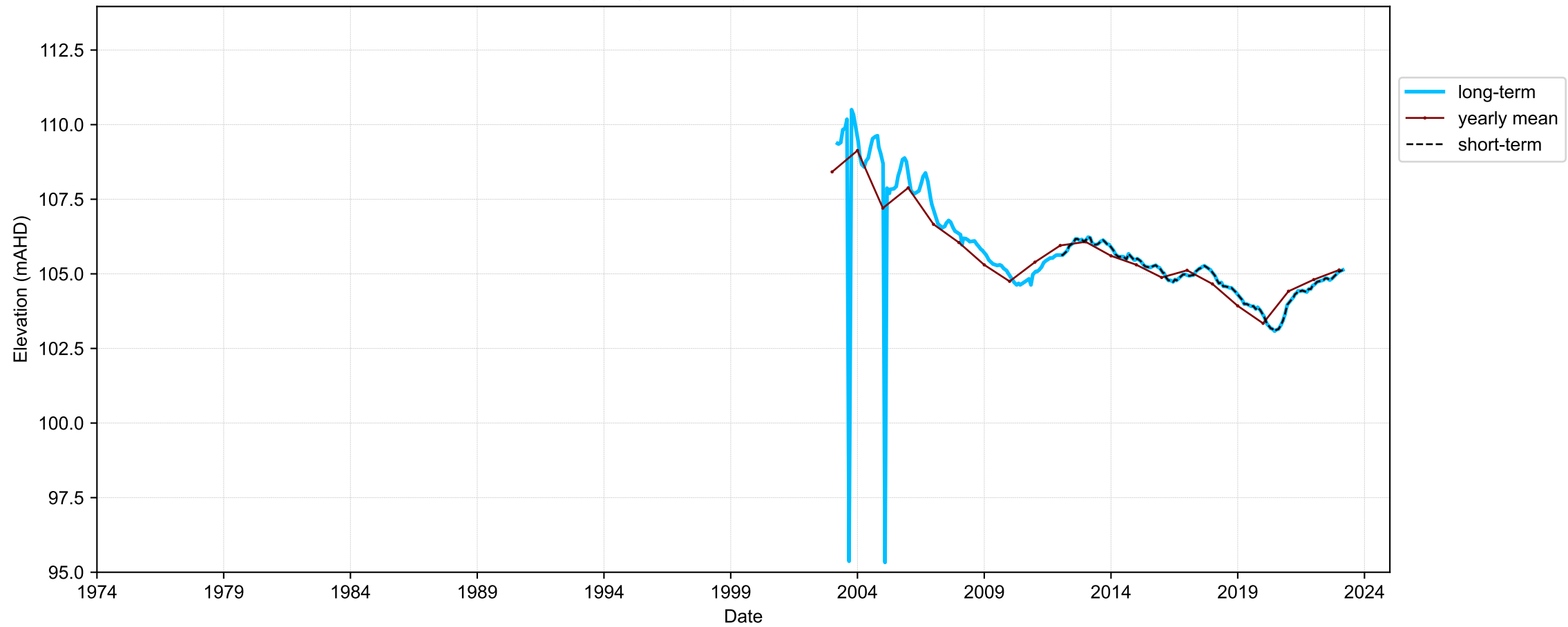
Hydrograph for hydroid: 10139830
