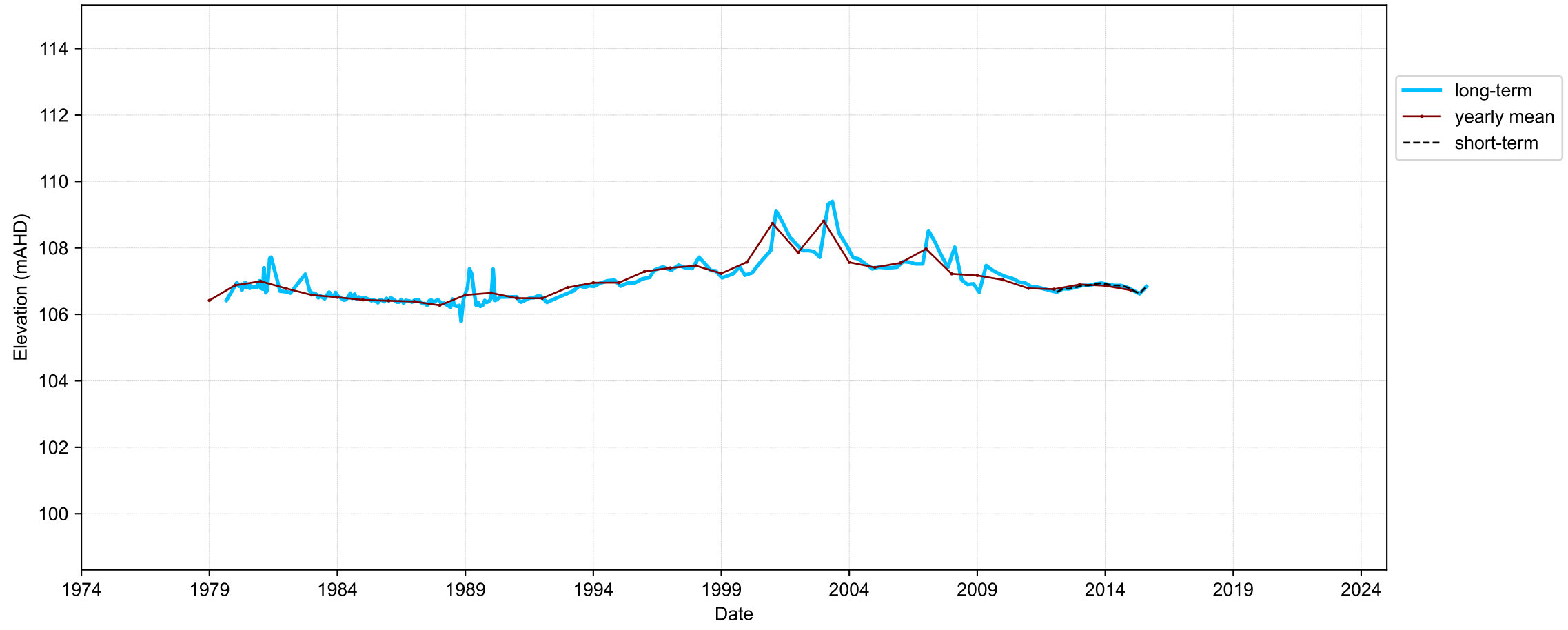
Hydrograph for hydroid: 10108399
