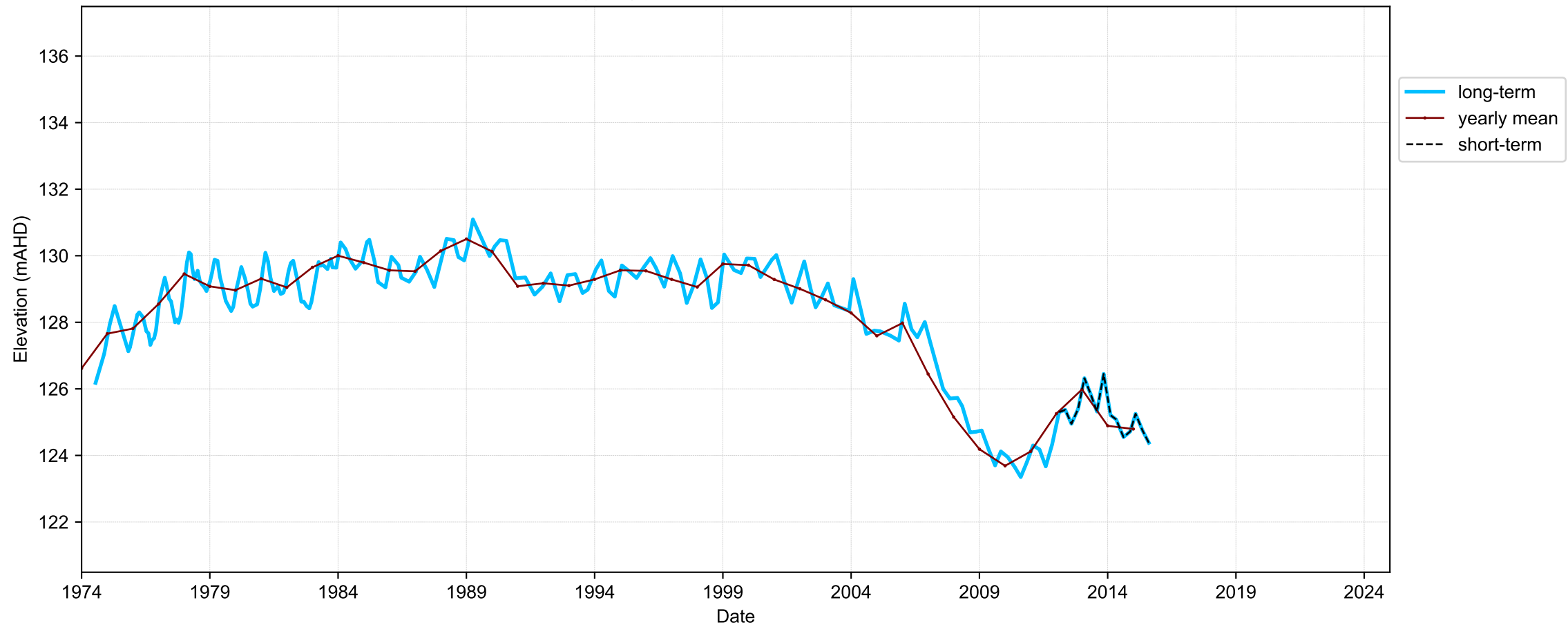
Hydrograph for hydroid: 10103166
