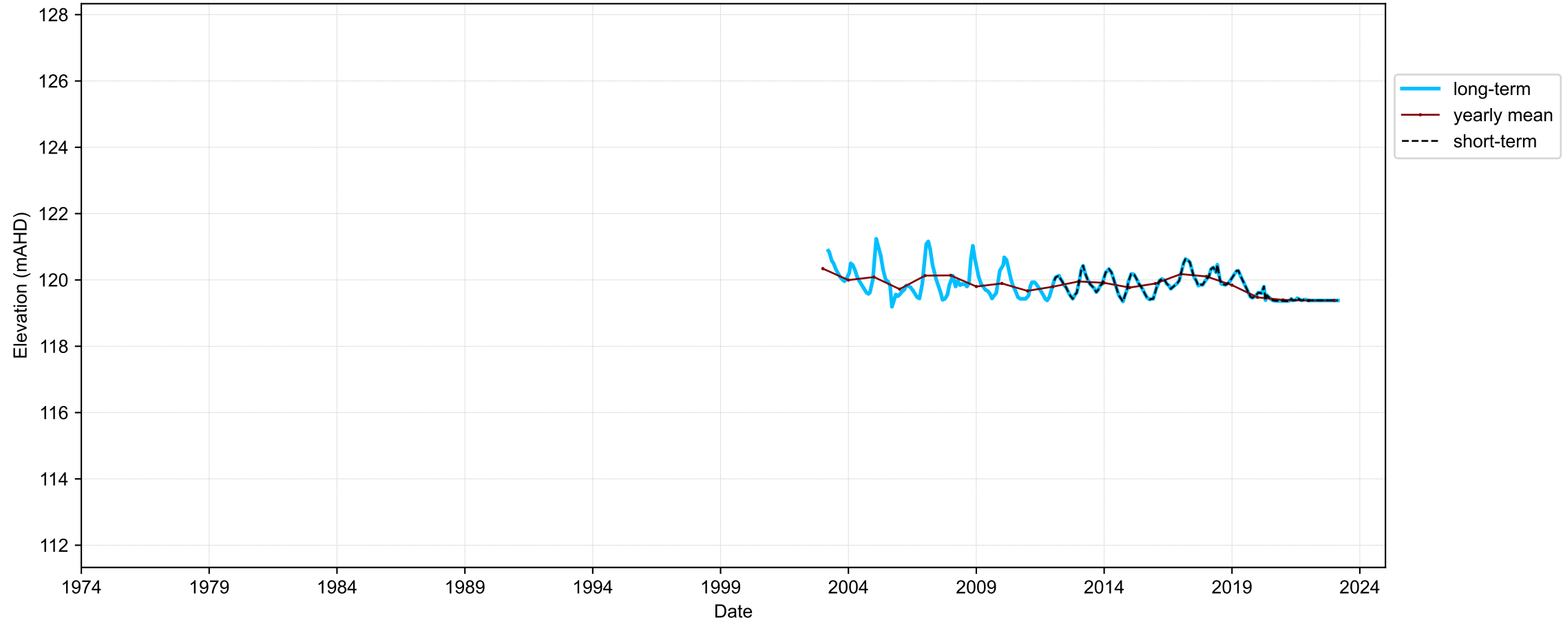
Hydrograph for hydroid: 10068076
