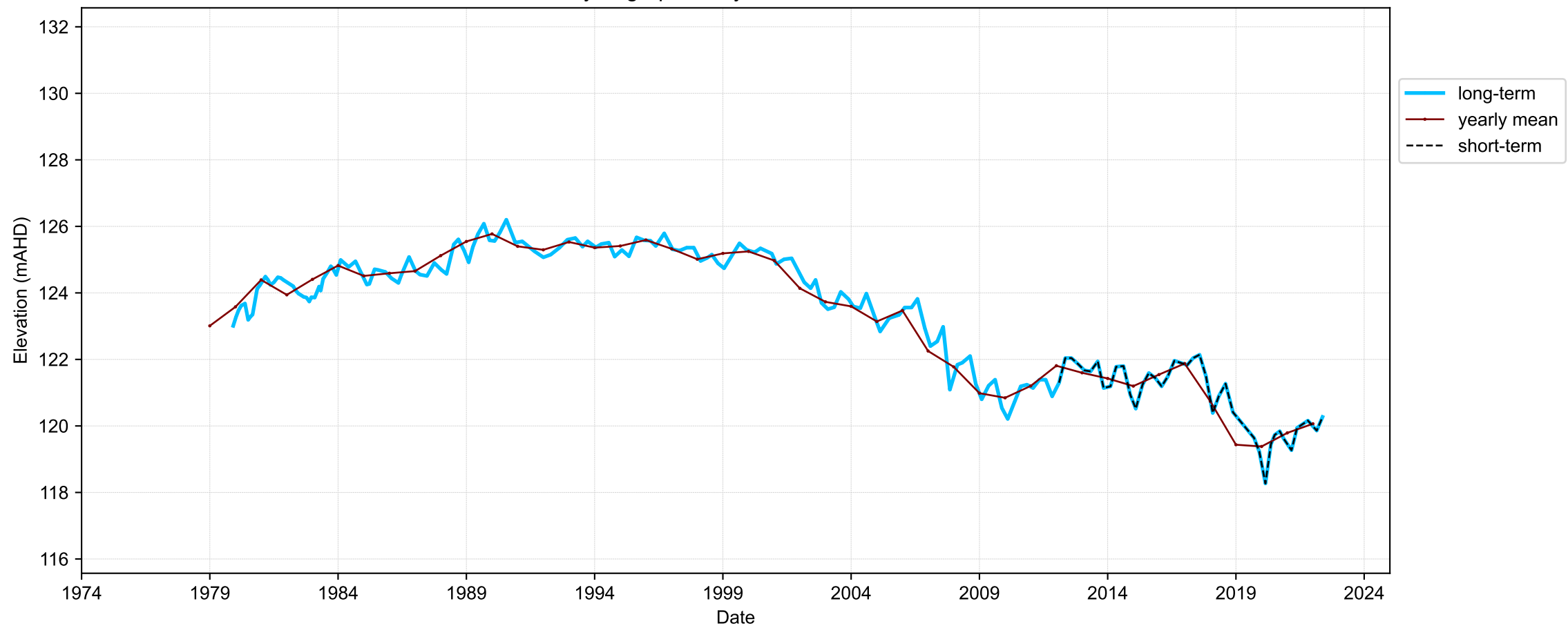
Hydrograph for hydroid: 10138442
