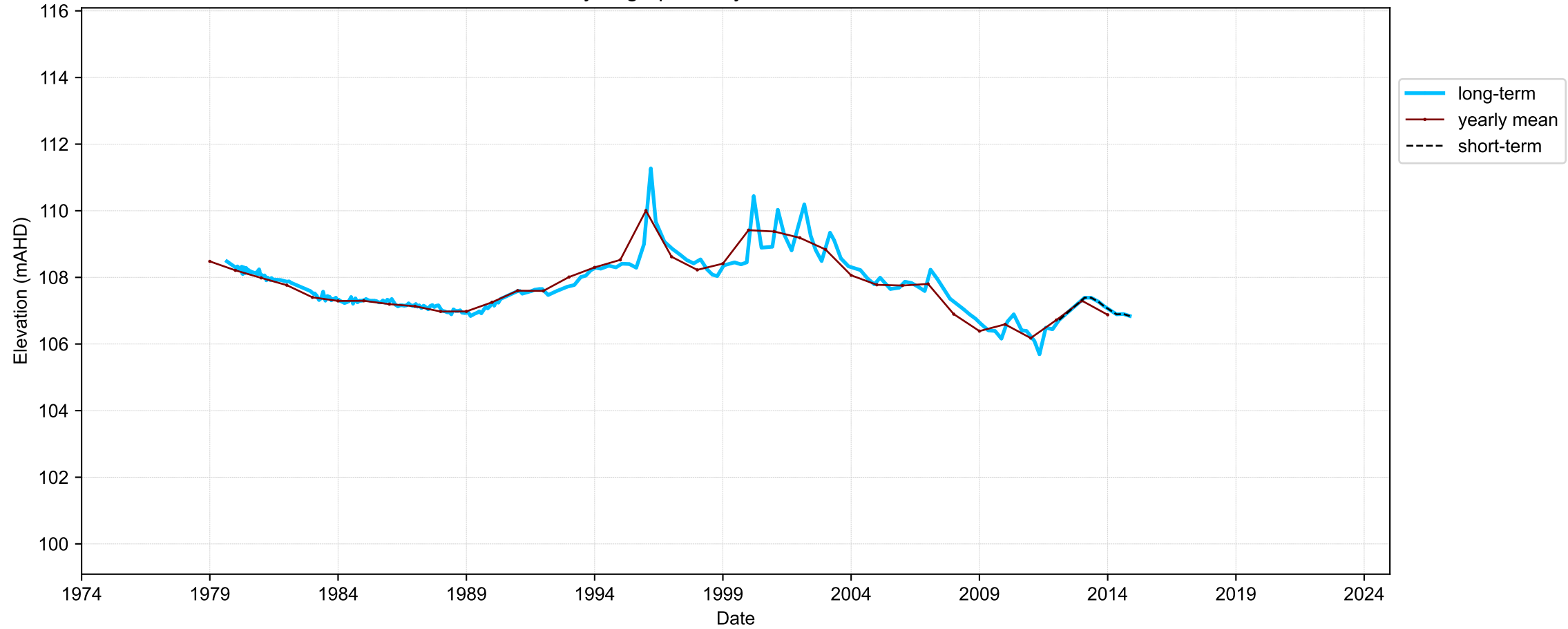
Hydrograph for hydroid: 10104128
