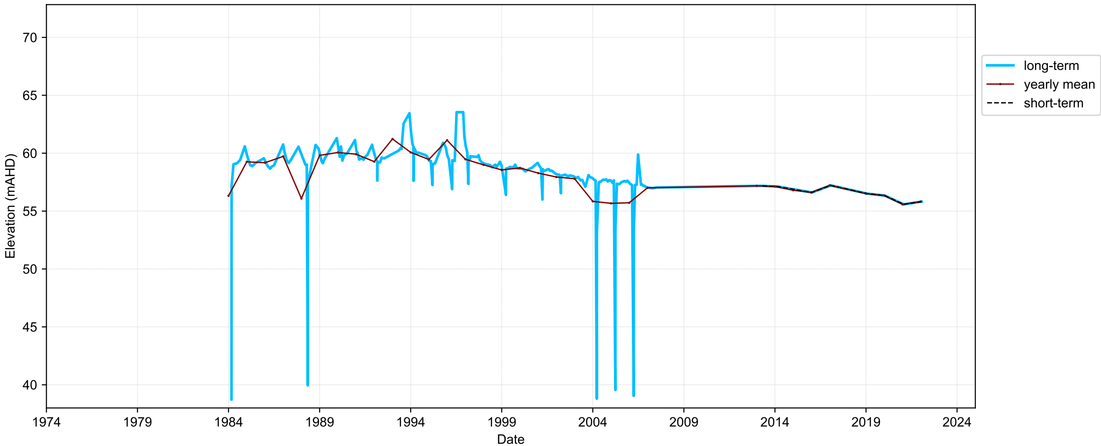
Hydrograph for hydroid: 20176745
