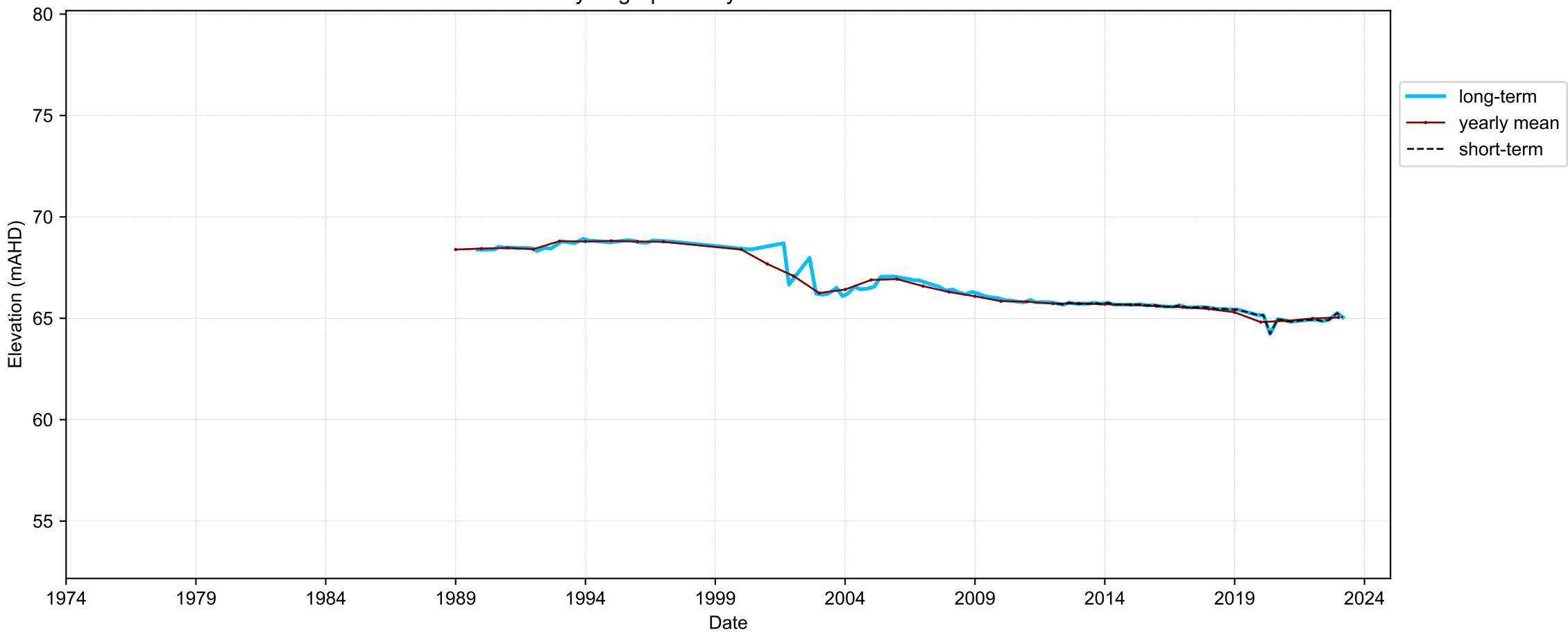
Hydrograph for hydroid: 10020578
