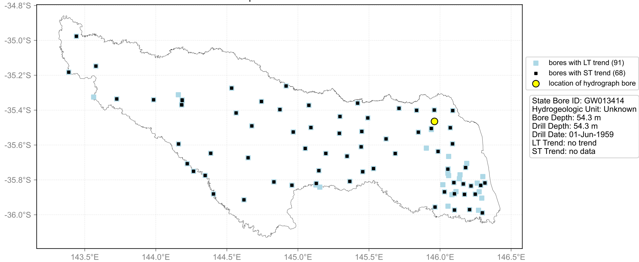
Hydrograph for hydroid: 10109227
