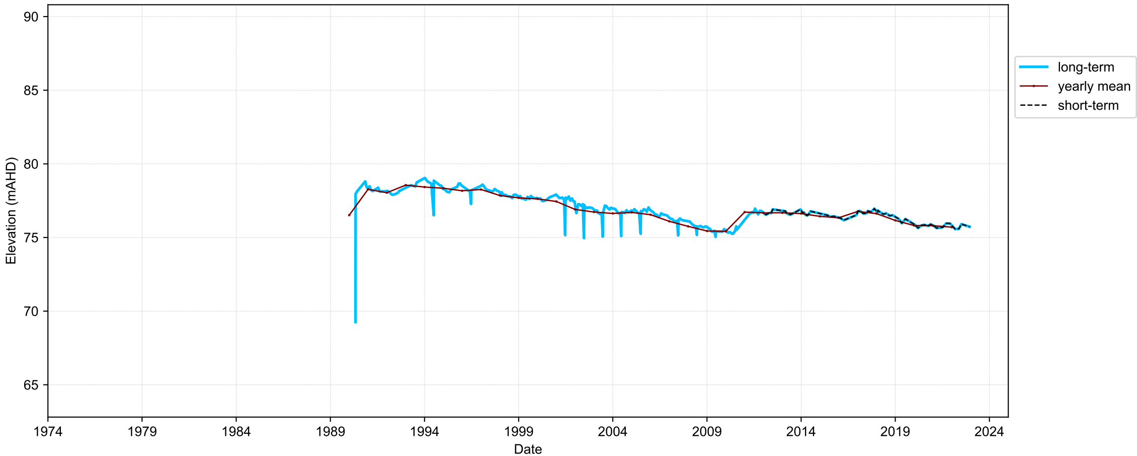
Hydrograph for hydroid: 20176617
