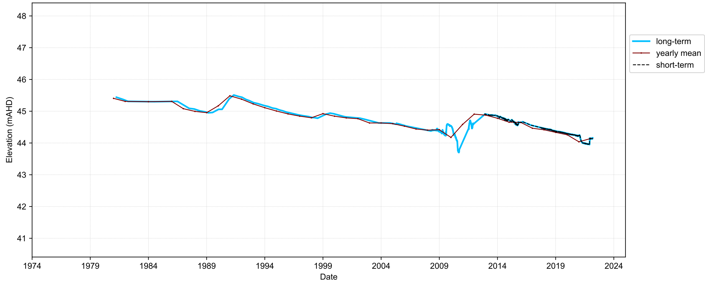
Hydrograph for hydroid: 10120342
