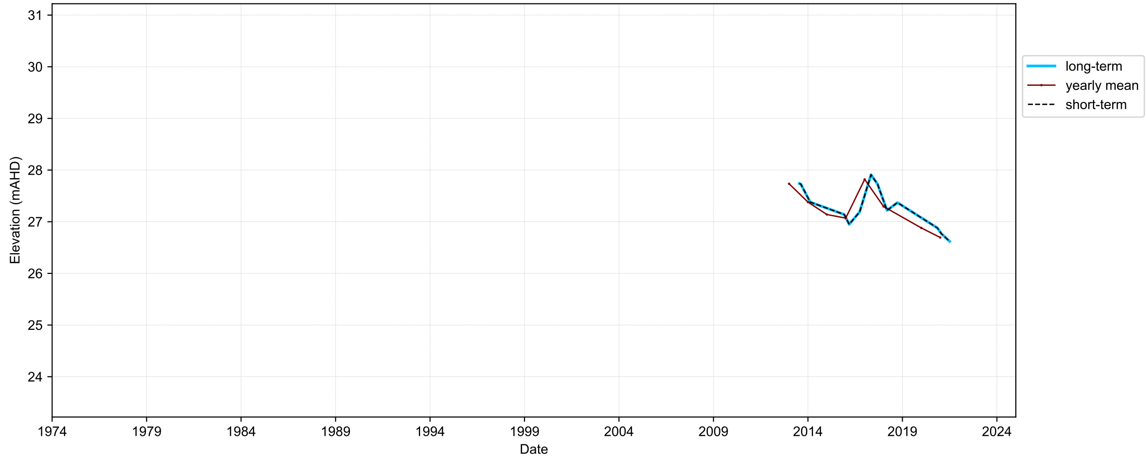
Hydrograph for hydroid: 10044310
