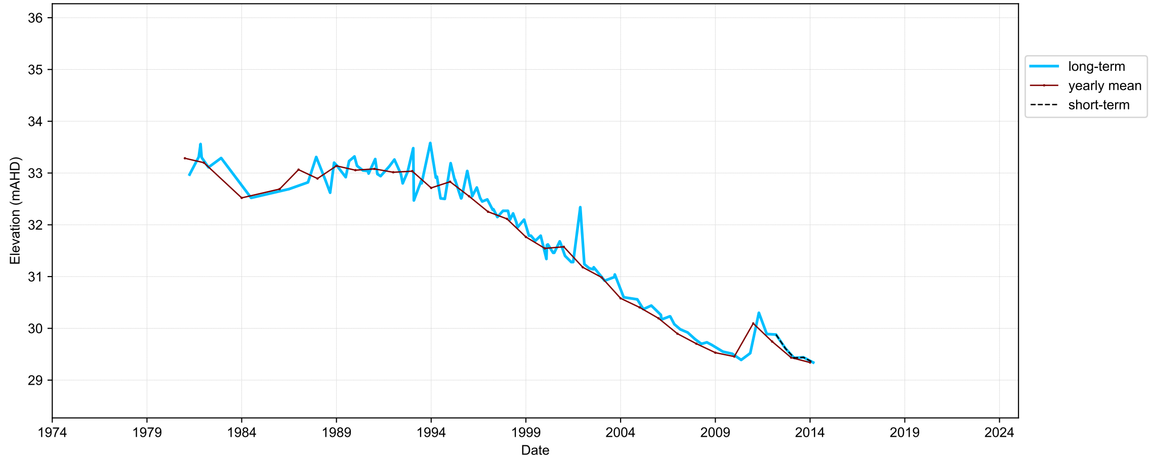
Hydrograph for hydroid: 10067807
