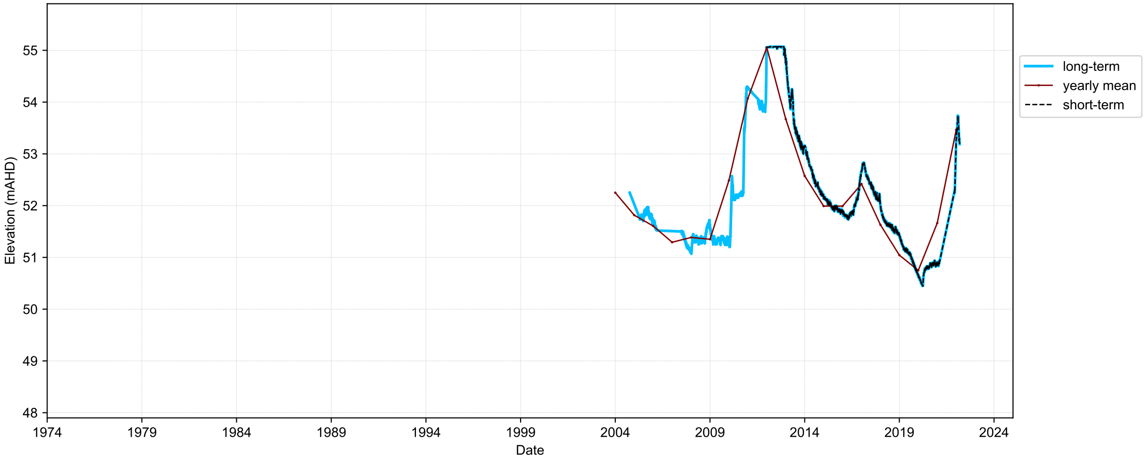
Hydrograph for hydroid: 10068551
