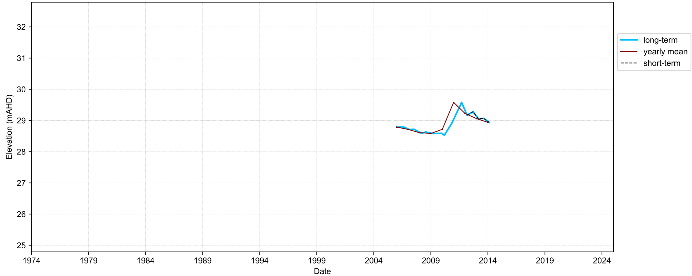
Hydrograph for hydroid: 10127009
