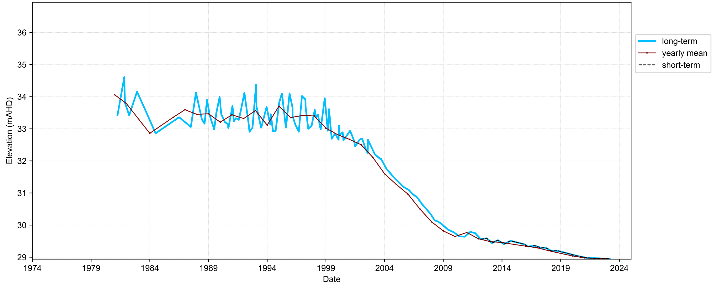
Hydrograph for hydroid: 10104279
