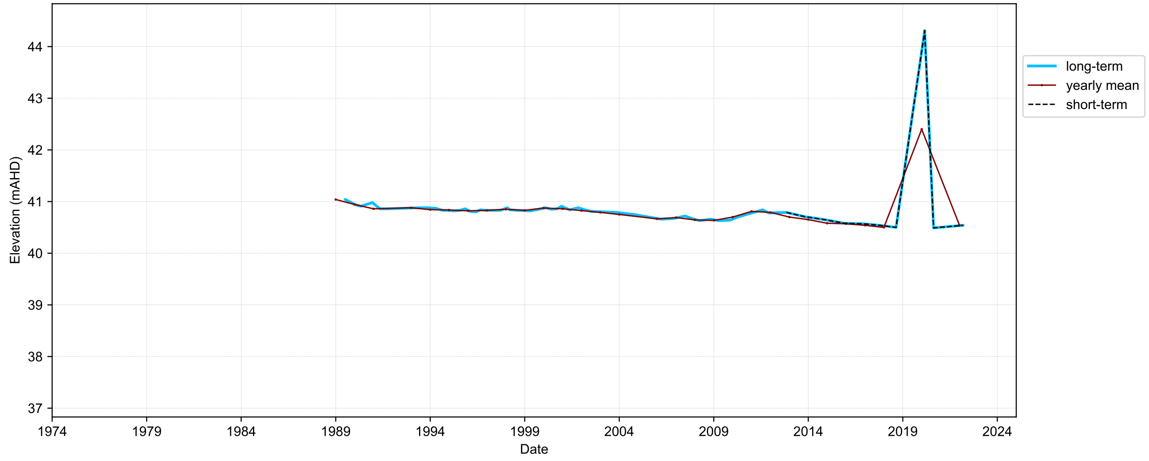
Hydrograph for hydroid: 10024911
