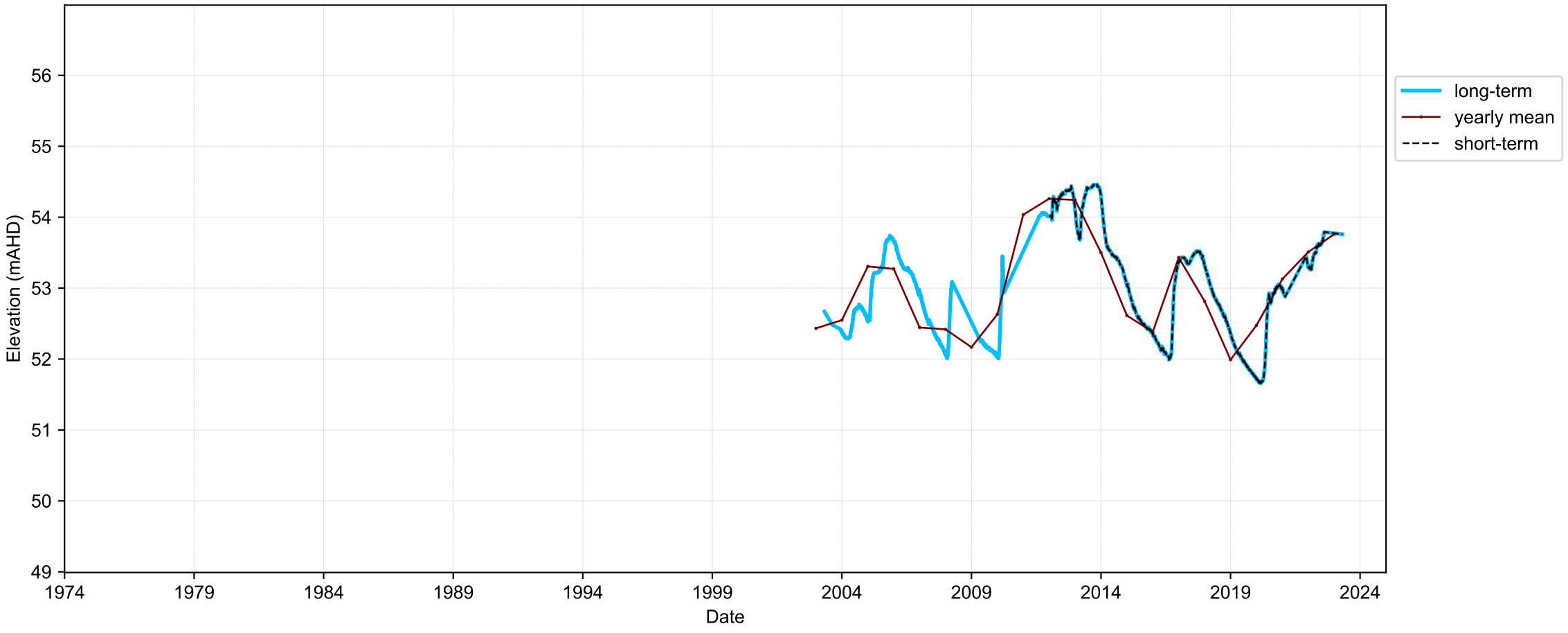
Hydrograph for hydroid: 10075751
