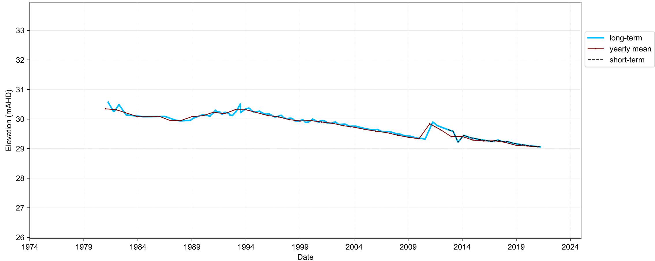
Hydrograph for hydroid: 10101965
