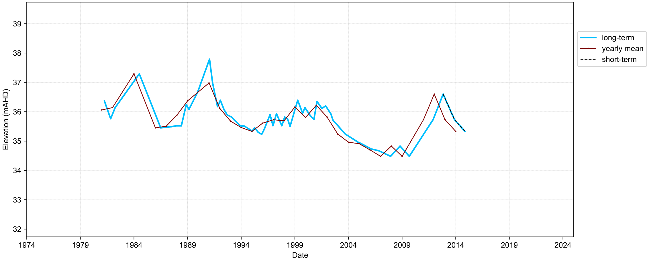
Hydrograph for hydroid: 10102370
