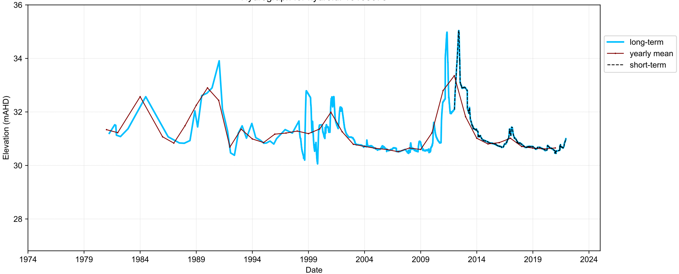
Hydrograph for hydroid: 10105078
