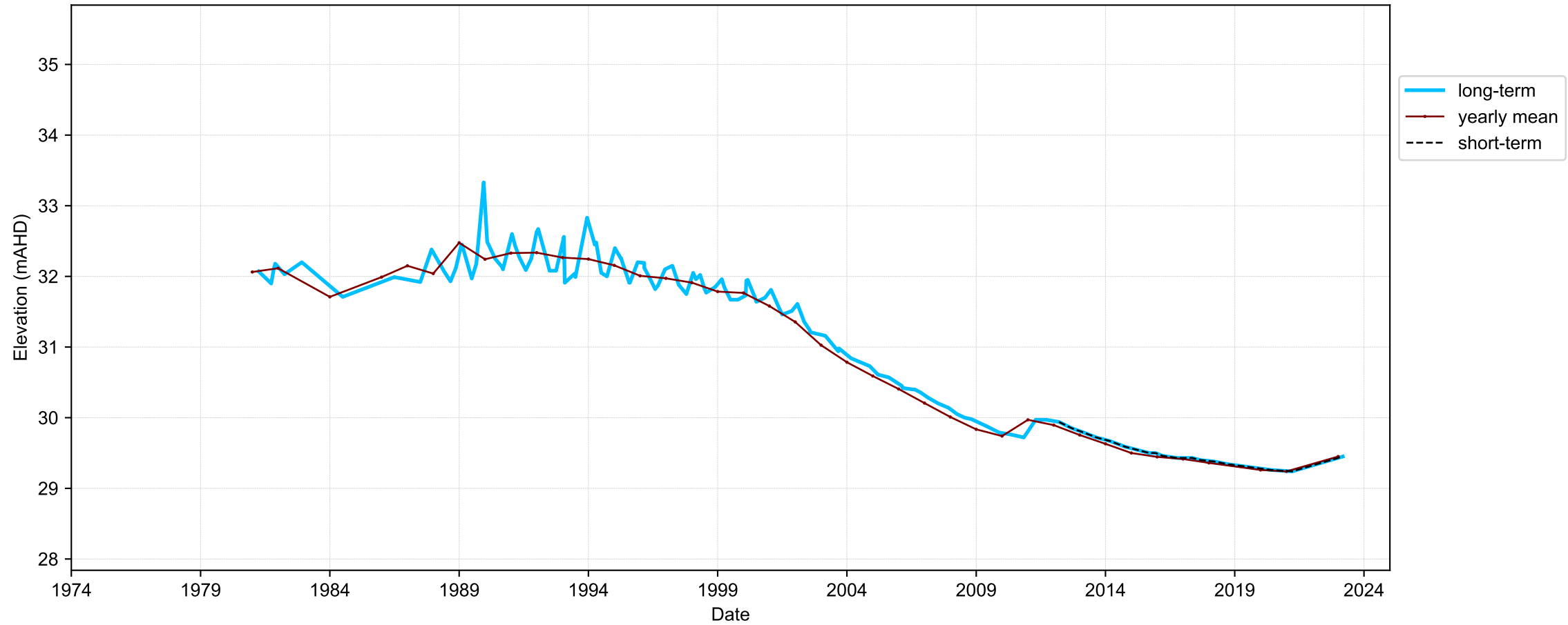
Hydrograph for hydroid: 10077986
