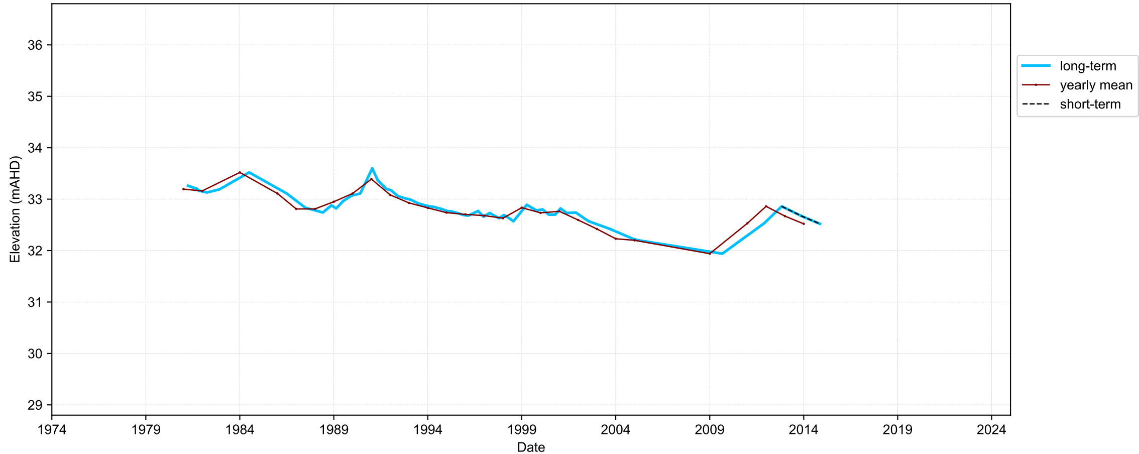
Hydrograph for hydroid: 10092604
