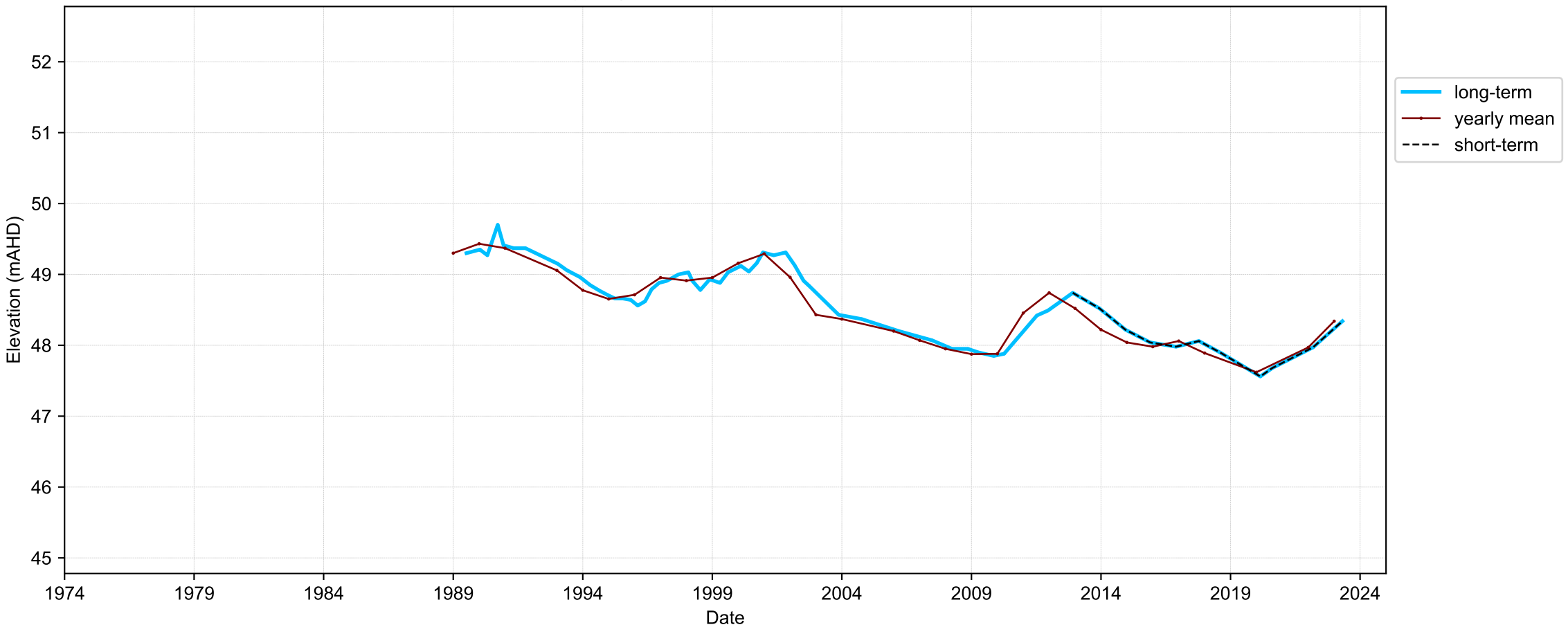
Hydrograph for hydroid: 10097568
