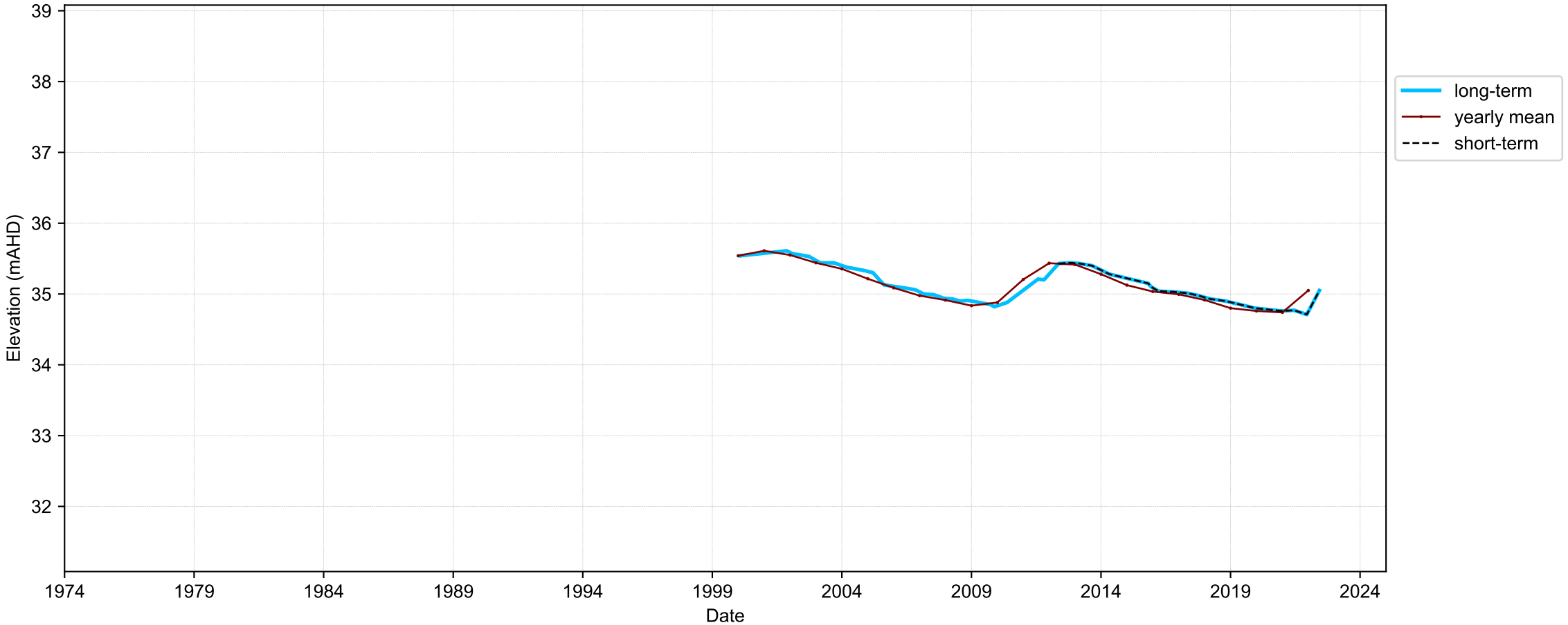
Hydrograph for hydroid: 10055721
