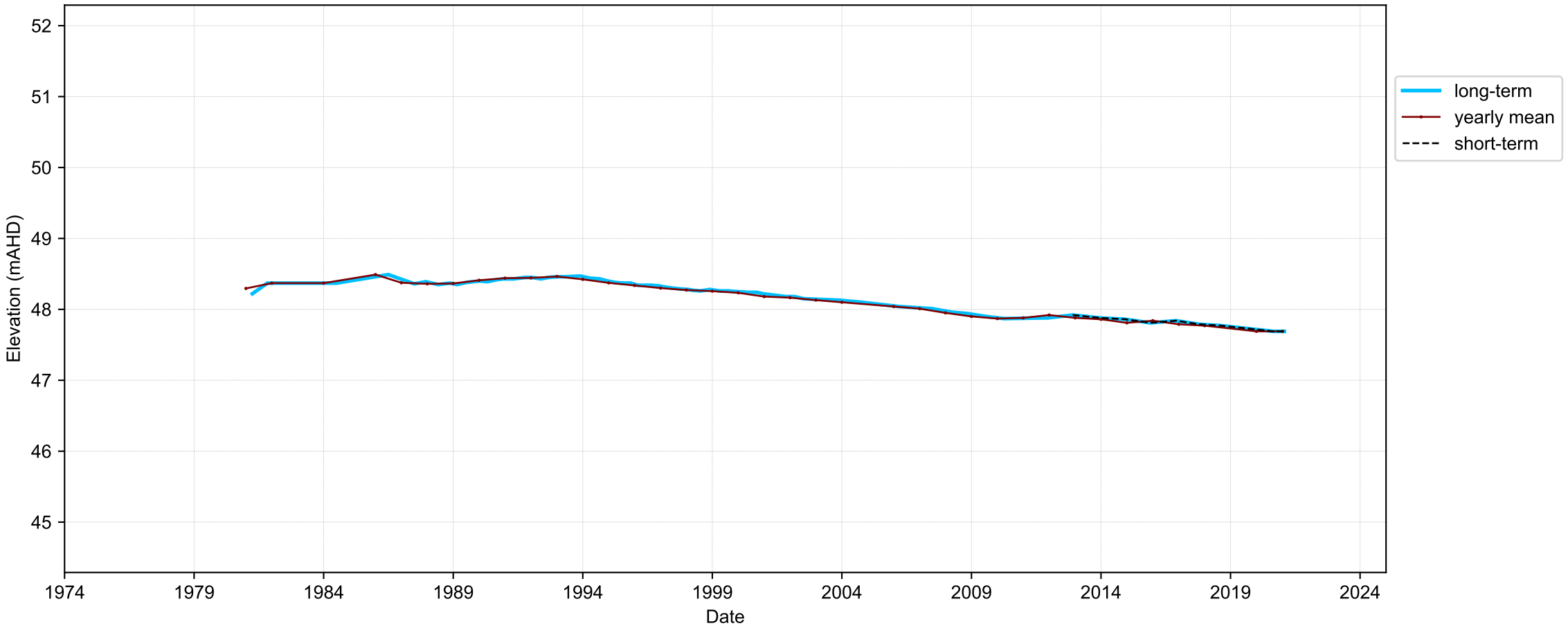
Hydrograph for hydroid: 10127517
