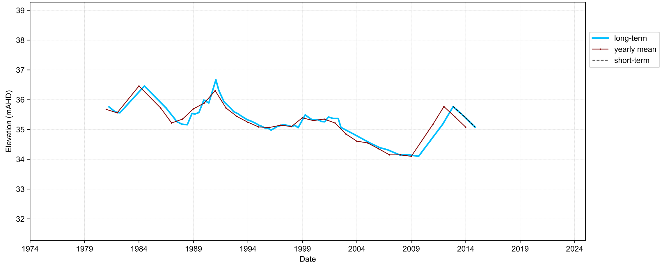
Hydrograph for hydroid: 10110269
