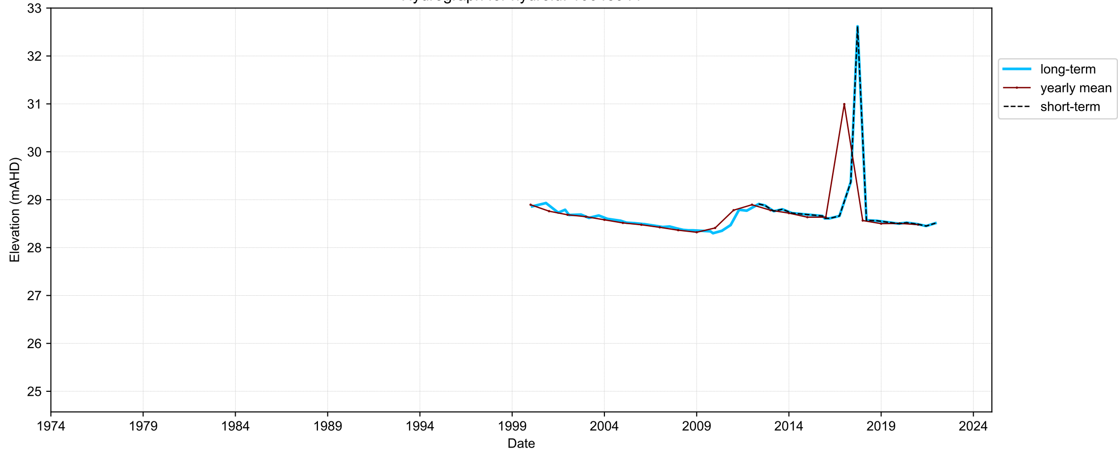
Hydrograph for hydroid: 10048944
