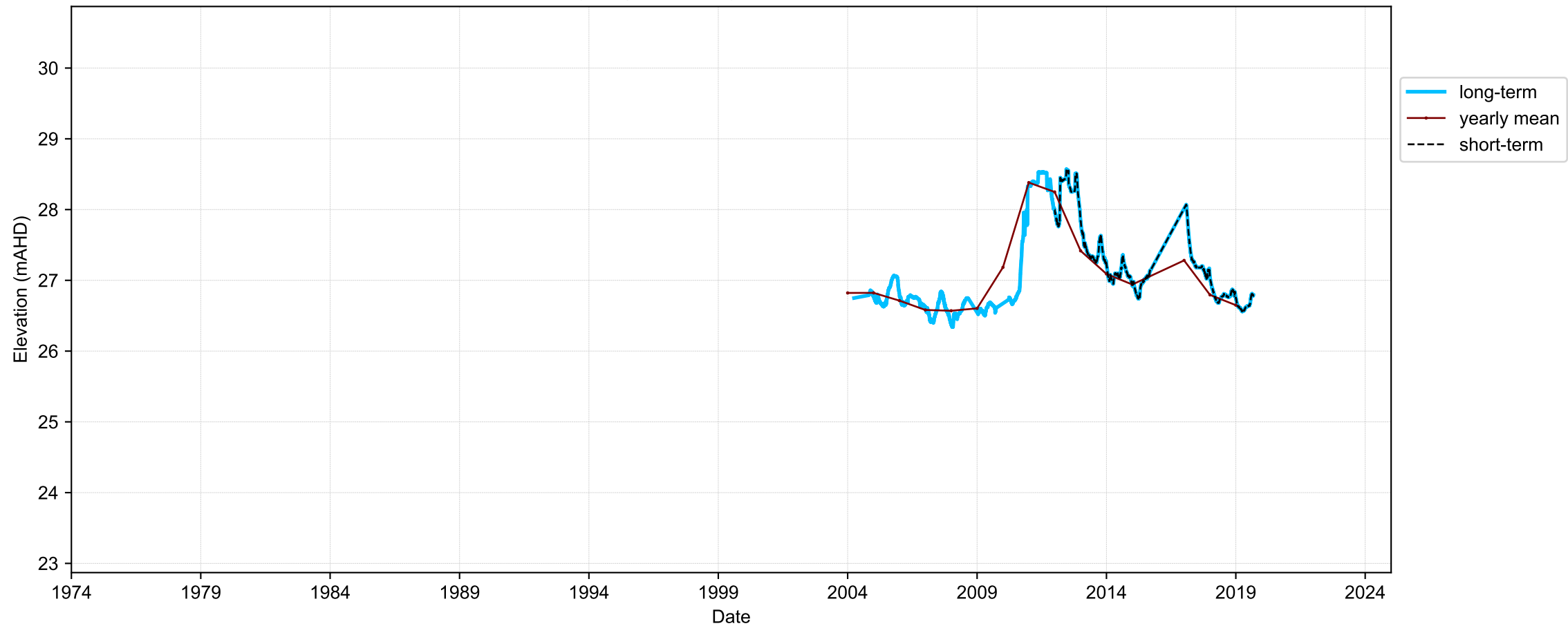
Hydrograph for hydroid: 10091618
