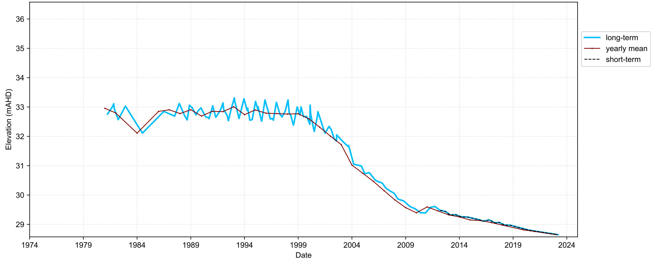
Hydrograph for hydroid: 10077387
