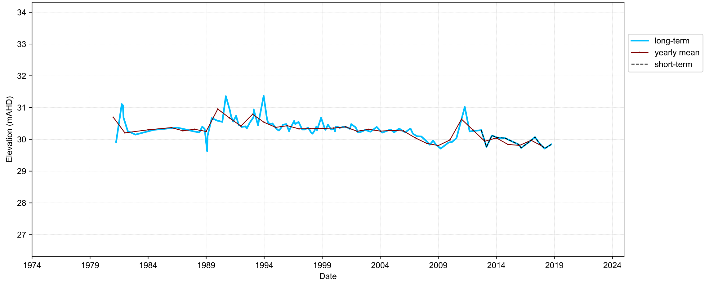
Hydrograph for hydroid: 10108578
