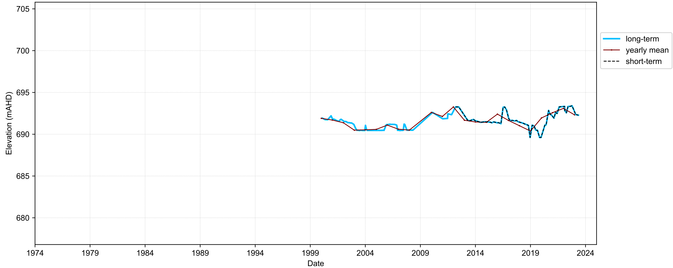
Hydrograph for hydroid: 10137662
