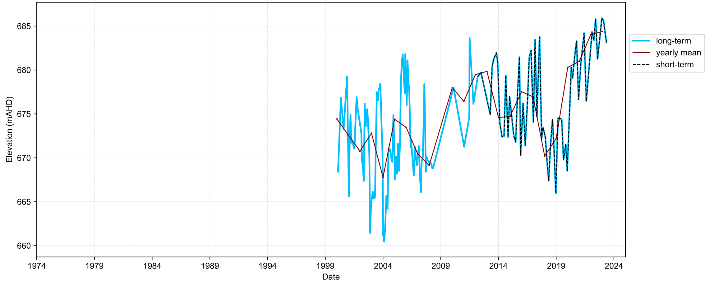
Hydrograph for hydroid: 10131901
