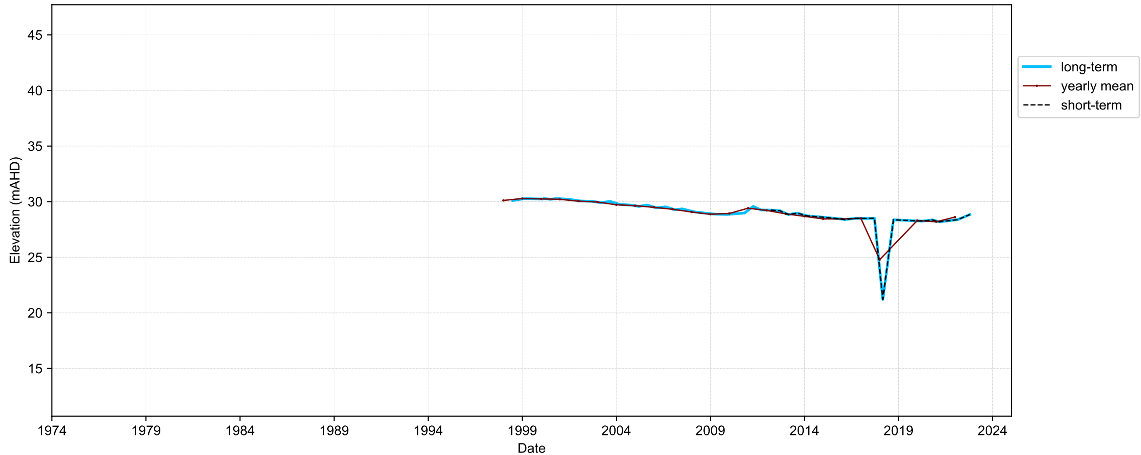
Hydrograph for hydroid: 10125807
