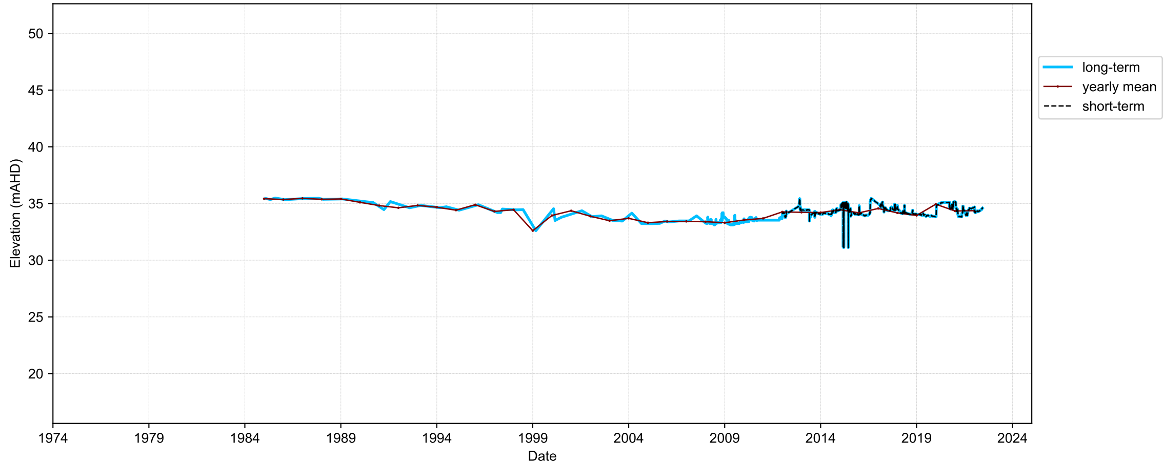
Hydrograph for hydroid: 10133618
