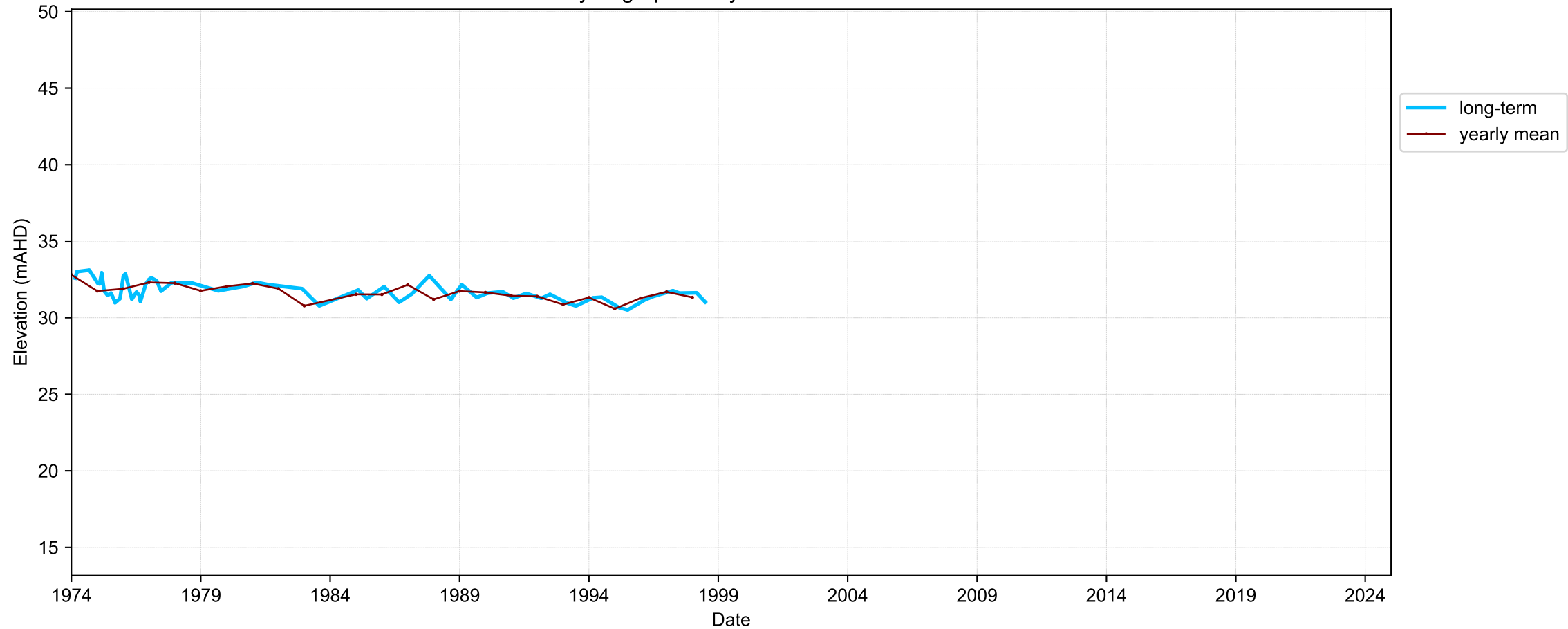
Hydrograph for hydroid: 10027871
