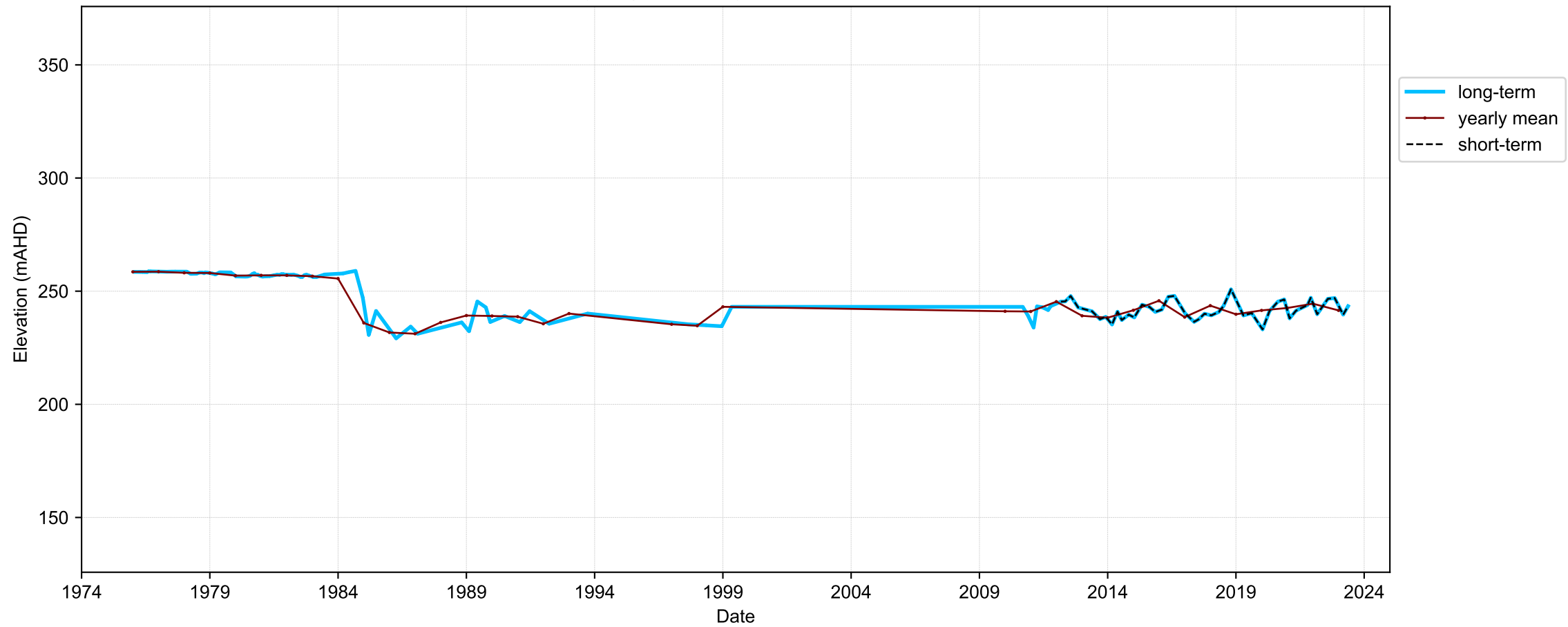
Hydrograph for hydroid: 10111408
