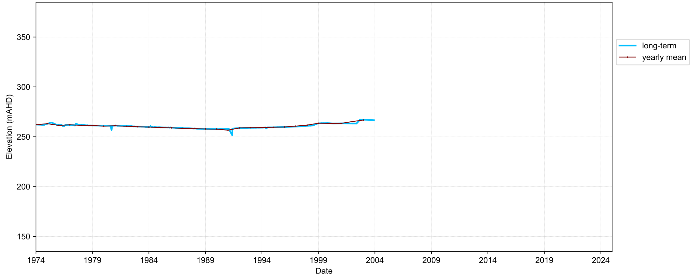
Hydrograph for hydroid: 10100315
