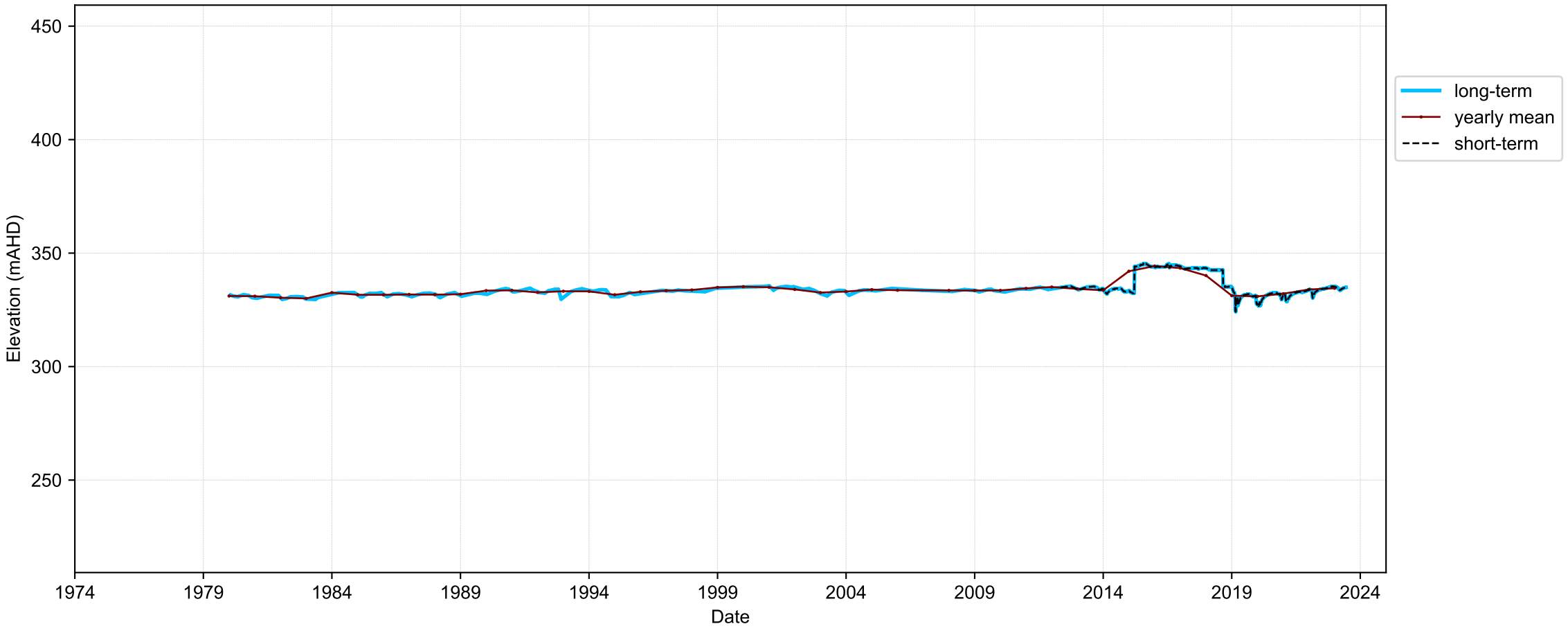
Hydrograph for hydroid: 10009935
