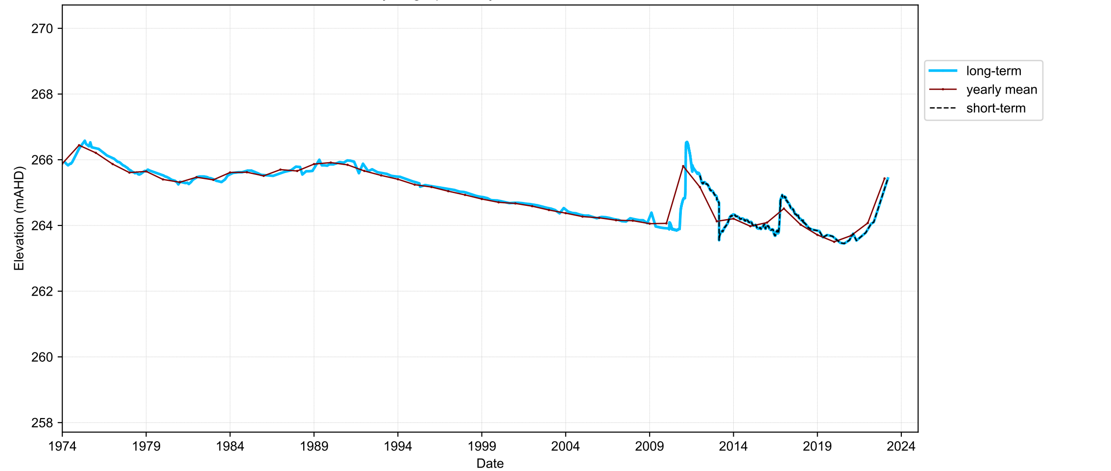
Hydrograph for hydroid: 10017149
