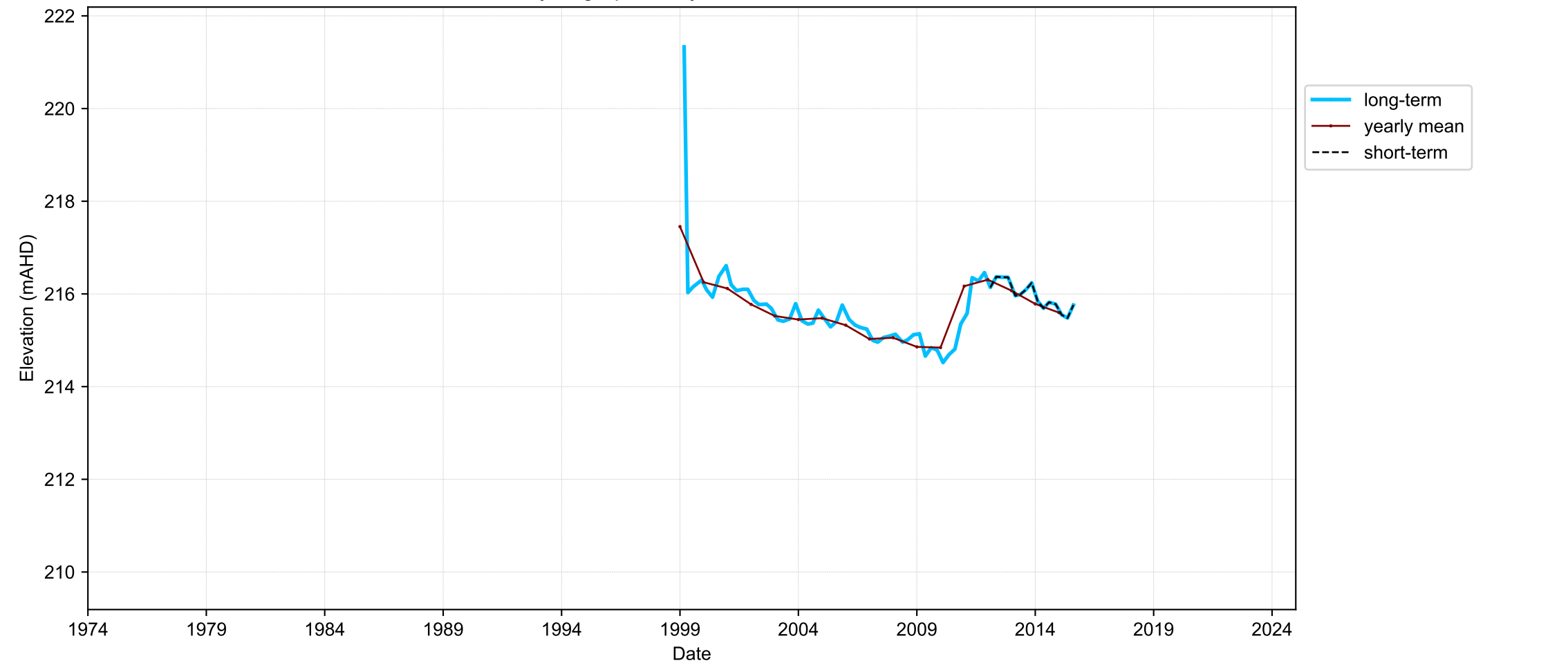
Hydrograph for hydroid: 10091216
