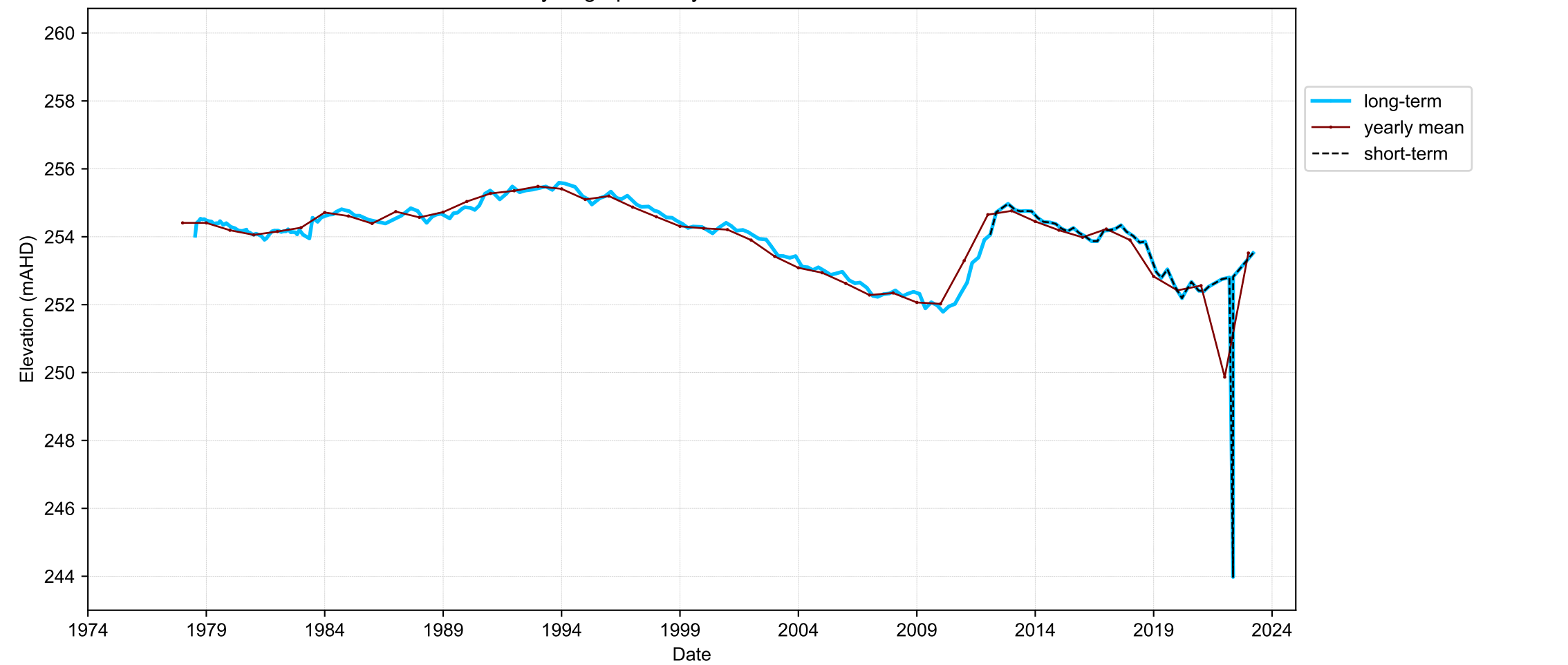
Hydrograph for hydroid: 10111672
