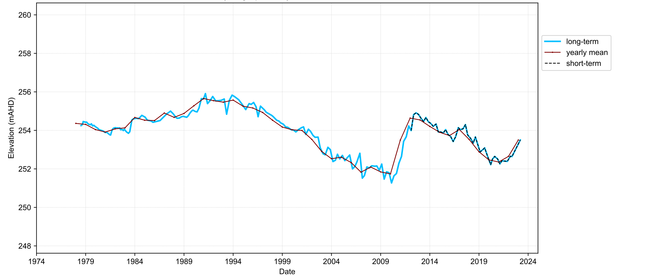
Hydrograph for hydroid: 10136559
