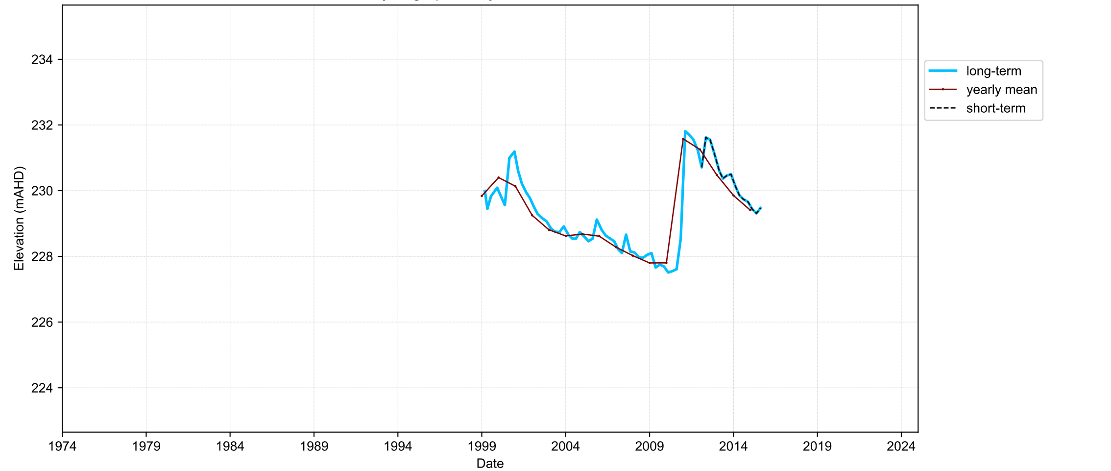
Hydrograph for hydroid: 10088680
