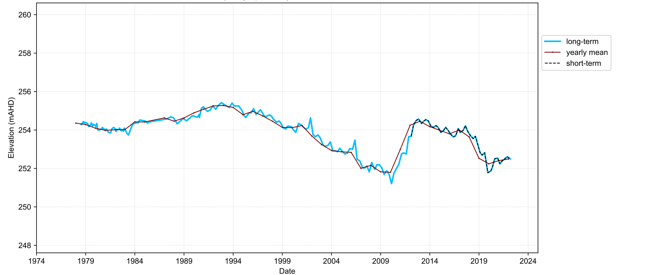
Hydrograph for hydroid: 10104598
