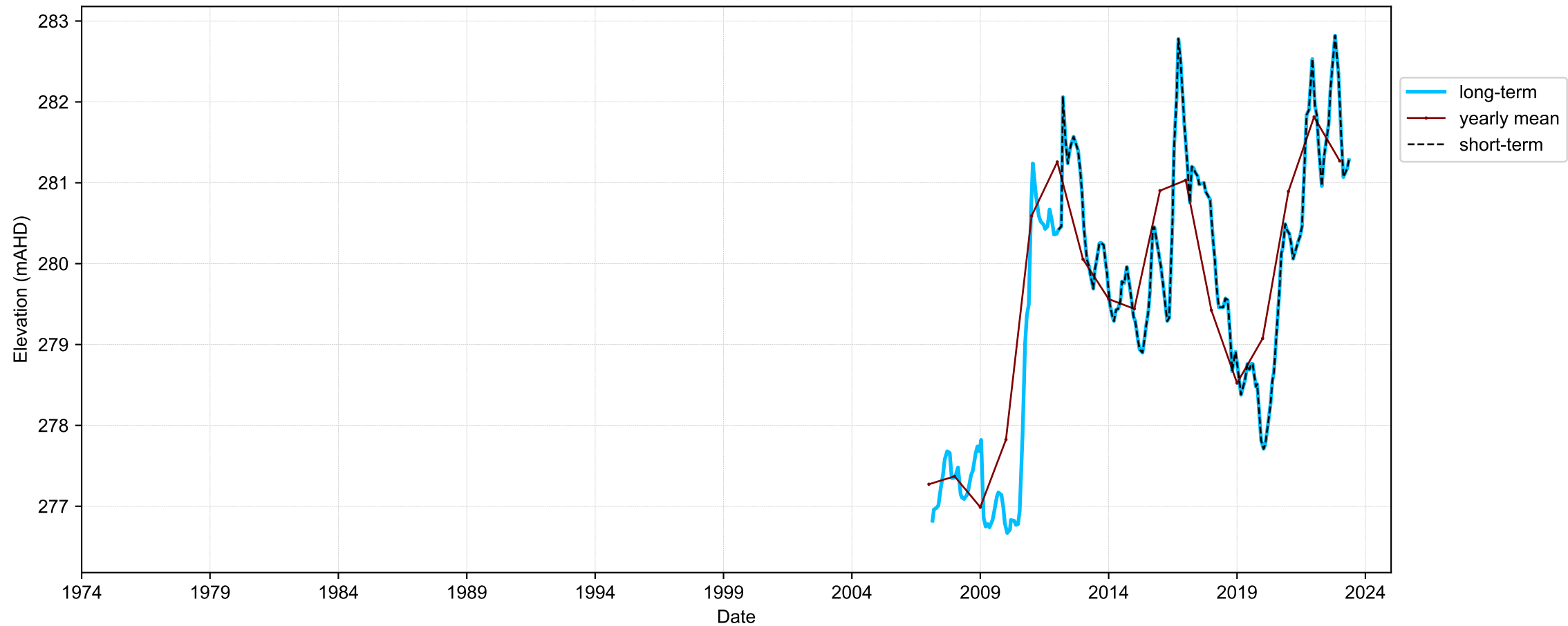
Hydrograph for hydroid: 10139417
