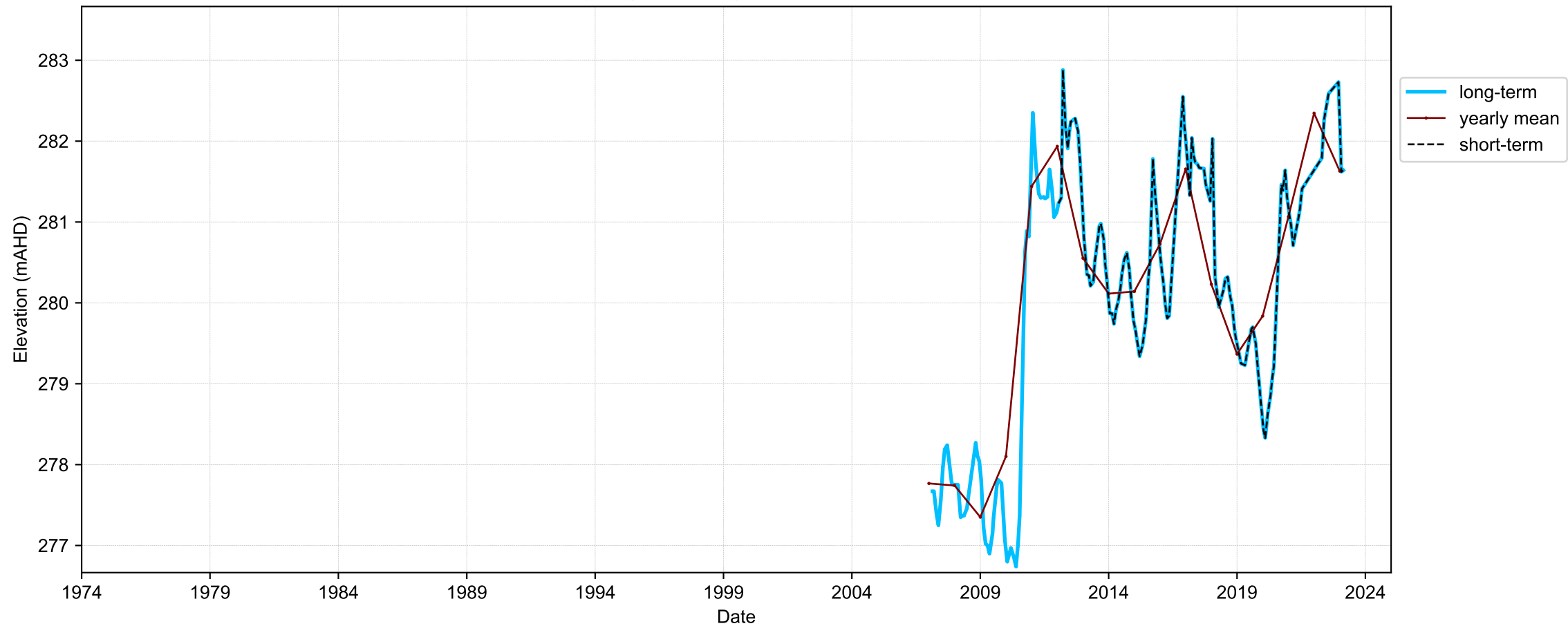
Hydrograph for hydroid: 10138783
